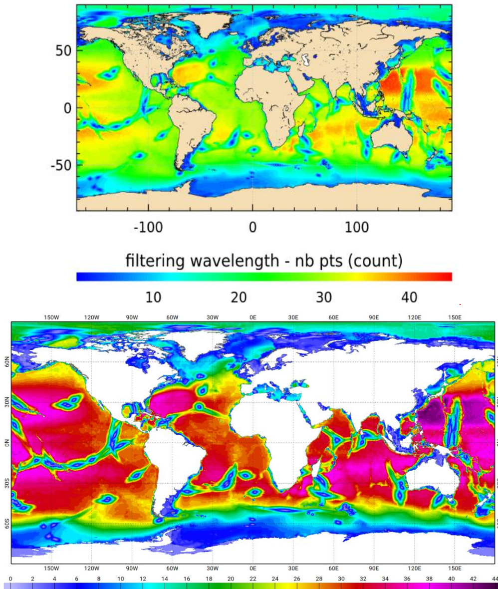
Figure 5 : along-track filtering wavelength used to remove internal tides surface signatures ( expressed in number of 1Hz along-track points, to be multiplied by a factor six to retrieve the equivalent wavelength in kilometer )
