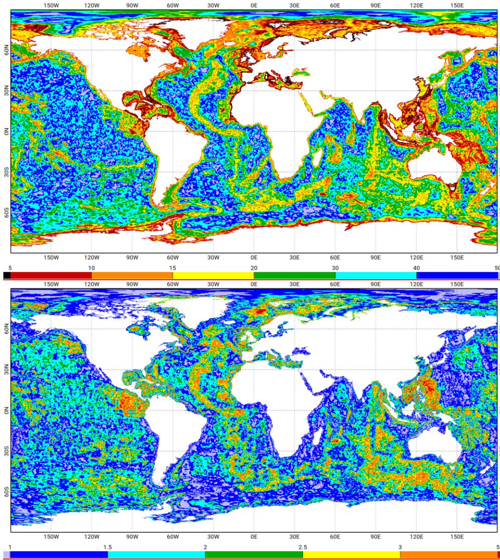
Figure 1: Element-wise resolution (in km) of the FES2014 unstructured grids (upper panel) and the FES2014/ resolution divided by FES2004 resolution ratio (lower panel). Resolution increase has been mostly focused on ocean ridges, shelves and shores (wherever reasonably accurate bathymetry was made available to the project). The numerical resolution of the frequency domain solutions is half the element-wise resolution due to second order basis functions (Lagrange P2).
