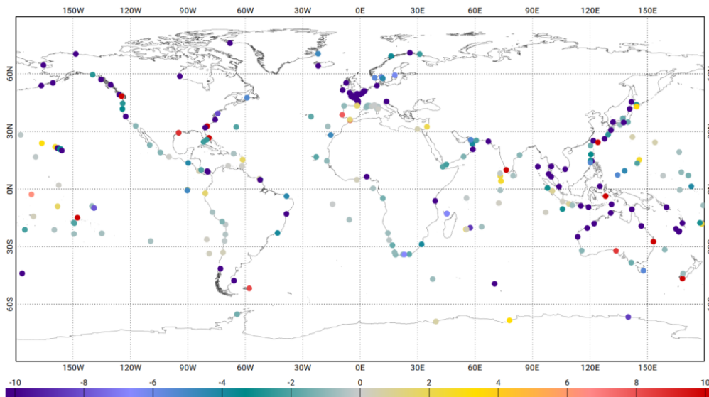
Figure 13 : Variance reduction differences (cm 2 ) at tidal gauges sites from GLOSS network, when using the new FES2014b tidal model and without atlas versus the GOT4v10 solution in cm 2 atlas . Analysis computed over the 2007 to 2011 time period. Blue colours indicate a higher variance reduction when using FES2014b tidal correction. Tidal corrections made for both models with their native constituents spectrum (i.e. not restricted to their common constituents).
