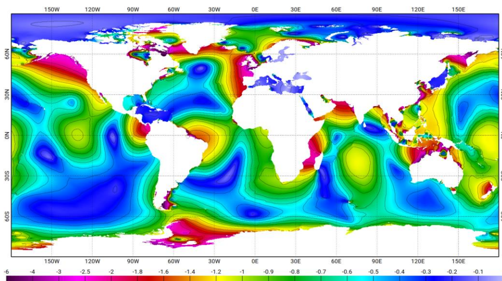
Figure 2324 : Lowest Astronomical Tides (LAT) relative to mean sea level computed from an 18-year FES2014 FES2014b tidal prediction.
