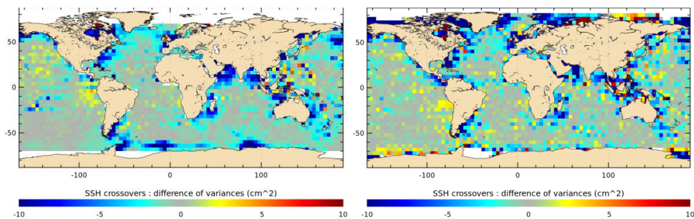
Figure 15 : maps Maps of SSH variance differences at crossovers using either the FES2014b tidal solution atlas or the GOT4v10 solution atlas in the SSH calculation for the Jason-2 mission (on the left, upper panel, J2 cycles 1-281) , and for AltiKa (on the right lower panel, AL cycles 1-21, in cm 2 ) . Blue colours indicate a higher variance reduction when using FES2014b tidal correction. Tidal corrections made for both models with their native constituents spectrum (i.e. not restricted to their common constituents).
