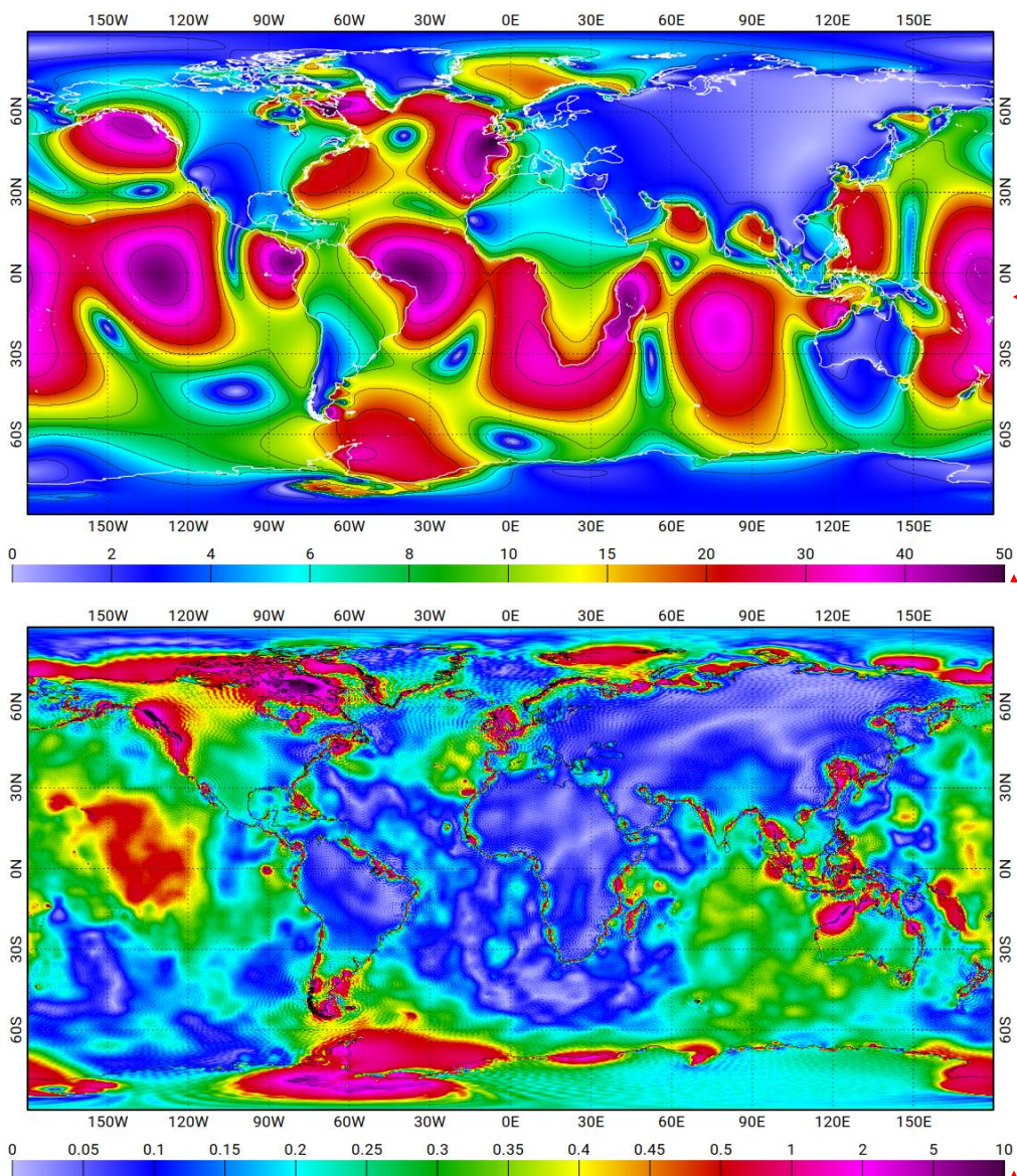
Figure 2122: upper panel, M2 tidal loading, vertical displacement (cm); lower panel, M2 tidal loading vector difference between FES2014 and GOT4.10 (cm). Wave-like patterns visible in some regions are likely due to differences between Green's functions based computation of LSA (as in FES2014 atlas) and spherical harmonics based computation (GOT).
