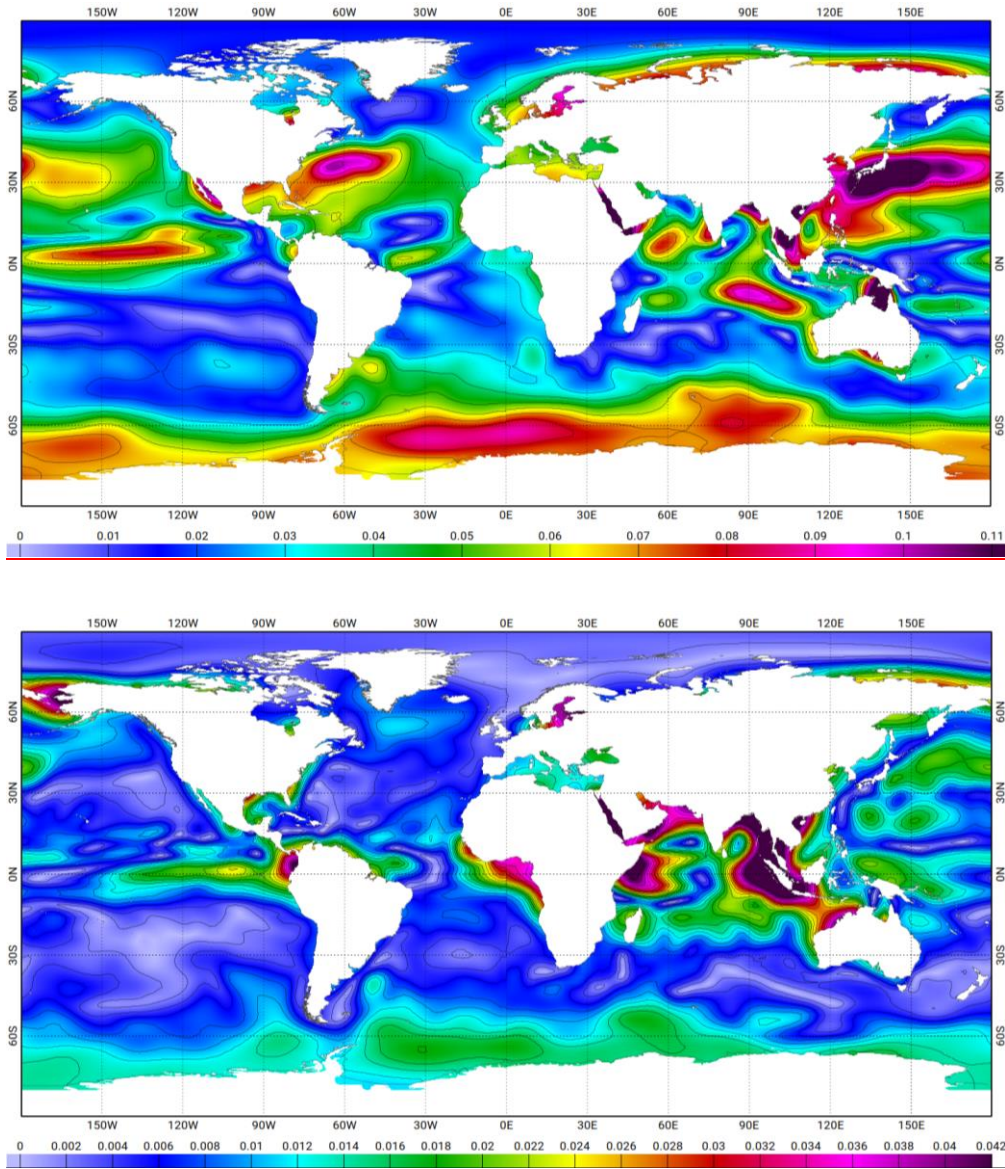
Figure 4 : maps Maps of amplitude in meters of S_a (upper panel) and S_{sa} (lower panel) ocean signals estimated from GLORYS2v1 reanalysis.
