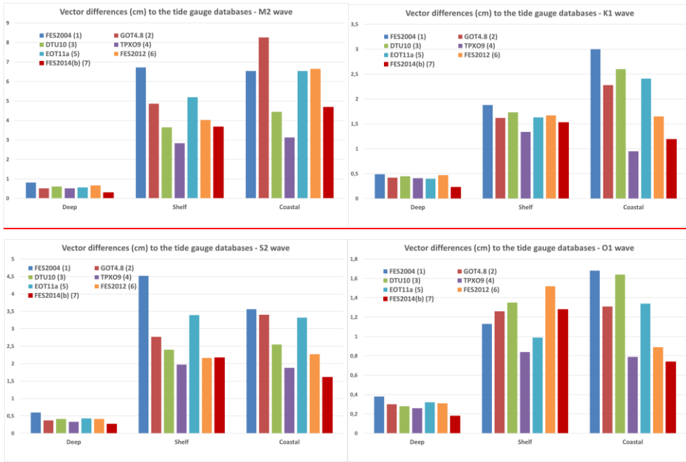
Figure 12: Vector differences (cm) between the tide-gauge (TG) databases and the global tidal models, for M2, K1, S2 and O1. Deep group is made of abyssal plain TGs, shelf made of tides gauges located in upper 500m depth limit. Coastal group is made of TGs collected in coastal data databases such as GLOSS.
