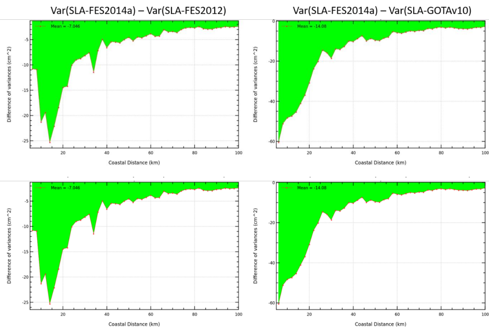
Figure 17 : Difference of variance of SLA for AL mission as a function of distance to coast, when using the new FES2014a tide model instead of FES2012 solution (on left) or GOT4v10 solution (on right) in the SSH calculation ( \text{cm}^2 ). AL cycles 1-14 are used. Tidal corrections made for both models with their native constituents spectrum (i.e. not restricted to their common constituents). When necessary, atlas solutions were extended toward the coast (low-order persistence).
