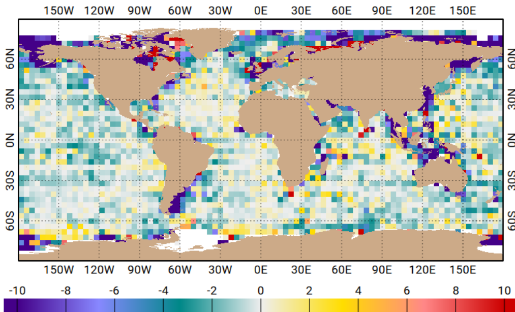
Figure 15 : maps Maps of SSH variance differences at crossovers using either the FES2014b tidal solution atlas or the GOT4v10 solution atlas in the SSH calculation for the Jason-2 mission (on the left, upper panel, J2 cycles 1-281) , and for AltiKa (on the right lower panel, AL cycles 1-21, in cm 2 ) . Blue colours indicate a higher variance reduction when using FES2014b tidal correction. Tidal corrections made for both models with their native constituents spectrum (i.e. not restricted to their common constituents).
