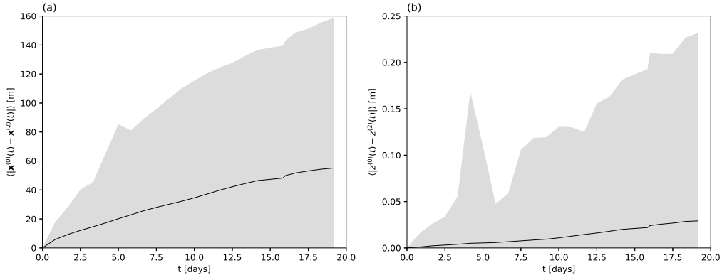
Figure B1. Solid line indicates the average horizontal distance d_h^I(t) (a) and the average vertical distance d_v^I(t) (b) of particles released from the same initial location but integrated with equations (1) and (B1) in the NEMO velocity field. Shaded region indicates the range of the distances among the individual pairs of particles.
