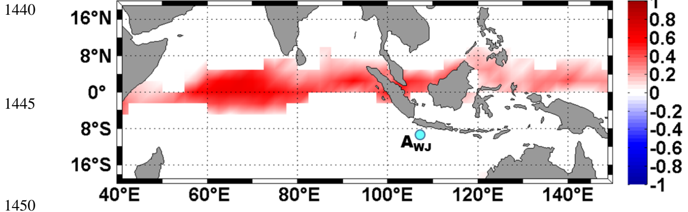
Figure 15. A correlation map between zonal wind and zonal currents (at 30 m) at A_{WJ} for the semiannual signals extracted using the EEMD method. The 95% significance level is approximately \pm 0.07 .
