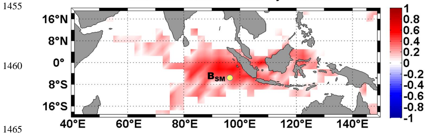
Figure 16. As in Figure 15, but at B_{SM} and for interannual signal.
