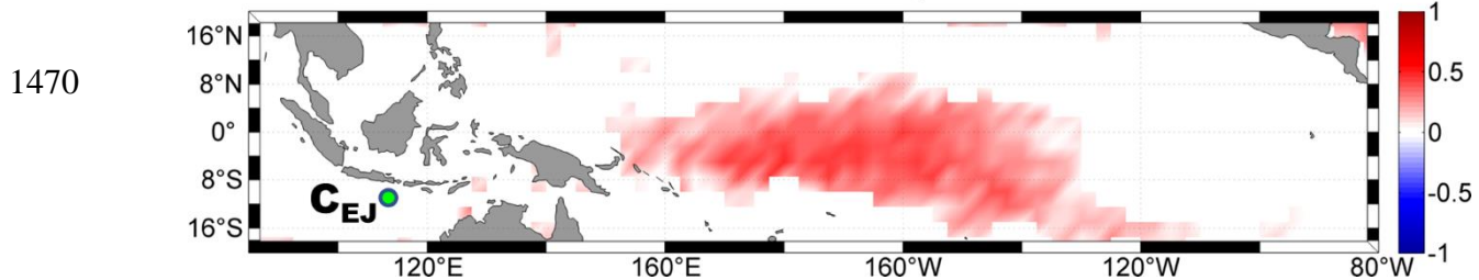
Figure 17. As in Figure 15, but at C_{EJ} and for interannual signal.
