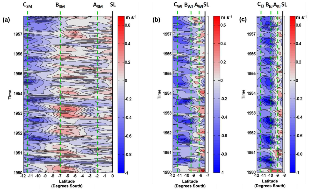
Figure 5. The zonal surface (1 m) currents along three meridional sections (yellow lines in Fig. 2): (a) SM (98°E), (b) WJ (107°E), and (c) EJ (113°E). Positive (negative) values of the zonal currents indicate eastward (westward). Meanwhile, green dash lines denote latitudes of the nine selected points and SL is shoreline.
