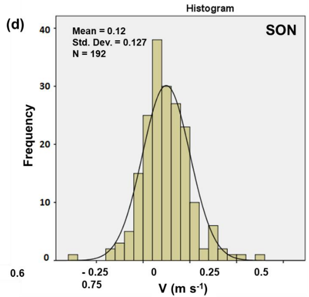
Figure 14. A probability distribution function of the EOF1 of zonal currents for each of the NW (a), SE (c), and transition (b and d) seasons at BSM at a depth of ~40 m.
