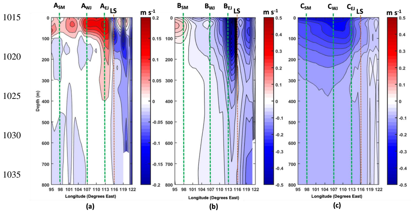
1040 Figure 4. Longitude-depth profiles of mean zonal currents along (a) Transect A, (b) Transect B, and (c) Transect C. Positive 1045 (negative) values of the zonal currents indicate eastward (westward). Green dash lines denote longitudes of the nine 1050 selected points, whereas dark orange dash lines denote longitude of Lombok Strait (LS).
