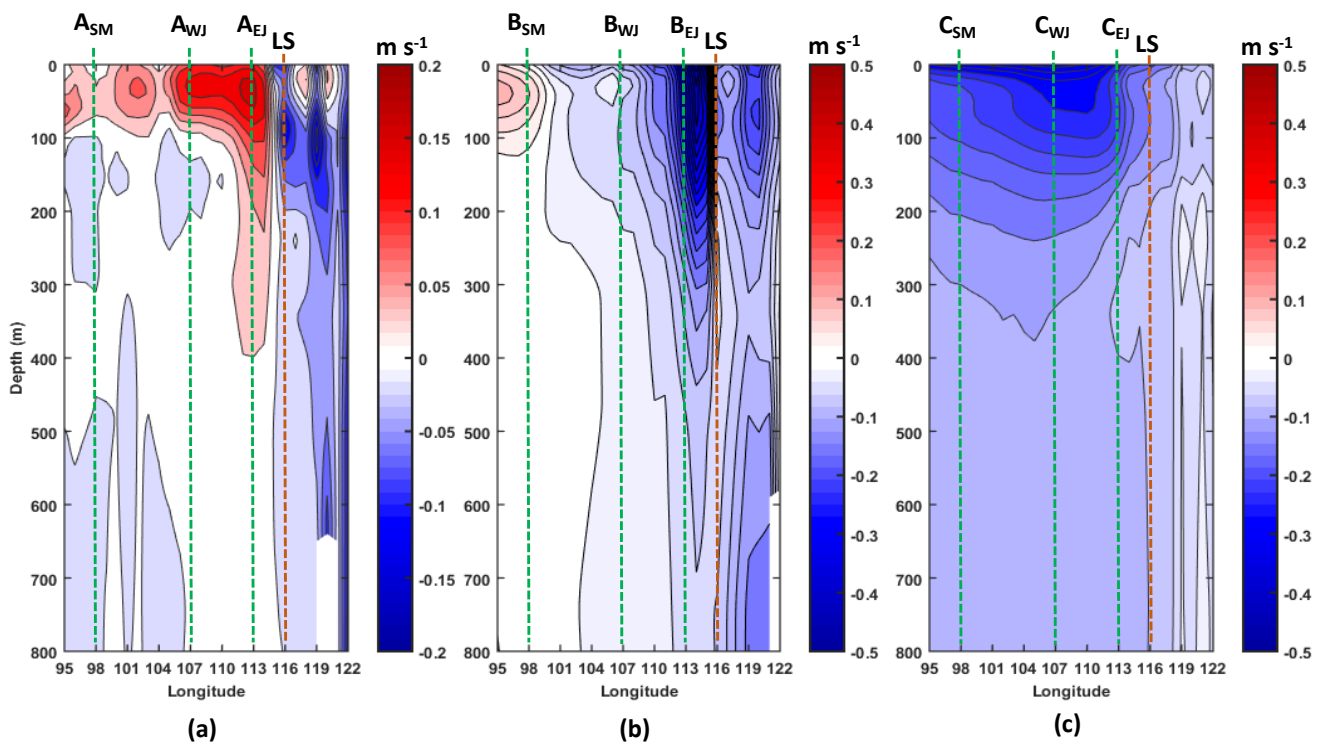
Figure 4. Longitude-depth profiles of mean zonal currents along (a) Transect A, (b) Transect B, and (c) Transect C. Positive (negative) values of the zonal currents indicate eastward (westward). Green dash lines denote longitudes of the nine selected points, whereas dark orange dash lines denote longitude of Lombok Strait (LS).
