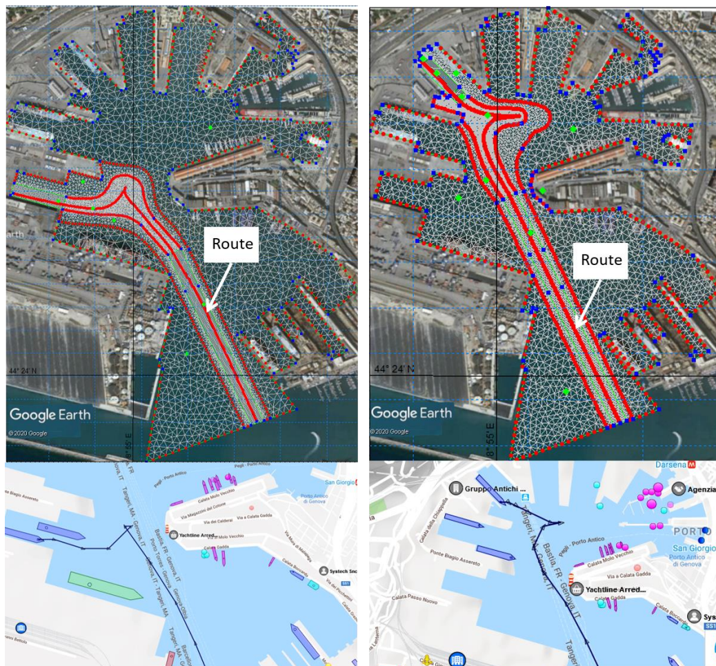
Figure 4 - Model domain and computational grids for docking routes of T1 (left panel) and T10 (right panel) docks. In the lower panels the corresponding actual routes are shown
