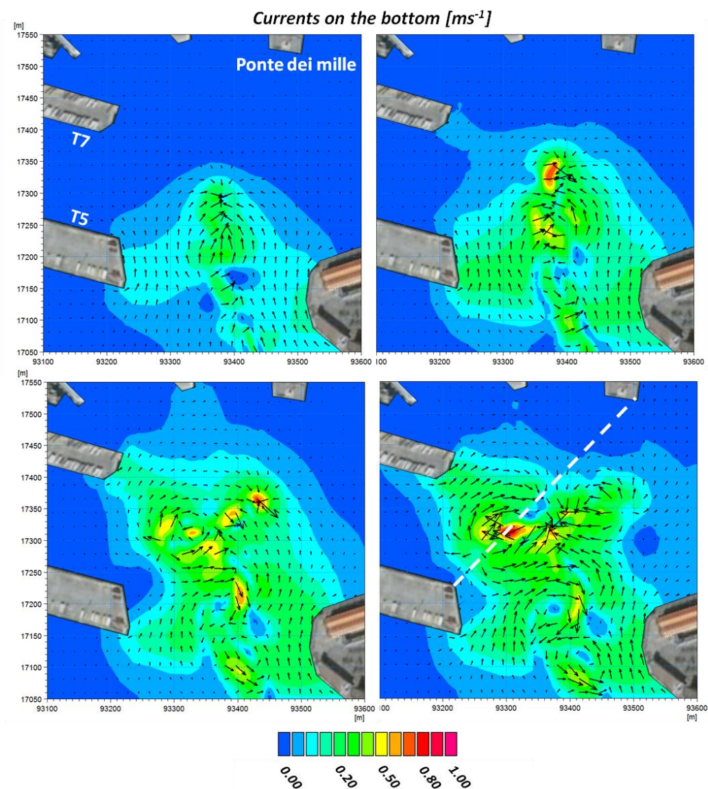
Figure 9 – Same as Figure 8 but for the bottom layer
