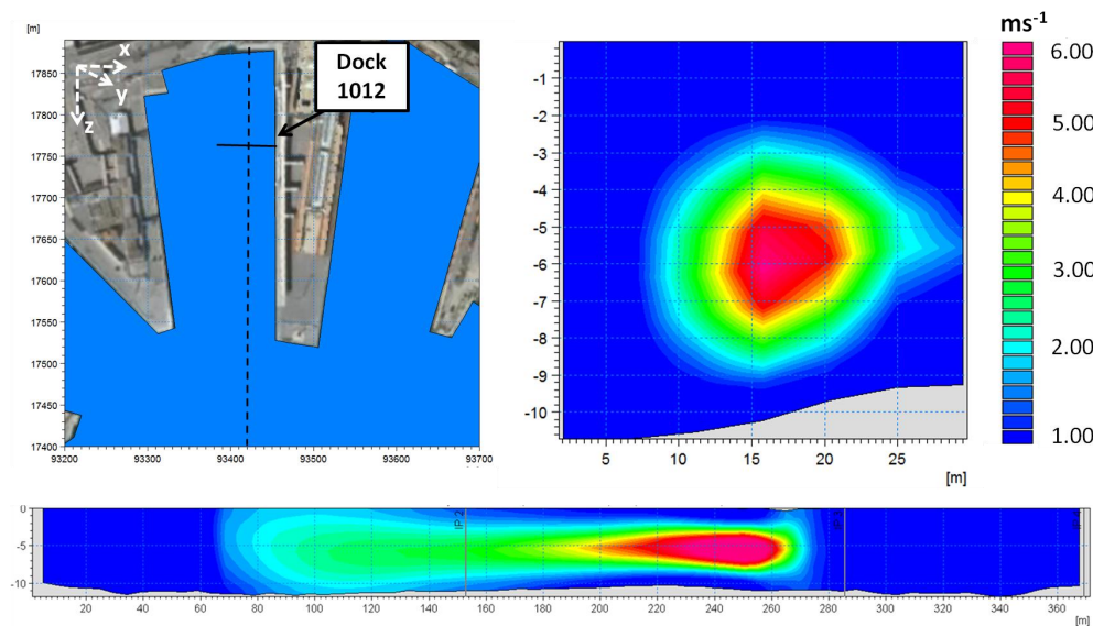
Figure 5 – Representation of the propeller-induced jet of the most representative ship departing from Dock 1012.
