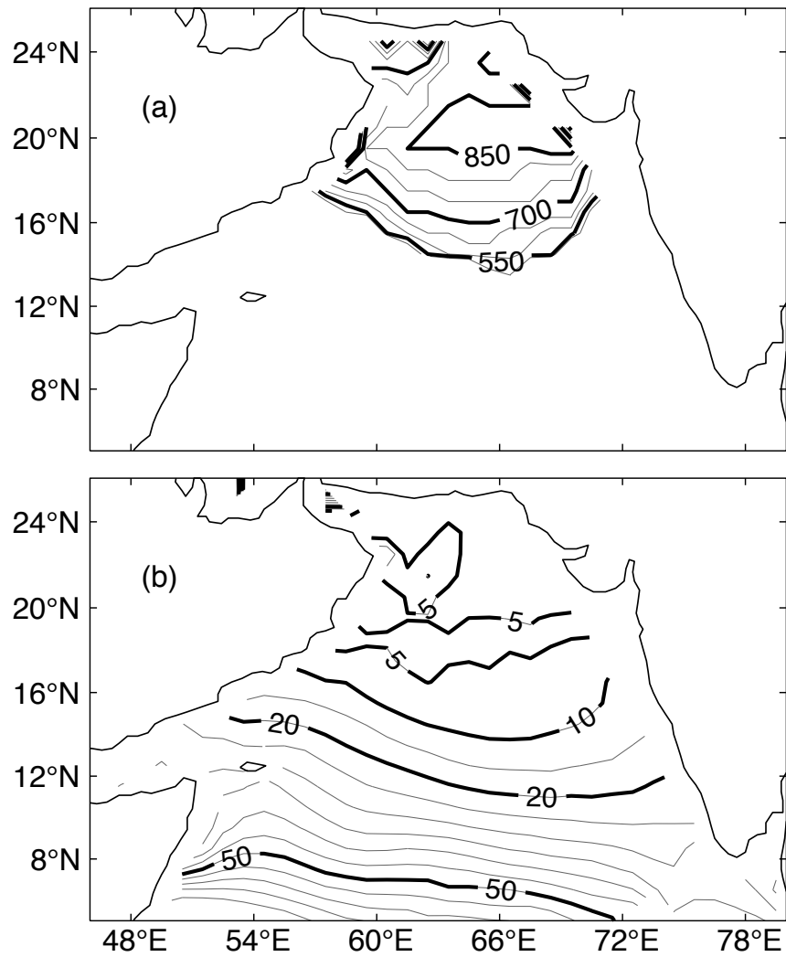
Figure 2: (a) Thickness (in m) of the layer containing oxygen of less than 10 \mu\text{mol/kg} based on climatological data from WOA 13. (b) Oxygen concentration (in \mu\text{mol/kg} ) on the \sigma = 27 \text{ kg/m}^3 isopycnal of WOA 13.
