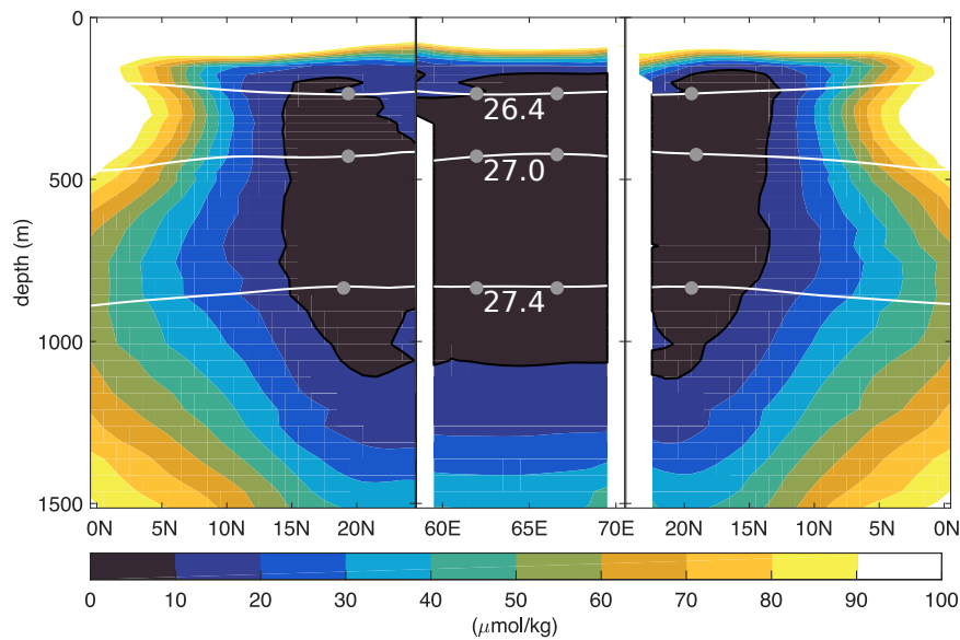
Figure 2: Annual mean of dissolved oxygen concentration along 62°E (left), 66.5° E (right) and 19° N (middle) from the WOA13 climatology (see Figure 1). Advective pathways from Lagrangian particles are calculated on three isopycnals (26.4, 27, 27.4 kg/m 3 ) shown as white lines. The grey dots mark the release points in the western (WR) and eastern (ER) basin on each isopycnal level.
