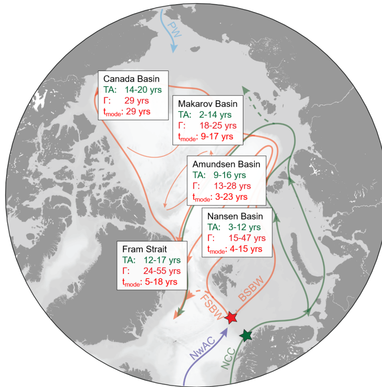
Figure 7. Summary of circulation times of Atlantic Water in the Arctic Ocean from this study: Tracer ages (TA) derived from the binary mixing model for the surface layer (green), mean ages ( \Gamma ) and mode ages ( t_{mode} ) derived from the TTD model for the mid-depth Atlantic layer (red).
