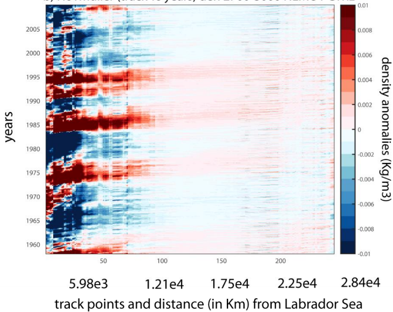
Figure 7. Hovmöller diagrams of density anomalies along the wave-track in the CTRL experiment. a) Map of the wave-track used in the study. The track-points correspond to the first point before the coast following the bathymetry at 3269 m. The points for all depth levels has been tracked. b) Density anomalies (in \text{kg}/\text{m}^3 ) along the track averaged from 2700m to 3000m levels for the CTRL experiment. The
