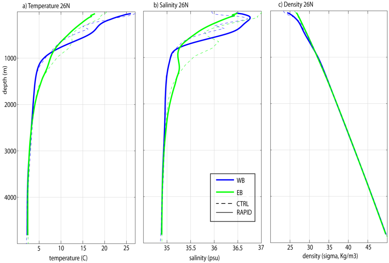
Figure 1. Temperature, salinity and density profiles at 26N. a) Temperature profiles (in °C) at 26N for WB (blue line) and EB (green line), CTRL experiment (dashed line) and RAPID data (solid line) for the period 2004-2009. b) same as a) but for salinity profiles. c) same as a) but for the density profiles.
