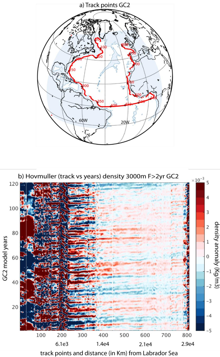
Figure 11. Hovmöller diagram of density along the wave track in the GC2 experiment. a) The track-points correspond to the first point before the coast following the bathymetry at 3138 m in GC2. b) Hovmöller diagram of density anomalies at 3000m along the wave
