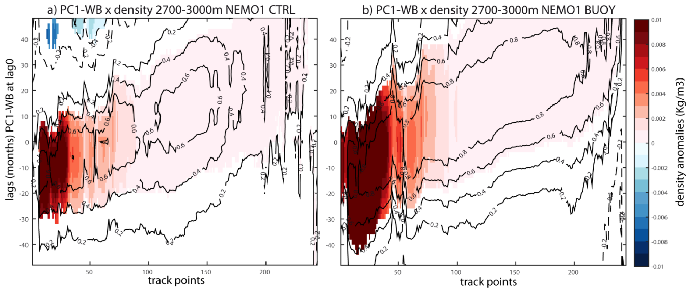
845 Figure 8. PC1-WB and density along the wave-track. a) Density anomalies (in kg/m 3 ) averaged from 2700m to 3000m projected onto PC1-WB for the CTRL experiment. Black lines correspond to the correlation every 0.2. Only significant areas are plotted with a Student's t-test at 95% confidence level considering only effective degrees of freedom. b) Same as a) but for the BUOY experiment.
