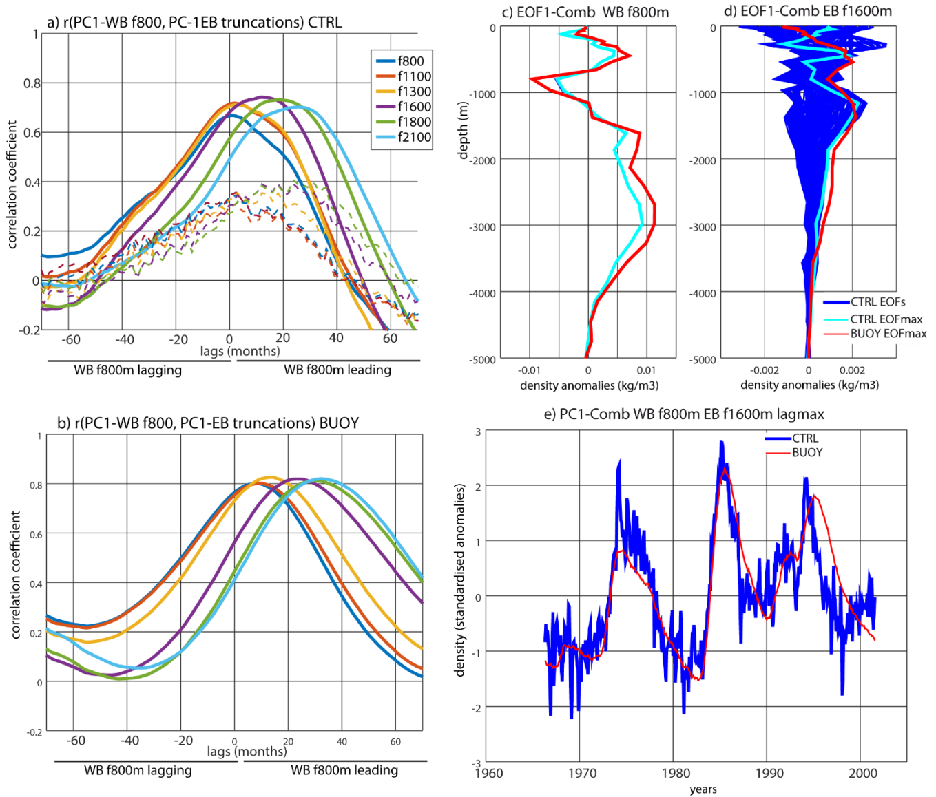
Figure 5. Relationship between Boundaries and the combined EOF. a) Lead-lag correlations between PC1-WB from 800m and PC1-EB at different truncations (represented with different colours). Positive (negative) values over x-axis represents the PC1-WB leading (lagging) the PC1-EB. 1-year running mean filter (solid line) and no filter (dashed line) is applied to the timeseries for the CTRL
