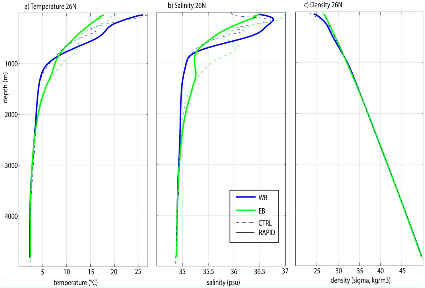
Figure 1. Temperature, salinity and density profiles at 26N. a) Temperature profiles (in °C) at 26N for Western Boundary (WB-↵, blue line) and Eastern Boundary (EB-↵, green line) for the CTRL experiment (dashed line) and the RAPID data (solid line) for the period 2004-2009. b) same as a) but for salinity profiles- (in psu). c) same as a) but for the density profiles- (in kg/m³).
