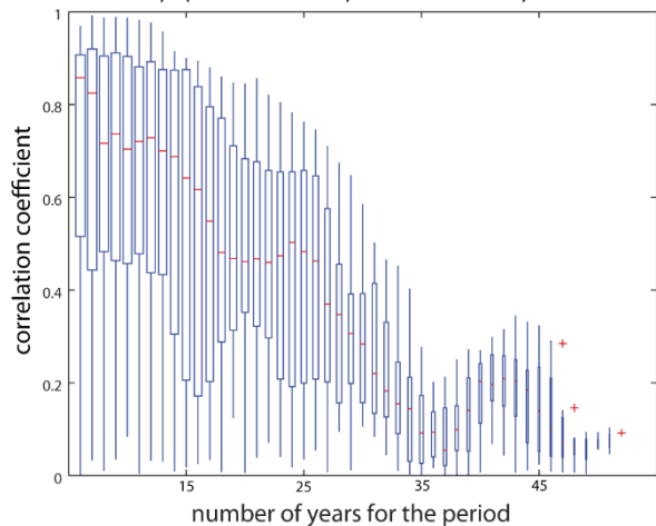
a) r(\text{PC1-WB CTRL}, \text{PC1-WB WIND})
