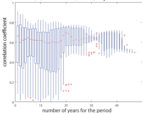
c) r(\text{PC1-WB CTRL}, \text{AMOC} > 2\text{yr})
