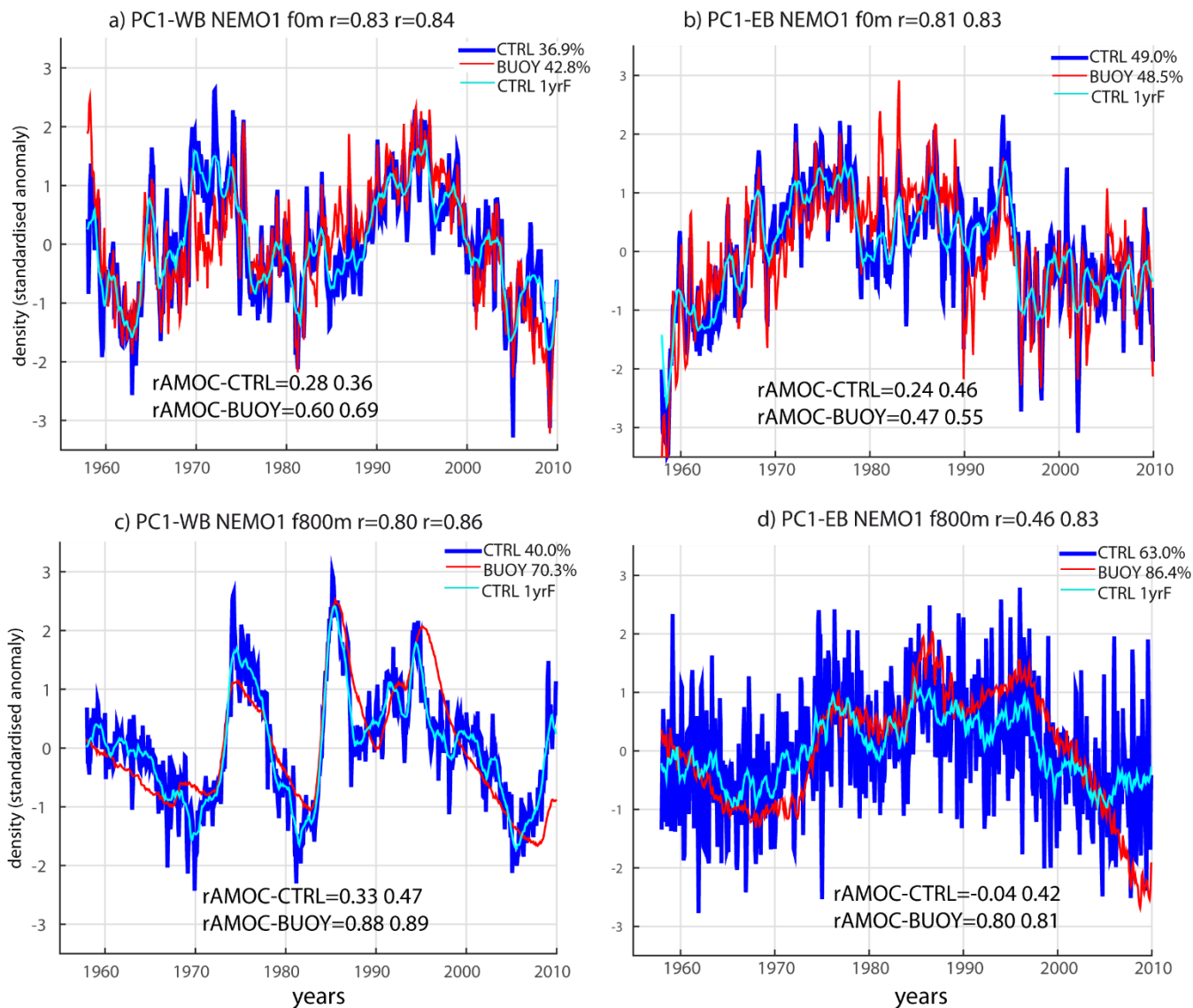
Figure 3 AMOC at 26N and individual EOF of density profiles at the 26N boundaries: sensitivity to depth truncation. a) Timeseries associated with the leading mode of density variability of the water column at the WB-26N for the CTRL (blue line) and BUOY (red line) experiment, considering (red line), using the total full water column. Cyan line corresponds to the time series timeseries of the CTRL smoothed with one-year running mean filter. In the title, double correlation score corresponds to correlations between blue-red and blue-cyan lines are detailed. b) Same as a) but for the EB-26N. c) -d) Same as a)-b) but considering the EOF analysis with profiles from 800m downwards. All the timeseries-Timeseries are dimensionless and the percentage of explained variance is detailed seen inset. Also on bottom, the legend as well as the correlation with AMOC timeseries (in Fig. 2a b). The correlation correlations between the CTRL PCs and BUOY experiments timeseries-the AMOC are detailed in the title, for the non-timeseries without filter and the 1-smoothed with one year
