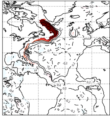
e) PC1WBxspa2700-3000m BUOY -20 months
