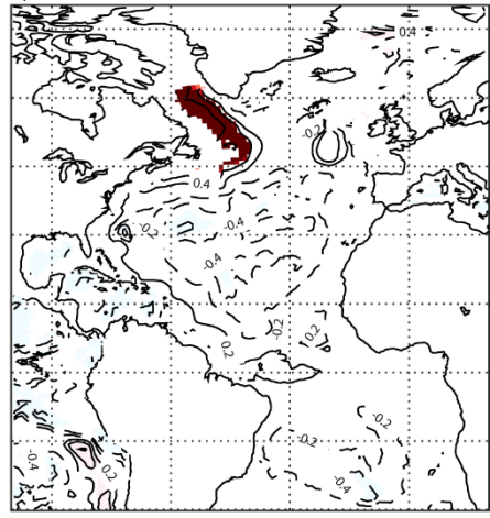
d) PC1-WB x den 2700-3000m BUOY -30 months
