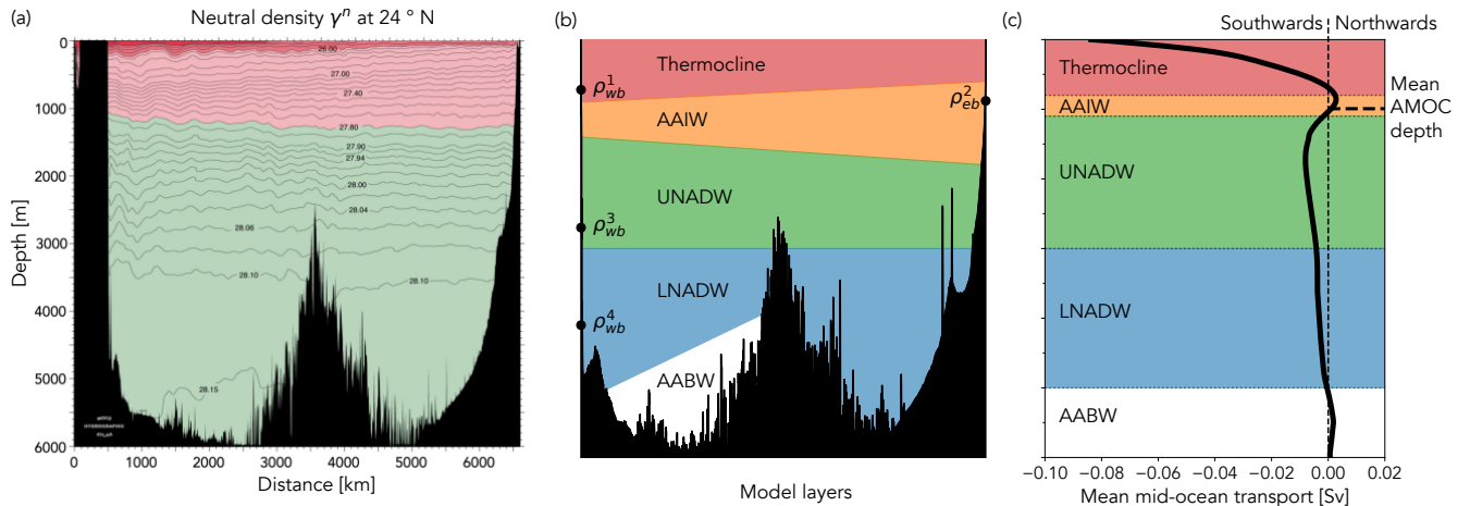
Figure 1. (a) World Ocean Circulation Experiment (WOCE) North Atlantic A05 section of neutral density \gamma^n [kg m^{-3}] at 24°N. From the WOCE Atlantic Ocean Atlas Vol. 3. (K. Koltermann, K.P., Gouretski, V.V., Jancke, 2011) (b) Schematic of four dynamic layers to be represented within the regression model by density anomalies at the western and eastern boundaries at a depth within each layer. The density anomalies are represented by the circular markers. (c) Profile of RAPID-estimated mean mid-ocean transport and the resulting northwards and southwards layer transports. Mean AMOC depth is around 1100 m.
