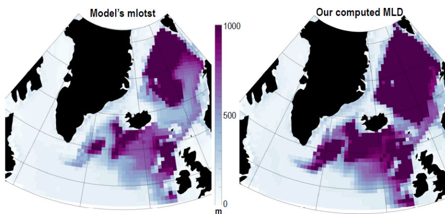
Figure A1. Maximum monthly mixed layer depth in the North Atlantic over 1985-2014 for the model CanESM5: left, using the model output 'mlotst'; right, when computed from the monthly temperature and salinity. Over the entire 30-year period, the root mean square error in the Nordic Seas is 305 m; in the subpolar gyre, 21 m.
