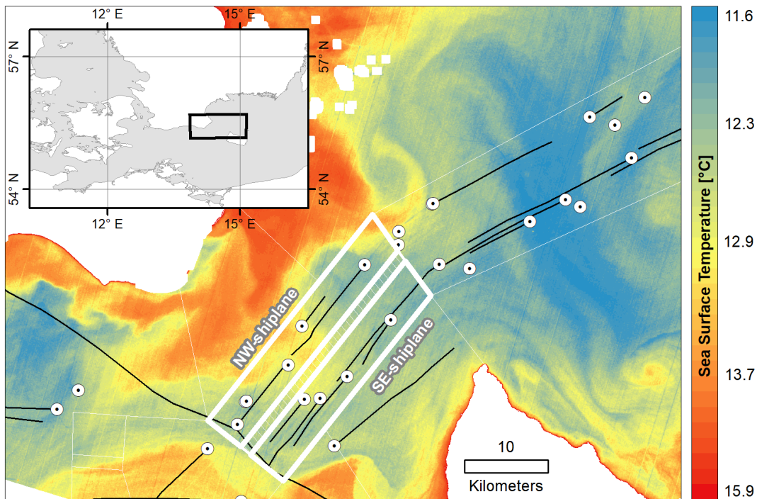
505 Figure 12. Ships and visible thermal wakes in the Bornholm sound from the analysed satellite scene from 2014-05-25 10:01. White circles with black dots indicate ships with an AIS transmitter present in the area at the time of the satellite passage, and the black lines are the digitalised visible thermal wakes from the satellite scene. White lines indicate the ship lane area, the bold lines mark the North-West and South-East ship lanes, and the dashed area is the traffic separation zone. Landsat-8 image courtesy of the U.S. Geological Survey.
