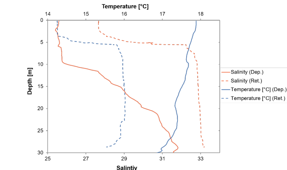
Figure 5: Salinity and temperature at the time of instrument deployment 28 August 2018 (solid lines) and retrieval 25 September 2018 (dashed lines).
