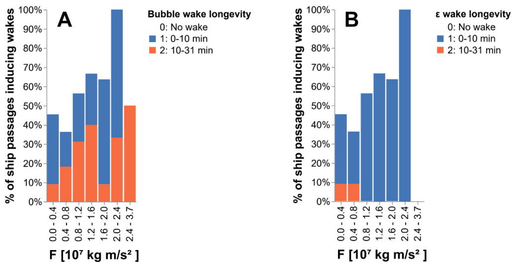
Figure 8. Wake longevity for the bubble wake (a) and dissipation rate of turbulent kinetic energy ( \epsilon ) wake (b), for detected wakes induced by ships passing at 0–3 ship widths from the instrument. The x-axis shows the force (F) of the vessel in Newton. Wake temporal longevitys < 10 min are shown in blue and wake longevitys 10–31 min are shown in orange.
