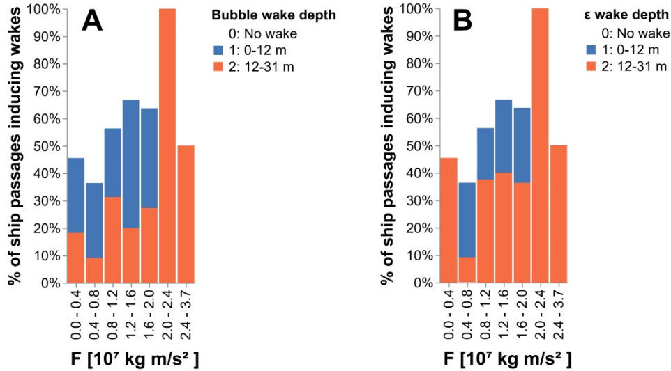
400 Figure 7. Maximum wake depth for the bubble wake (a) and dissipation rate of turbulent kinetic energy ( \epsilon ) wake (b) for detected wakes induced by ships passing at 0–3 ship widths from the instrument. The x-axis shows the force (F) of the vessel in Newton. Wake depths within the range presented in previous peer reviewed studies are shown in blue and wakes deeper than previously reported are shown in orange.
