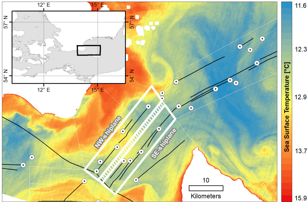
515 Figure 12. Ships and visible thermal wakes in the Bornholm sound from the analysed satellite scene from 2014-05-25 10:01. White circles with black dots indicate ships with an AIS transmitter present in the area at the time of the satellite passage, and the black lines are the digitalised visible thermal wakes from the satellite scene. White lines indicate the ship lane area, the bold lines mark the North-West and South-East ship lanes, and the hatched dashed -area is the traffic separation zone. Landsat-8 image courtesy of the U.S. Geological Survey.
