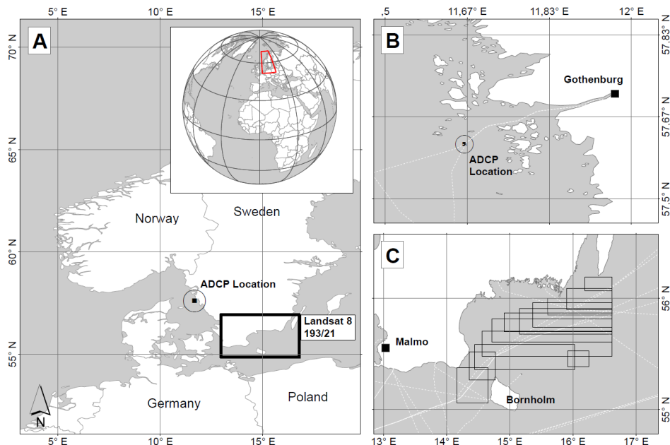
125 Figure 1: Overview of the two study areas (a) showing the location of the ADCP under the ship lane outside Gothenburg (b) and the area covered by the analysed satellite images (c). White dashed lines indicate ship routes of ferry lines and the boxes in (c) indicate the area defined as the ship lane area in the satellite image analysis. The ship lane and traffic separated zone north of Bornholm are shown in Figure 12.
