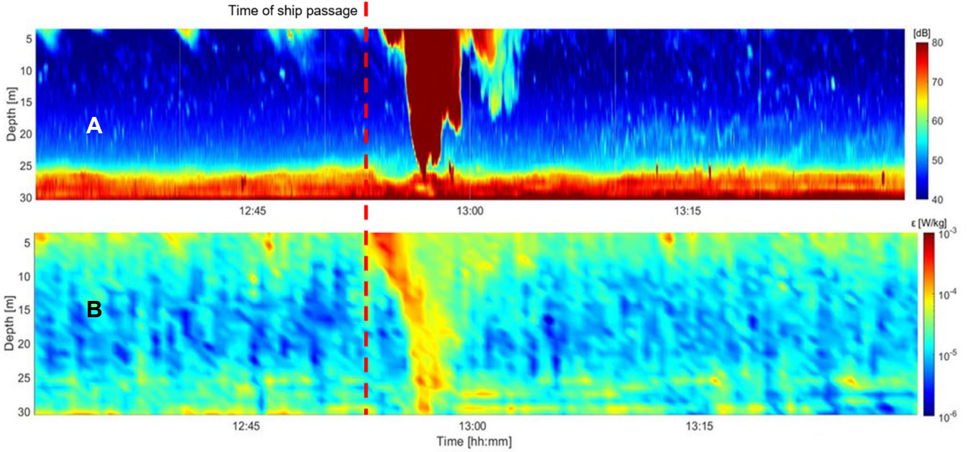
205 Figure 3: Example of the bubble wake signal in the echo amplitude dataset (a) and the calculated dissipation rate of turbulent kinetic energy, \epsilon , (b) from one hour of ADCP measurements. The upward facing ADCP was placed at 32 m depth, repeatedly measuring the water column in one point. The dashed red line marks the time of ship passage. The high intensity red (a) and yellow (b) areas after the ship passage represent the wake region. The increase of \epsilon down to the bottom is evidence of increased turbulence and a vertical mixing down to 30 m depth. The wake was induced by a cargo ship (width 25 m, length 229 m, draught 7 m), which passed the instrument at a distance of 34 m and a speed of 19 knots.
