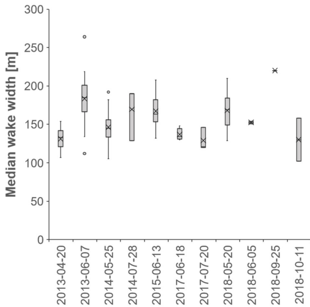
495 Figure 11. Median wake width distribution for the thermal wakes in the 11 satellite scenes with visible thermal wakes and < 23 % cloud cover, for the period April 2013 to December 2018. The median values are indicated with an X_ and outliers with rings (o). The lower and upper edges of the box represent the 25 th and 75 th percentile of the dataset, and the entire box represents the interquartile range (IQR). The top whisker extends to the largest value within a distance of < 1.5 times the IQR from the upper edge of the box, and the bottom whisker extends to the smallest value within a distance of ≤ 1.5 times the IQR of the lower edge of the 500 box. Values at a distance > 1.5 times the IQR from the box edges are considered outliers and indicated by rings (o).
