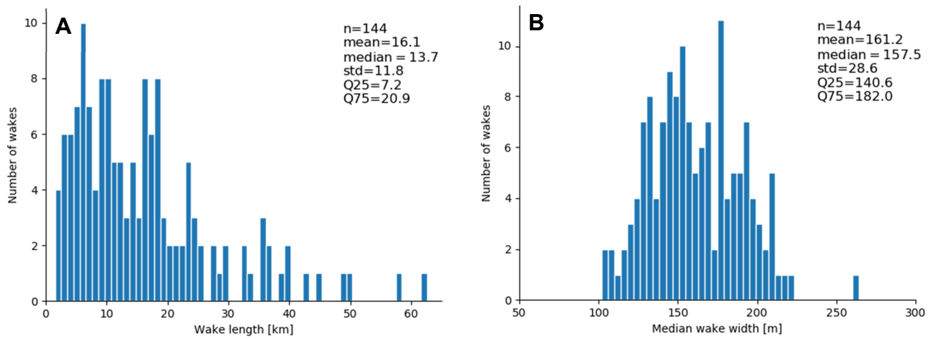
480 Figure 10. Distribution of observed thermal wake lengths (a) and widths (b), in the ship lane area indicated in Figure 1c. The observations are from satellite scenes with visible thermal wakes and < 23 % cloud cover, for the period April 2013 to December 2018 (n=144).
