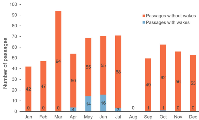
465 Figure 9. Seasonal distribution of ship passages for the satellite scenes with < 23 % cloud cover, for the period April 2013 to December 2018. The data labels in the stacked bar indicate the number of passages in each category. As some month has more than one analysed scene, the total number of ship passages for each month was divided by the number of analysed scenes, to get an average number of passages per scene for each month. August had no scenes with < 23 % cloud cover and therefore has no data.
