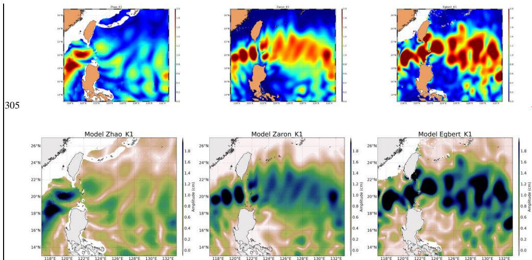
Figure 4 : amplitude of the IT models for K1 tide component, in the Luzon area.
