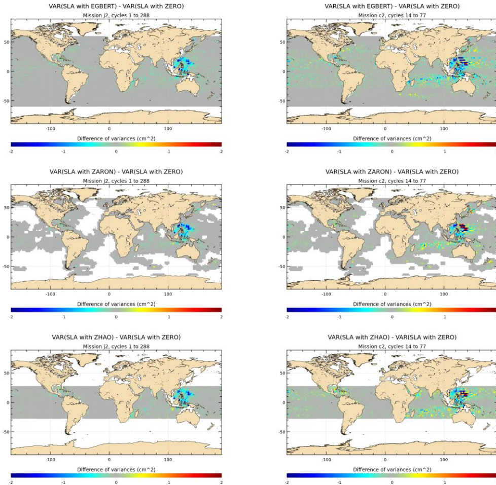
Figure B1 : Maps of SLA variance differences successively using each either O1 IT correction and from each model respectively or a reference ZERO correction in the SLA calculation , for J2 and C2 missions ( cm^2, cm^2 ). J2 cycles 1-288 have been used; C2 cycles 14-77 have been used.
