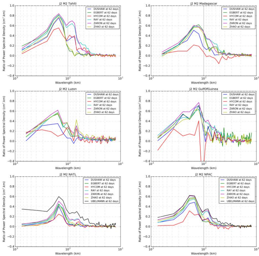
Figure 13 : Percentage Normalized difference of the IT signal removed by each IT model power spectral density of J2 SLA as a function of wavelength and for each IT region studied. Blue line= DUSHAW model, green= EGBERT model, red= HYCOM model, light blue= RAY model, purple= ZARON model, light green= ZHAO model, black= UBELMANN model.
