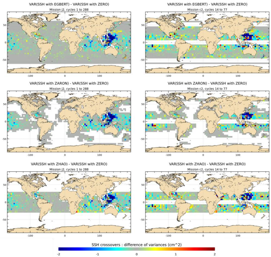
Figure 11 : Maps of SSH variance differences at crossovers successively using each either K1 IT correction and from each model respectively or a reference ZERO correction in the SSH calculation, for J2 and C2 missions (cm 2 ,cm 2 ). J2 cycles 1-288 have been used; C2 cycles 14-77 have been used.
