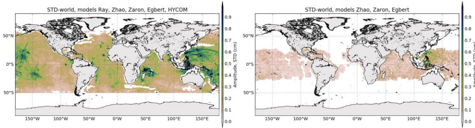
Figure 6 : global Global maps of standard deviation of the M2 (left) and K1 (right) IT models (cm)
