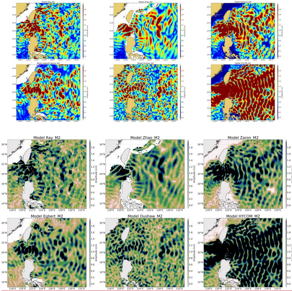
Figure 3 : amplitude Amplitude of the IT models for M2 tide component on Luzon area
