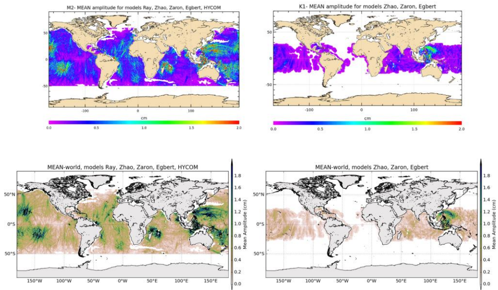
Figure 5 : global Global maps of mean amplitude of the M2 (left) and K1 (right) IT models (cm)
