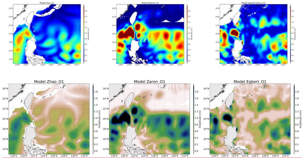
850 Figure A1: amplitude of the IT models for O1 tide component in Luzon area
