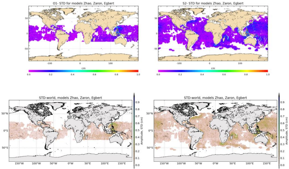
Figure A4 : global Global maps of standard deviation of the O1 (left) and S2 (right) IT models (cm)
