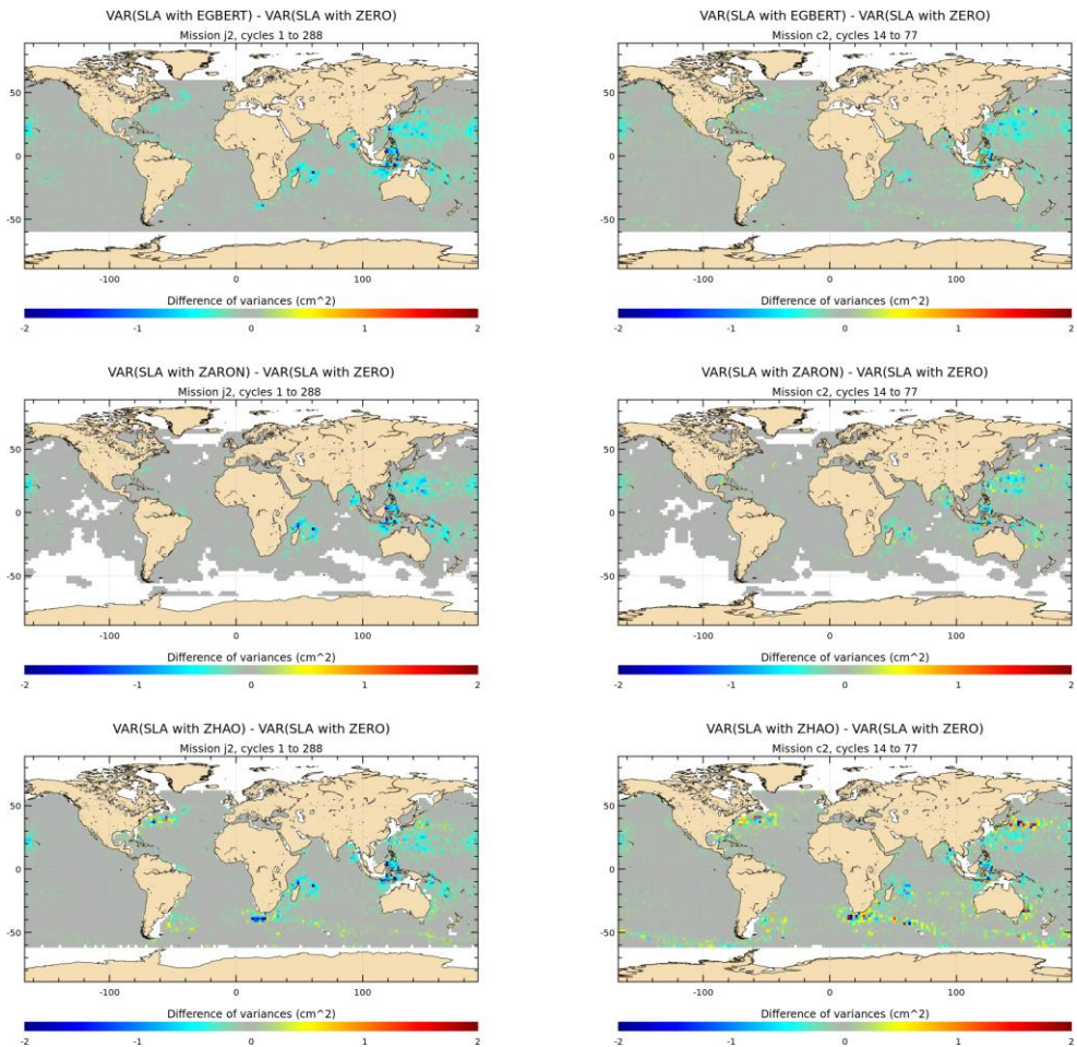
Figure C1 : Maps of SLA variance differences successively -using each either S2 IT correction and from each model respectively or a reference ZERO correction in the SLA calculation, for J2 and C2 missions (cm 2 ,cm 2 ). J2 cycles 1-288 have been used; C2 cycles 14-77 have been used.
