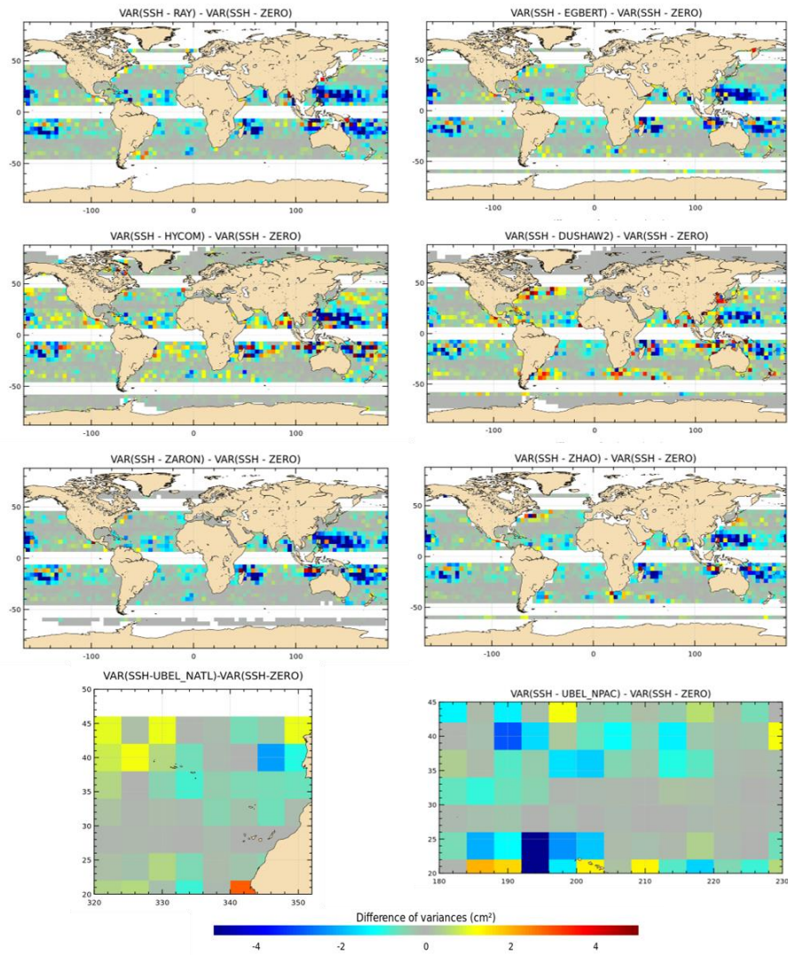
Figure 9 : Maps of SSH variance differences at crossovers successively using each either M2 IT correction and from each model respectively or a ZERO reference correction in the SSH calculation for C2 mission (cm 2 -cm 2 ). C2 cycles 14-77 have been used.
