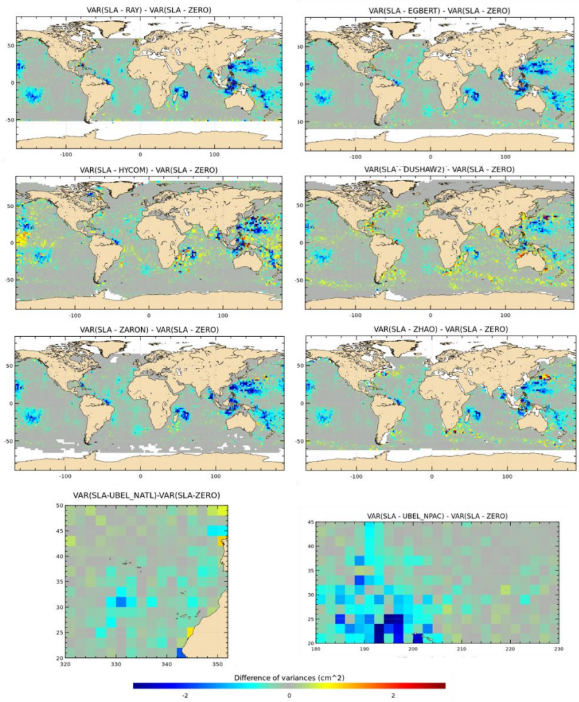
Figure 10 : Maps of SLA variance differences successively using each either M2 IT correction and from each model respectively or a ZERO reference correction in the SLA calculation for C2 mission ( \text{cm}^2 ). C2 cycles 14-77 have been used.
