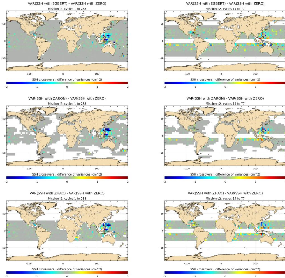
Figure B2 : Maps of SSH variance differences at crossovers successively using each either O1 IT correction and from each model respectively or a reference ZERO correction in the SSH calculation, for J2 and C2 missions (cm 2 -cm 2 ). J2 cycles 1-288 have been used; C2 cycles 14-77 have been used.
