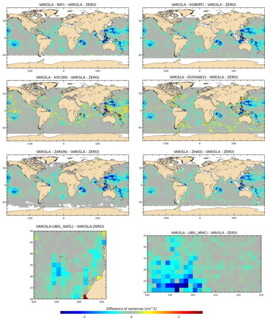
Figure 8 : Maps of SLA variance differences successively using each either M2 IT correction and from each model respectively or a ZERO reference correction in the SLA calculation for J2 mission (cm 2 -cm 2 ), J2 cycles 1-288 have been used.
