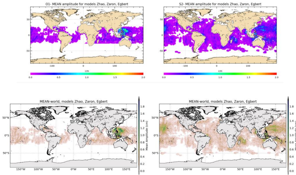
Figure A3 : global Global maps of mean amplitude of the O1 (left) and S2 (right) IT models (cm)
