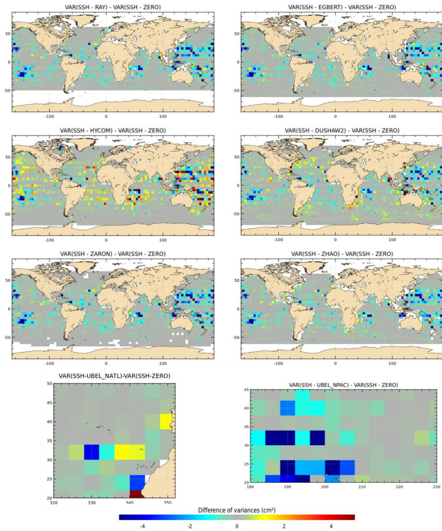
Figure 7 : Maps of SSH variance differences at crossovers successively using each either M2 IT correction and from each model respectively or a ZERO reference correction in the SSH calculation for J2 mission (cm 2 -cm 2 ). J2 cycles 1-288 have been used.
