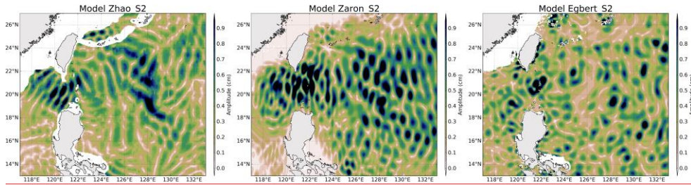
Figure A2 : amplitude Amplitude of the IT models for S2 tide component on in Luzon area
