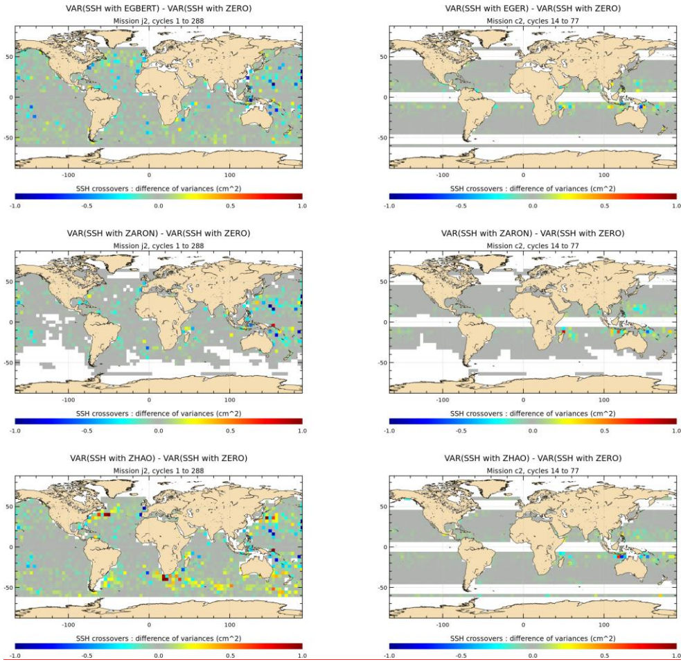
Figure C2: Maps of SSH variance differences at crossovers successively using each either S2 IT correction and from each model respectively or a reference ZERO correction in the SSH calculation, for J2 and C2 missions (cm 2 ,cm 2 ). J2 cycles 1-288 have been used; C2 cycles 14-77 have been used.
