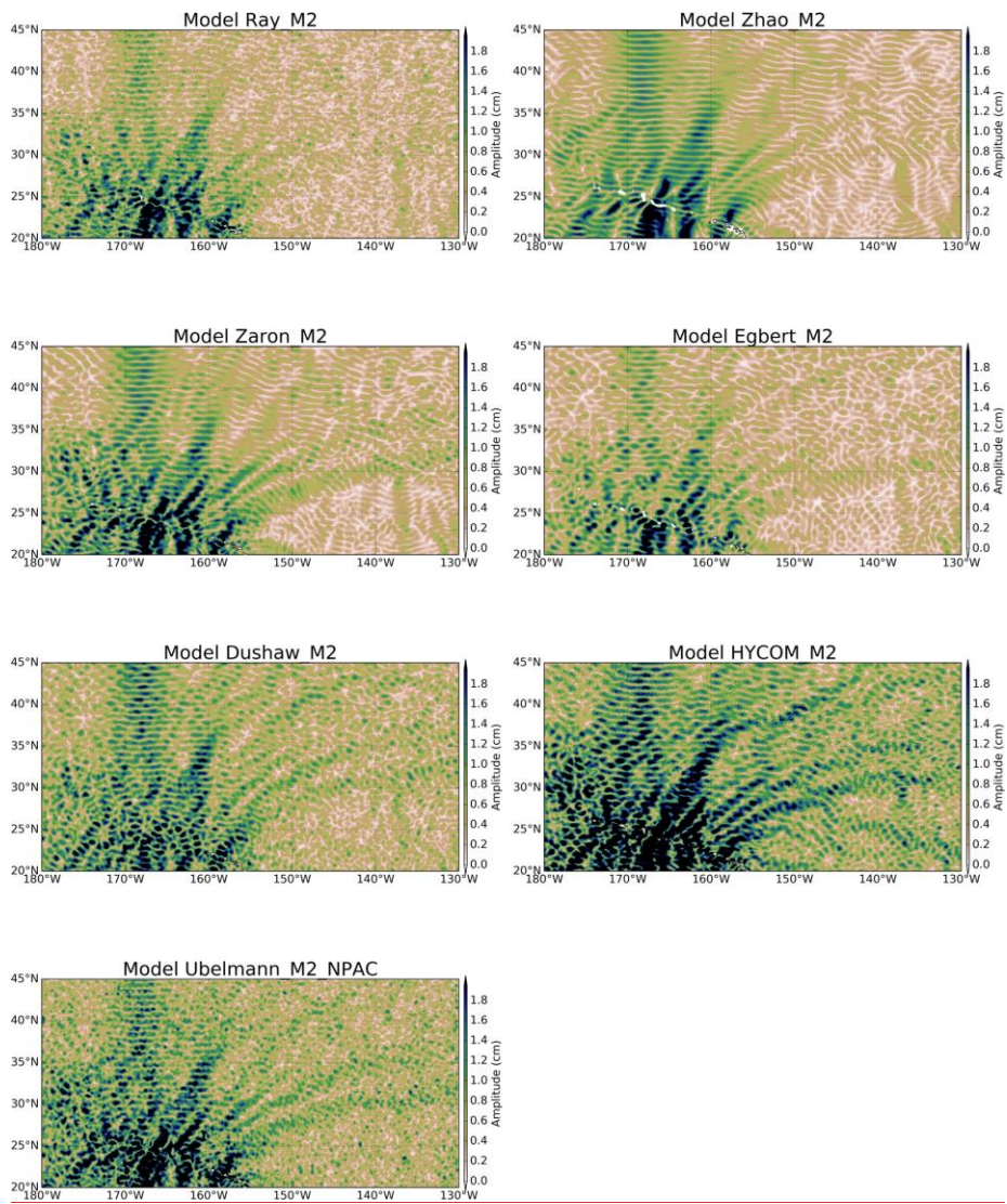
Figure 2 : amplitude Amplitude of the IT models for M2 tide component on NPAC region (north Hawaii)
