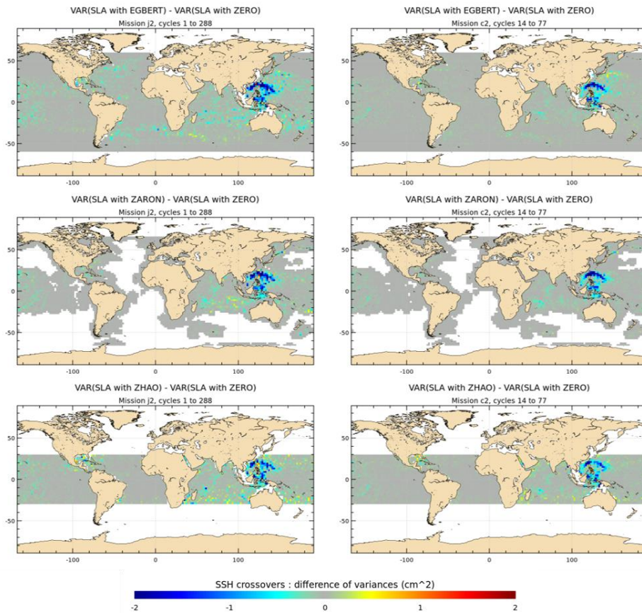
Figure 12 : Maps of SLA variance differences successively using each either K1 IT correction and from each model respectively or a reference ZERO correction in the SLA calculation, for J2 and C2 missions (cm 2 -cm 2 ). J2 cycles 1-288 have been used; C2 cycles 14-77 have been used.
