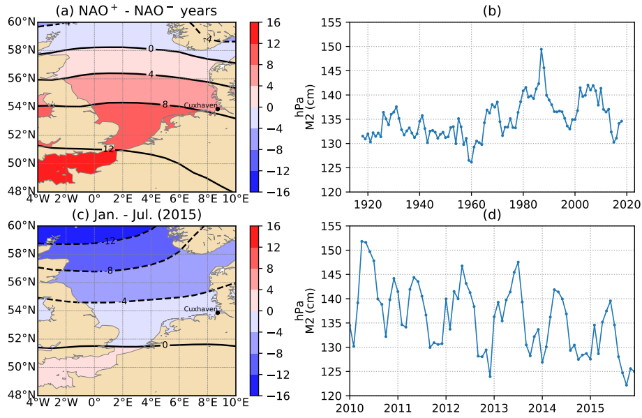
Figure 12. At decadal time scale: (a) Difference of winter sea-level pressure between 1989 (NAO + ) and 1969 (NAO - ) in the North Sea (b) Annual M_2 amplitude at Cuxhaven from 1918 to 2018. At seasonal time scale: (c) Difference of monthly sea-level pressure between January and July 2015 in the North Sea (d) Monthly M_2 amplitude at Cuxhaven from January 2010 to December 2015. Contour intervals are every 4 hPa in (a) and (c).
