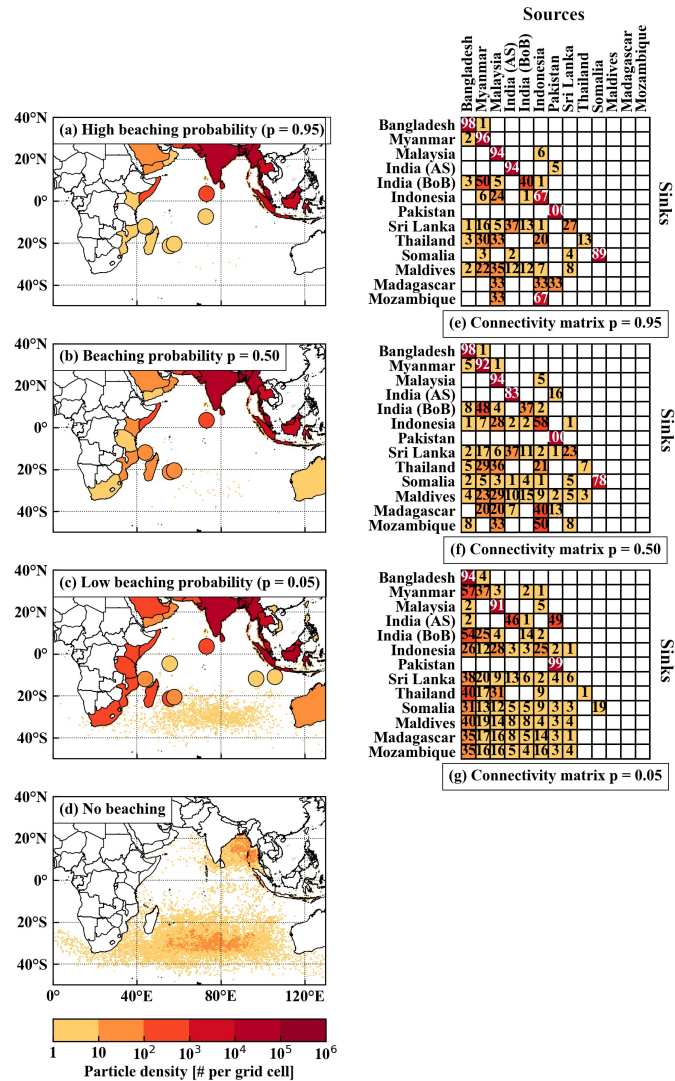
Figure 5. Density of beached particles per country or island and density of particles in the ocean per 0.5 \times 0.5^\circ grid cell for particles released from river source locations in the northern hemisphere Indian Ocean after 21 years of simulation, with: (a) “high” beaching probability, p = 0.95/5 days (10 year animation of simulation results available at http://doi.org/10.5446/47058 ); (b) beaching probability of p = 0.50/5 days (10 year animation of simulation results available at http://doi.org/10.5446/47057 ); (c) “low” beaching probability, p = 0.05/5 days (10 year animation of simulation results available at http://doi.org/10.5446/47056 ); (d) no beaching. Filled circles highlight islands which do not clearly show up on the map otherwise, from north to south these represent: Maldives, Seychelles, British Indian Ocean Territory, Christmas Island, Cocos (Keeling) Islands, Comoros, Mauritius, and Réunion. Connectivity matrices showing the percentage of particles that beach in selected countries (rows) against countries of origin (columns), for: (e) “high” beaching probability, p = 0.95/5 days; (f) beaching probability of p = 0.50/5 days; and (g) “low” beaching probability, p = 0.05/5 days. In these matrices, India is split into a western (bordering the Arabian Sea, “India (AS)”) and an eastern side (bordering the Bay of Bengal, “India (BoB)”). Note that the sum of each row does not always precisely equal 100 % because: not all countries with river plastic sources are shown, percentages are rounded to integer numbers, and percentages below 1 % are omitted.
