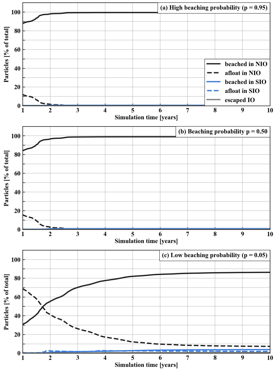
Figure 4. Percentage of total simulated particles as a function of the simulation duration that have: beached in the northern (NIO) or southern hemisphere Indian Ocean (SIO); are afloat in the NIO or SIO; or that have left the Indian Ocean entirely, for: (a) a “high” beaching probability of p = 0.95/5 days; (b) a beaching probability of p = 0.50/5 days; (c) a “low” beaching probability of p = 0.05/5 days. Percentages are shown after all particles have been released after 1 year of simulation, and up to 10 years of simulation, after which the simulation results have reached a steady state in all cases.
