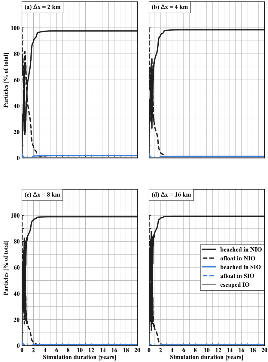
Figure A5. Sensitivity analysis results where beaching occurs with a probability p = 0.50/5 days for particles within a distance \Delta x = [2, 4, 8, 16, 32] km to the nearest coastline that are moving towards the coast. Results are not very sensitive to different values for \Delta x , and we use \Delta x = 8 km as the default value in further simulations.
