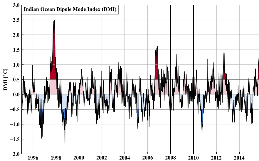
Figure A3. Indian Ocean Dipole Mode Index (DMI) as defined by Saji et al. (1999) and obtained from the National Oceanic and Atmospheric Administration. Red and blue shading indicate positive and negative modes of the Indian Ocean Dipole (IOD) respectively. We use 2008 and 2009 (marked between thick black vertical lines) as neutral IOD years to simulate the influence of monsoon seasons on the transport of plastics in the Indian Ocean.
