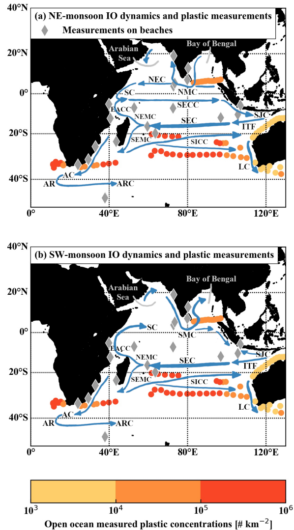
Figure 1. Overview of standardised open ocean plastic measurements in the Indian Ocean (filled circles); approximate locations of sampling studies of plastics on beaches (grey diamonds); and schematic dominant ocean surface currents (blue arrows) during the (a) northeast monsoon season; and (b) southwest monsoon season. Open ocean sampling studies were performed by Morris (1980); Reisser et al. (2013); Eriksen et al. (2014); Cózar et al. (2014) and standardised by van Sebille et al. (2015). Sampling studies of plastics on beaches were performed by Ryan (1987); Slip and Burton (1991); Madzema and Lasiak (1997); Uneputtu and Evans (1997); Barnes (2004); Jayasiri et al. (2013); Duhec et al. (2015); Nel and Froneman (2015); Bouwman et al. (2016); Kumar et al. (2016); Imhof et al. (2017); Lavers et al. (2019). Schematic ocean surface currents are based on Schott et al. (2009). The following currents are shown and labeled with their abbreviations: Northeast Monsoon Current (NMC) and Southwest Monsoon Current (SMC); North Equatorial Current (NEC); Somali Current (SC); South Equatorial Counter Current (SECC); South Java Current (SJC); East African Coastal Current (EACC); Indonesian Throughflow (ITF); North-east Madagascar Current (NEMC); Southeast Madagascar Current (SEMC); Agulhas Current (AC); Agulhas Retroreflection (AR); Agulhas Return Current (ARC); South Indian Counter Current (SICC); Leeuwin Current (LC).
