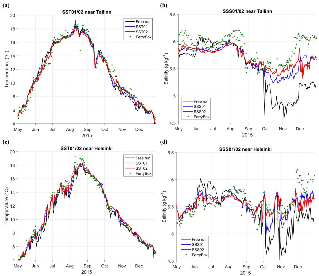
Figure 7: Time series of SST (a, c) and SSS (b, d) near Tallinn (a, b, 59.4833° N, 24.7667° E) and Helsinki (c, d, 59.9500° N, 24.8833° E), locations shown in Fig. 2a. FerryBox data are shown by dots, black lines represent control run without DA, red lines correspond to DA with relaxation time 5 days (weight of observations 0.2), blue lines for 10 days (weight 0.1).
