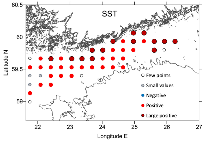
Figure 9: Improvement of RMSD of DA compared to that of FR, both taken in reference to 110 k FerryBox observations. Comparison is made for 20 x 20 grid cells (10' N x 20' E) for SST (a) and SSS (b) over the whole study period. Legend codes: few points - less than 100 observations in a box, small values - absolute percentage change less than 10%, negative - DA RMSD growth more than 10%, positive - DA improvement (RMSD reduction) from 10% to 30%, large positive - improvement more than 30%.
