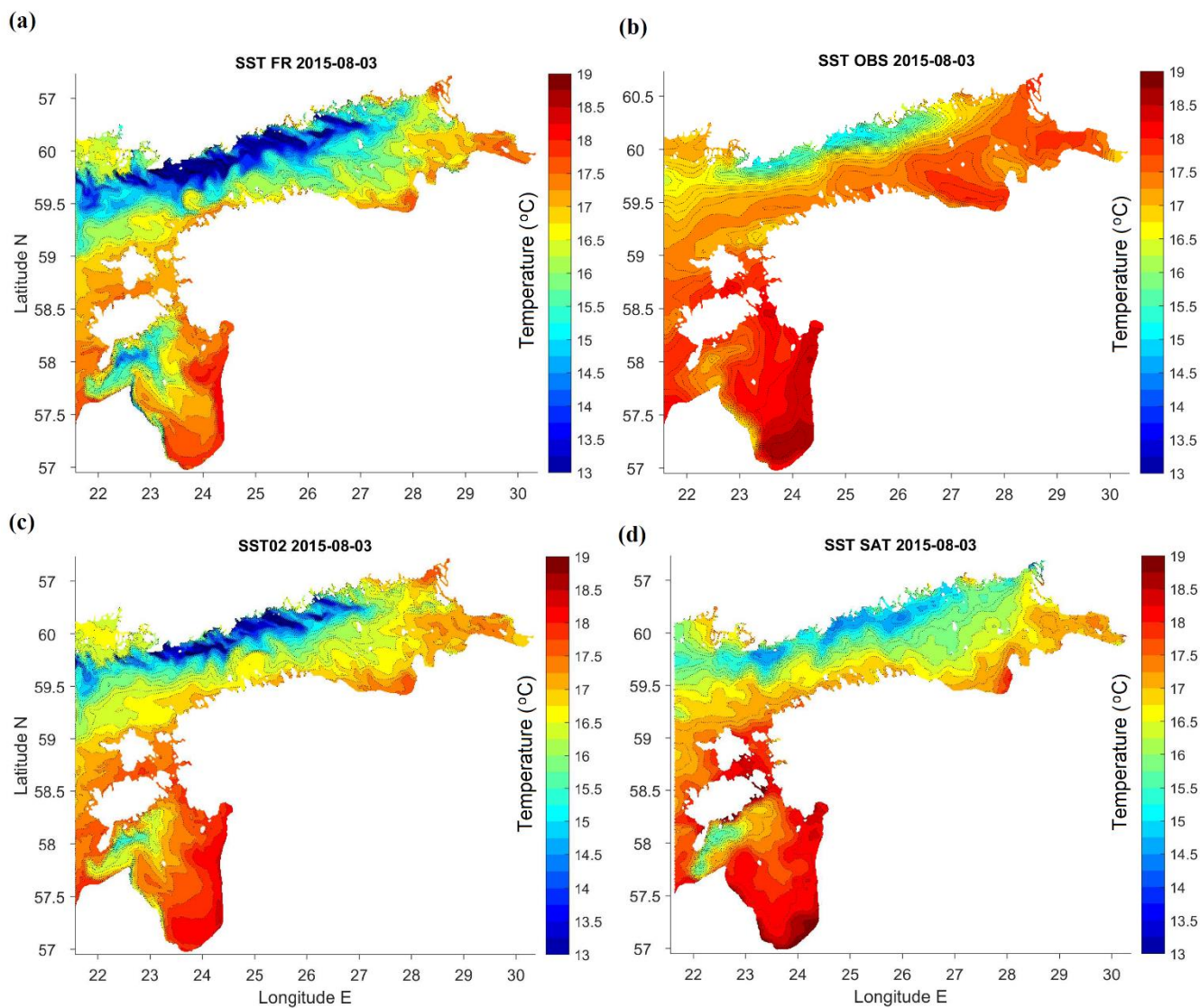
800 Figure 5: Maps (longitude E, latitude N) of SST in the study area on 3 August 2015: (a) free model run without DA, (b) observations reconstructed using EOF method, (c) DA with relaxation time 5 days (weight of observations 0.2), (d) satellite observations.
