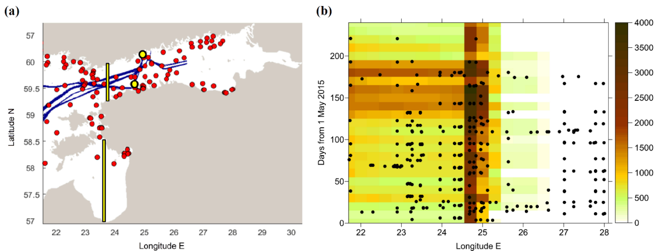
775 Figure 2: Distribution of observations. (a) Map of FerryBox observation points along ship tracks (blue) and shipborne monitoring observations (red) over the study period. Shown are also the locations for time-latitude graphs and time series (black contours with yellow background). (b) Observation frequency over longitude and time. FerryBox data are shown by colour image; each image cell presents the number of initial observations over intervals of 10 days and 18' E longitude. Shipborne observations are shown by black dots.
