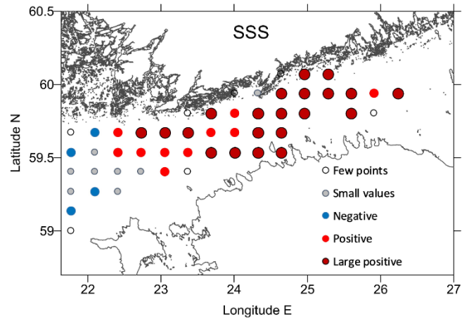
Figure 9: Improvement of RMSD of DA compared to that of FR, both taken in reference to 110 k FerryBox observations. Comparison is made for 20 x 20 grid cells (10' N x 20' E) for SST (a) and SSS (b) over the whole study period. Legend codes: few points - less than 100 observations in a box, small values - absolute percentage change less than 10%, negative - DA RMSD growth more than 10%, positive - DA improvement (RMSD reduction) from 10% to 30%, large positive - improvement more than 30%.
