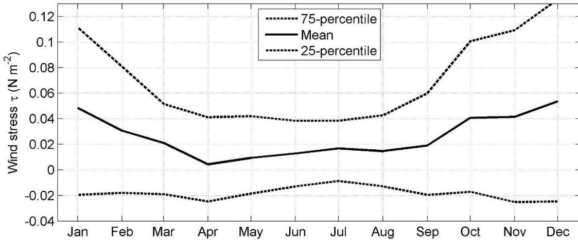
Fig. 7. Annual cycle of an along-gulf component of wind stress. Mean (solid black curve, positive eastward), 75- and 25-percentiles (dashed lines) are based on data from 1981-2015, measured at Kalbådagrund Lighthouse, Gulf of Finland.
