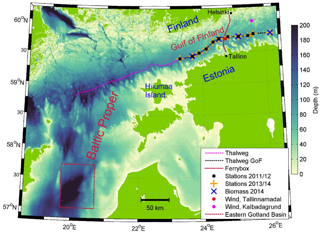
630 Fig. 1. Bathymetric map of the Baltic Proper and the Gulf of Finland. The locations of the CTD stations along the gulf (Thalweg GoF) visited in 2011/12 and 2013/14, phytoplankton biomass sampling stations along the gulf in 2014, transect from the northern Baltic Proper to the central Gulf of Finland (Thalweg + Thalweg GoF), Tallinn–Helsinki Ferrybox line, Tallinnamadal and Kalbådagrund wind measurements locations and Eastern Gotland Basin (box) area are shown.
