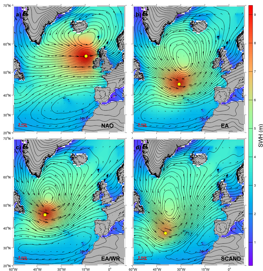
Figure 9. Winter atmospheric situations for the positive phase of a) NAO, b) EA, c) EA-WR and d) SCAND indices in the North Atlantic Ocean. The vectors represent the 10 m wind speed in m/s; the contours, the sea level pressure in Pa and the color range is the mean value of SWH in m. The red left bottom arrow represents the wind scale.
