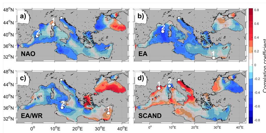
Figure 8. Pearson correlation coefficient of winter mean 99 th percentile SWH Mediterranean Sea series and a) NAO, b) EA, c) EA-WR and d) SCAND winter mean indices. No significant values at the 90% confidence interval are dotted. The white points show 1) the maximum positive and 2) the maximum negative value of correlation coefficient.
