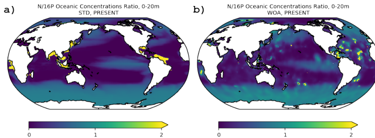
Figure 5: Molar oceanic ratios N:16P averaged in the upper 20m for PRESENT, as calculated by the model (a) for the STD simulation, and based on World Ocean Atlas (WOA; Garcia et al., 2010b) data (b). Values >1.0 denote overshoot of N vs P relative to the Redfield ratio (C:N:P = 122:16:1); blue areas indicate a surplus of P or deficiency of N.
