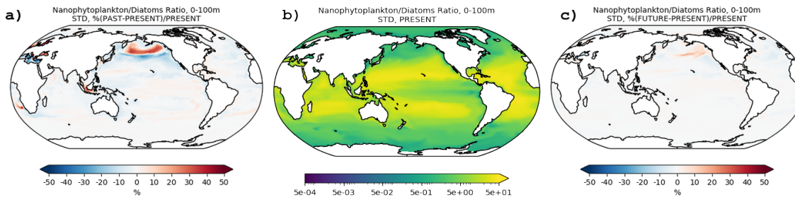
Figure 6: Nanophytoplankton to diatoms oceanic concentrations ratio averaged in the upper 100m for PRESENT (b) for the STD simulation, and the relative changes to PAST (a) and FUTURE (c).
