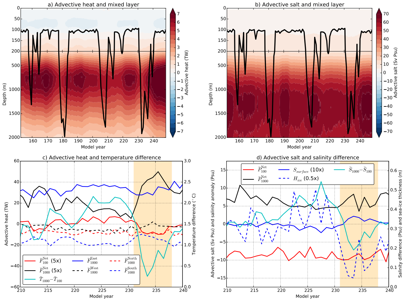
Figure 9. (a): Hovmöller diagram of the vertical distribution of heat input along the eastern boundary of the Polynya region ( 11^{\circ} E, 63.5^{\circ} S – 66.5^{\circ} S). Positive (negative) values indicate heat advection advected into (out of) the Polynya region. The time series are smoothed by a 60-month running mean. The black curve again indicates the (annual maximum) mixed layer depth of the Polynya region. (b): Similar to a), but now for the salt input. (c): The horizontal heat input over the Polynya region boundaries over the model years 210 – 240, where positive (negative) values of \bar{F} indicate accumulation (depletion) of heat in the Polynya region over the corresponding vertical extent. The net horizontal heat input over the Polynya region boundaries are indicated by \bar{F}^{Net} (magnified by a factor 5) over the corresponding vertical extent. The cyan curve is the temperature difference between subsurface ( \bar{T}_{1000} ) and surface ( \bar{T}_{100} ) over the Polynya region. All the time series consists of yearly averages and the shading indicates the last multiyear MRP event. (d): Similar to c), but now for the net advective salt input ( \bar{P}_{100}^{Net} and \bar{P}_{1000}^{Net} ). The cyan curve is the salinity difference between subsurface ( \bar{S}_{1000} ) and surface ( \bar{S}_{100} ) over the Polynya region. In addition, the blue curve shows the yearly-averaged surface salinity anomaly with respect to model year 210 ( S_{surface} , magnified by a factor 10) and the dashed blue curve displays the annual maximum sea-ice thickness ( H_{ice} , reduced by a factor 2).
