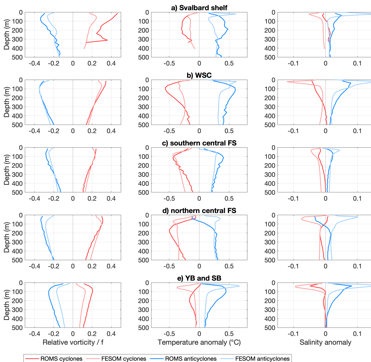
Figure 10. Vertical extent of eddies tracked in 100 m depth during the years 2006–2009 in ROMS (dark colours) and FESOM (light colours) with lifetimes >30 days for cyclones (red) and anticyclones (blue) generated in regions a) Svalbard shelf, b) West Spitsbergen Current, c) southern central Fram Strait, d) northern central Fram Strait and e) Yermak and Svalbard Branch. Left, middle and right panels show relative vorticity, temperature anomaly and salinity anomaly, respectively. Anomalies are calculated by taking the value in the eddy centre relative to the mean value of the month.
