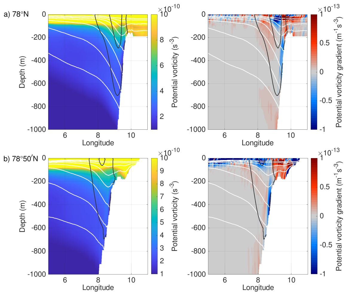
Figure 13. Ertel potential vorticity (left panel) and its gradient in zonal direction (right panel) across Fram Strait at (a) 78^{\circ}\text{N} and (b) 78^{\circ}50'\text{N} computed from long-term mean FESOM data (2006–2009). Black lines show simulated meridional velocity contours (0.1 and 0.2 m/s), and white lines show the simulated 27.9, 28, 28.1, 28.2, and 28.22 \text{kg}/\text{m}^3 isopycnals.
