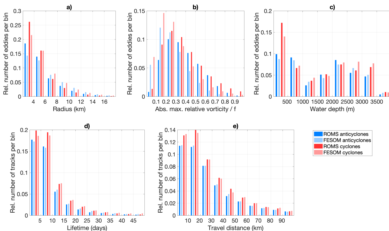
Figure 7. Histogram of (a) radius, (b) maximum relative vorticity normalised by f , (c) water depth, (d) eddy lifetime and (e) travel distance for anticyclonic (blue) and cyclonic eddies (red) normalised by the number of eddies/tracks tracked in the area 8^{\circ}\text{W} – 20^{\circ}\text{E}/76^{\circ}\text{N} – 82^{\circ}\text{N} in the years 2006–2009 in ROMS (dark colours) and FESOM (light colours).
