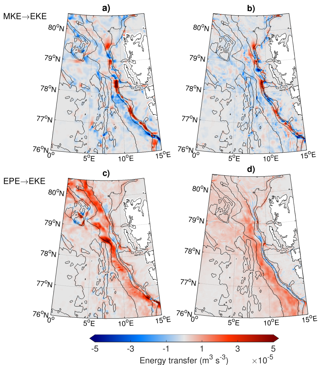
Figure 11. Simulated depth integrated energy transfer from (a,b) mean kinetic to eddy kinetic energy (HRS, product of horizontal Reynolds stress and mean shear, \int_H \left( -\overline{\mathbf{u}'\mathbf{u}'} \cdot \frac{\partial \overline{\mathbf{u}}}{\partial x} - \overline{\mathbf{u}'\mathbf{v}'} \cdot \frac{\partial \overline{\mathbf{u}}}{\partial y} \right) dz ) and (c,d) eddy available potential to eddy kinetic energy (vertical eddy buoyancy flux, \int_H \overline{w'b'} dz ) averaged for 2006–2009 in (a,c) ROMS and (b,d) FESOM. Black contours show bathymetry contours at 1000 m intervals and at 200 m and 500 m depth.
