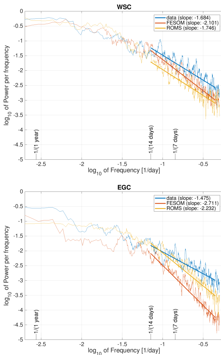
Figure 4. Power density spectra of daily averaged absolute velocity in 75 m depth in the (top) West Spitsbergen Current and (bottom) East Greenland Current from mooring measurements (blue), and models FESOM (red) and ROMS (yellow). Thick lines indicate slopes of the spectra.
