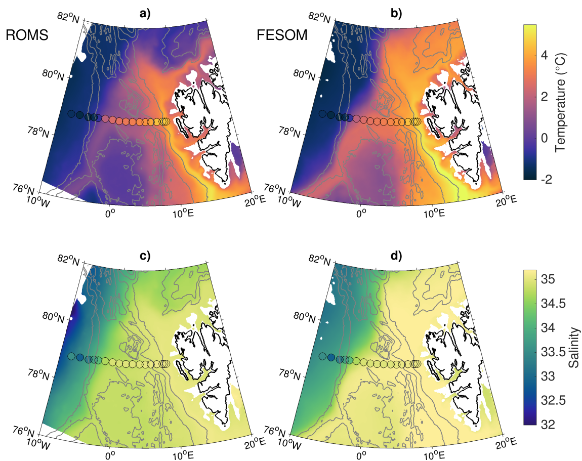
Figure 3. Temperature (a,b) and salinity (c,d) in 100 m depth averaged over the time period 2006–2009 simulated by ROMS (left) and FESOM (right). Dots show mooring measurements in 75 m depth for the same time period (von Appen et al., 2019). Grey contour lines indicate bathymetry at 1000 m intervals.
