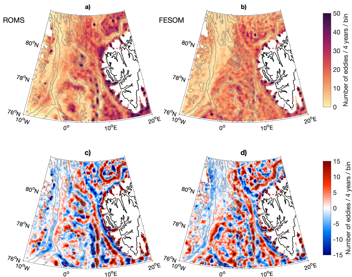
Figure 6. (a,b) Total number of eddy occurrences in the years 2006–2009 for (left) ROMS and (right) FESOM, binned in a 1/24^\circ grid and smoothed with a 3 point Hanning window kernel. (c,d) Difference between cyclonic and anticyclonic eddies (cyclones minus anticyclones).
