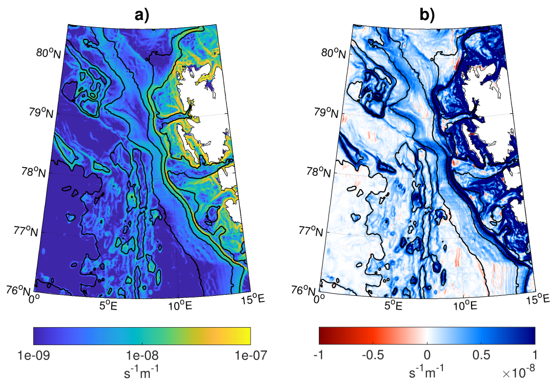
Figure 12. a) Topographic \beta = -\frac{f}{H}\nabla H and b) \beta - \partial_{xx}v , where v is the simulated meridional velocity from FESOM. The second derivative of v is computed from monthly means, and then averaged over the years 2006–2009. A change of sign of \beta - \partial_{xx}v is a necessary condition for barotropic instability. Black contours show bathymetry contours at 1000 m intervals and at 250 m and 500 m depth.
