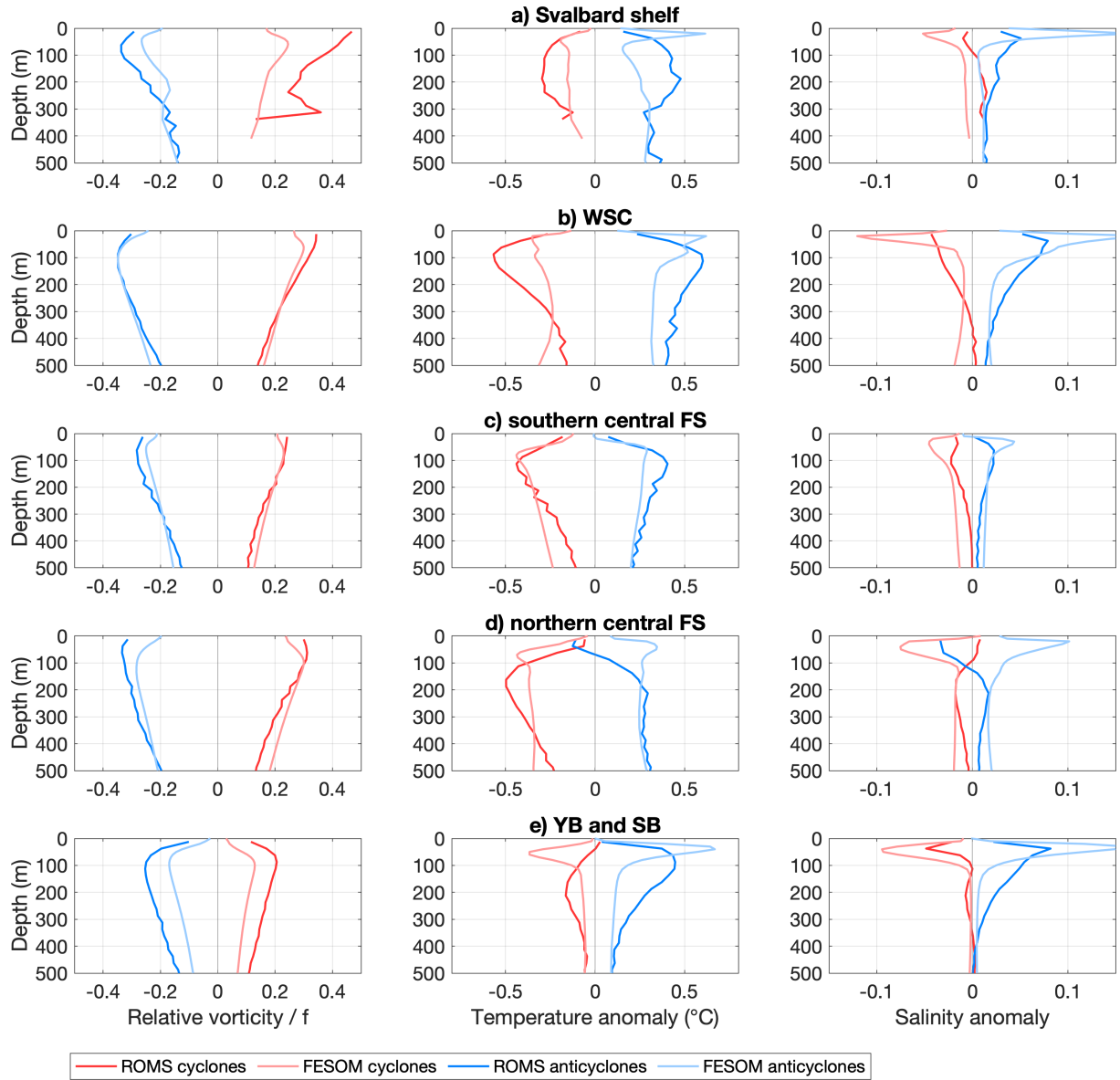
Figure 10. Vertical structure of eddies tracked in 100 m depth during the years 2006–2009 in ROMS (dark colours) and FESOM (light colours) with lifetimes >30 days for cyclones (red) and anticyclones (blue) generated in regions a) Svalbard shelf, b) West Spitsbergen Current, c) southern central Fram Strait, d) northern central Fram Strait and e) Yermak and Svalbard Branch. Left, middle and right panels show relative vorticity, temperature anomaly and salinity anomaly, respectively. Anomalies are calculated by taking the value in the eddy centre relative to the mean value of the month.
