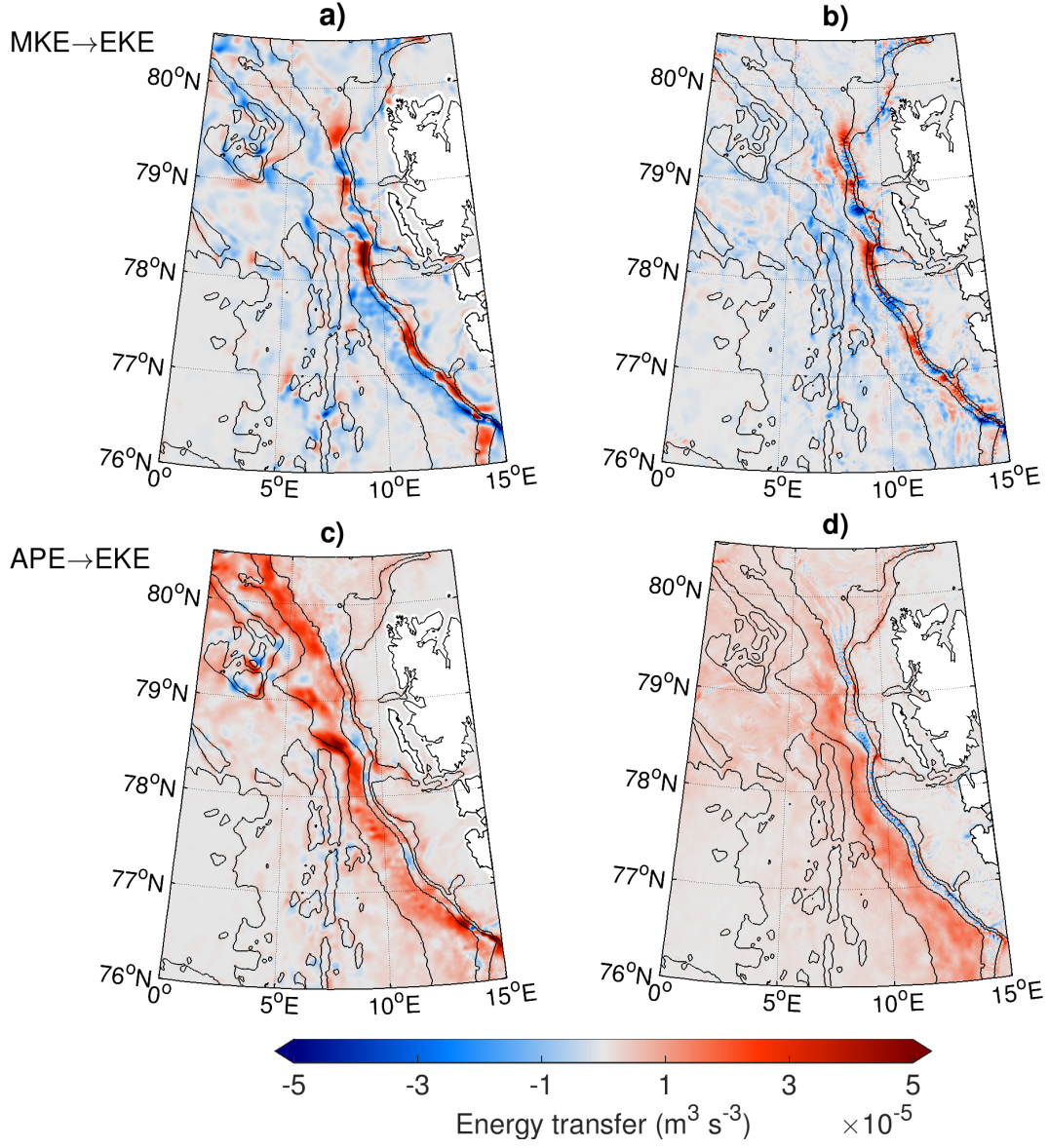
Figure 12. Simulated depth integrated energy transfer from (a,b) mean kinetic to eddy kinetic energy (product of horizontal Reynolds stress and mean shear, \int_H \left( -\overline{\mathbf{u}'\mathbf{u}'} \cdot \frac{\partial \overline{\mathbf{u}}}{\partial x} - \overline{\mathbf{u}'\mathbf{v}'} \cdot \frac{\partial \overline{\mathbf{u}}}{\partial y} \right) dz ) and (c,d) available potential to eddy kinetic energy (vertical eddy buoyancy flux, \int_H \overline{w'b'} dz ) averaged for 2006–2009 in (a,c) ROMS and (b,d) FESOM. Black contours show bathymetry contours at 1000 m intervals and at 200 m and 500 m depth.
