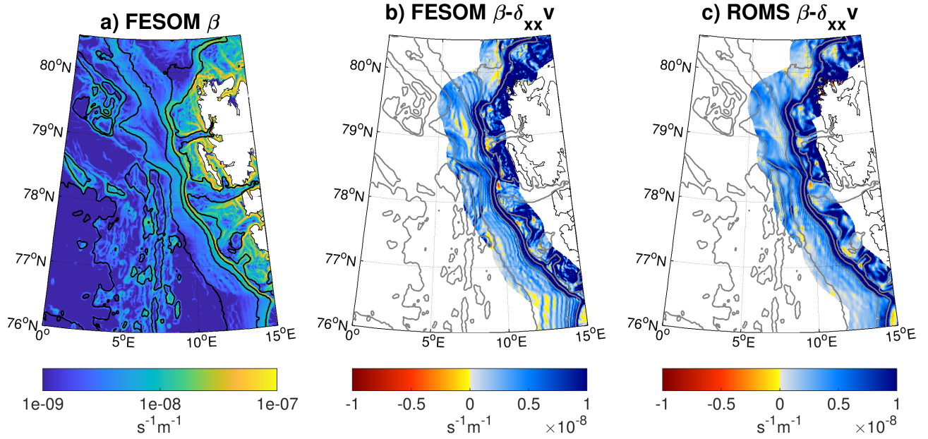
Figure 13. Topographic \beta = -\frac{f}{H} \nabla H computed from FESOM bathymetry (a) and \beta - \partial_{xx} \bar{v} for FESOM (b) and ROMS (c), where \bar{v} is the simulated depth-averaged meridional velocity. The second derivative of \bar{v} is computed from monthly means, and then averaged over the years 2006–2009. A change of sign of \beta - \partial_{xx} \bar{v} is a necessary condition for barotropic instability. Contours show bathymetry at 1000 m intervals and at 200 m and 500 m depth. Note that values in (b) and (c) are only shown in the vicinity of the WSC main pathway (within a distance of 50 km to the 250 m isobath).
