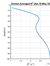
Figure R1. Vertical profile of domain averaged (forced region) buoyancy frequency N^2 ( s^{-2} ) averaged from Apr. 10 to May 10.
