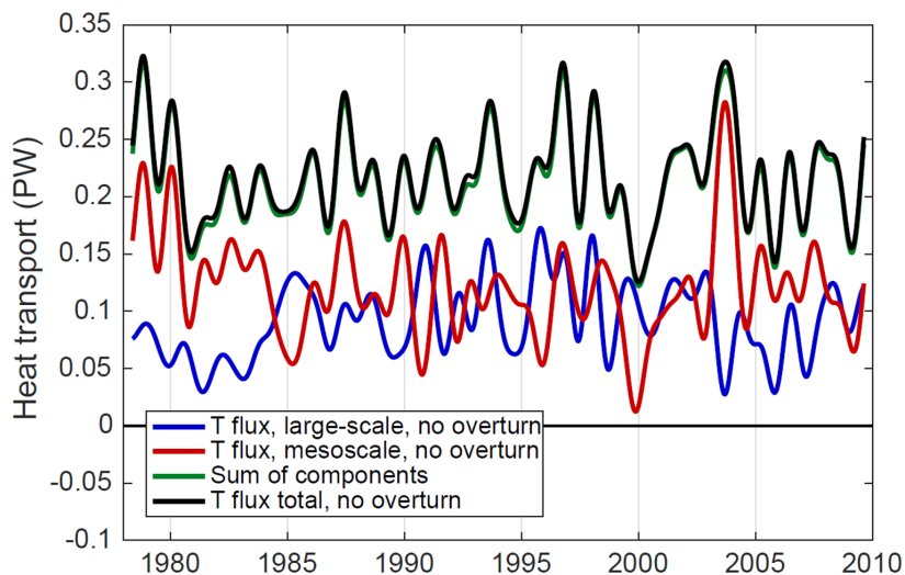
Figure 5. Basin-integrated contributions of large-scale and mesoscale v and T to the ID variability of heat transport across 40^\circ\text{N} in the Atlantic. The zonal means of v and T are removed prior to the computations. The sum of the large-scale and mesoscale components (green) is compared to the total temperature flux minus the overturning contribution (black); differences between the two are due to high-frequency co-variances of v and T at timescales shorter than 5 days.
