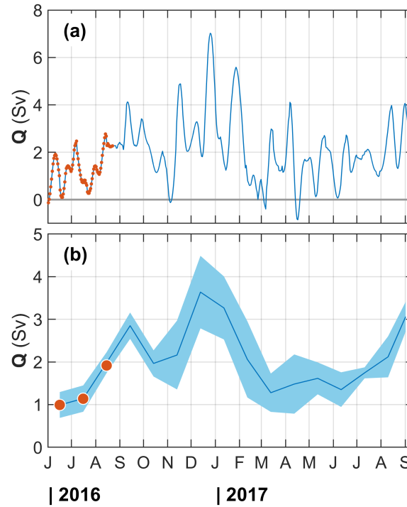
Figure 6. Total AW transport, in the 50–650 m range covered with moorings MN and MW, assigning a width of 12.5 km to MW and 7.6 km to MN (see text for details and sensitivity to choices). AW is defined with \Theta > 5^\circ\text{C} , as measured at MW which has temperature sensors throughout the deployment. MN has temperature record in the first 3 months and the transport calculation using those records (red) agree with MW. a) Daily transports from 14 day low-passed records, b) monthly averages of the transports shown in (a). The envelope is \pm standard error using a decorrelation time scale of 7 days).
