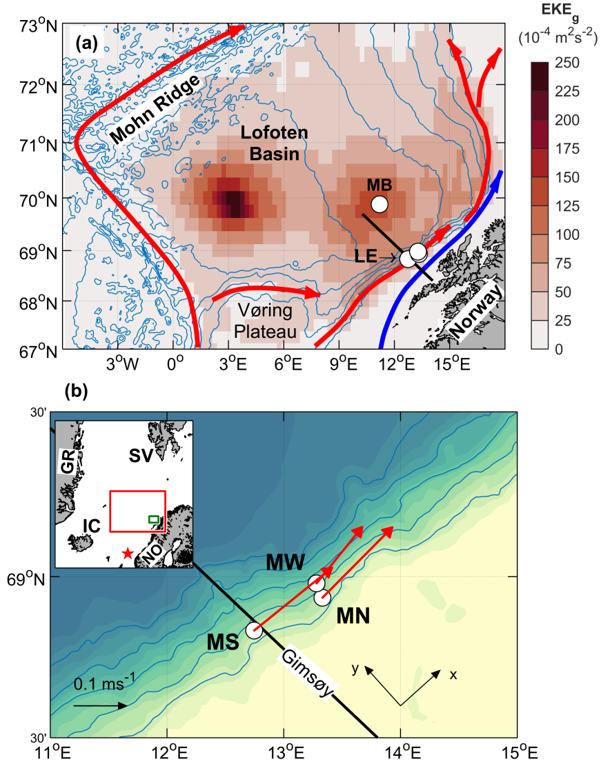
Figure 1. (a) Bathymetry of the Lofoten Basin in the Norwegian Sea (ETOP01, contours at 500 m intervals) and the geostrophic EKE ( EKE_g ) averaged over the period 1993 to 2018, calculated using sea-level anomalies from satellite altimeter observations. General circulation of the warm Atlantic Water is indicated by red arrows showing the slope current and the front current. The Norwegian coastal current is indicated by the blue arrow. Black transect is the portion of Gimsøy section shown in Fig. 2. Mooring positions are shown by circles, also showing the basin mooring (MB) at the secondary EKE_g maximum. Lofoten Escarpment (LE) is the steep slope region near the slope moorings. (b) A zoom-in to the moorings analyzed in this study, showing MS, MN and MW together with 200–600 m depth-averaged current vectors (scale on lower left), Gimsøy section (black), and the orientation of the coordinate system (along-slope, x , and across-slope, y ). Blue isobaths are drawn every 500 m. The inset is a location map with domains of (a) and (b) marked in red and green, respectively. The monitoring location for the Svinøy section is shown by the red star. NO: Norway, SV: Svalbard, IC: Iceland, GR: Greenland.
