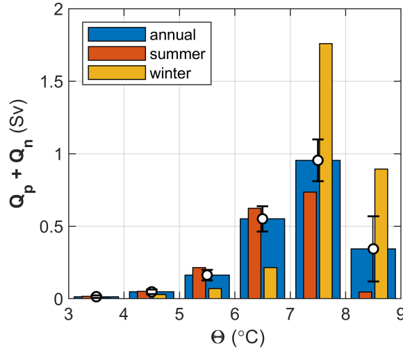
Figure 7. Total net transport ( Q_p + Q_n ) in the 50–650 m depth range, averaged in temperature classes for the entire record (annual), summer (JJA) and winter (DJF) months. Error bars ( \pm standard error) are shown for the annual averages.
