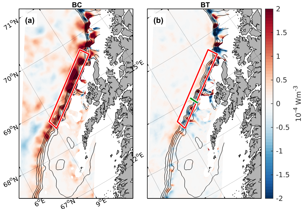
Figure 11. Maps of a) baroclinic and b) barotropic conversion rates averaged over one year (1999) and between 100-1000 m depth or to bottom in shallower areas. Longitudes and latitudes are identical in both panels and are only labelled in (a). The red box is the slope region where volume-averaged conversion rates shown in Fig 12a are computed. The green line across the slope in (b) marks a segment across the mooring positions used for comparison of volume averaged and segment/virtual mooring calculations (see text and Fig 12b). Black contours show the 200, 400, 600, 800 and 1000 m isobaths.
