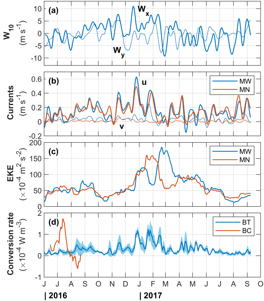
Figure 10. Time series of a) ERA5 wind along-slope ( W_x ) and cross-slope ( W_y ) components, b) 200–600 m averaged u and v measured at mooring MW (blue) and MN (red), c) 200–600 m averaged EKE at MW (blue) and MN (red) and d) barotropic (BT, blue) and baroclinic (BC, red) conversion rates. BC is at 400 m level and only available for 3 months. BT is the depth-average and one standard deviation envelope over calculations at 200, 300, 400, 500 and 600 m. All curves are 30-day moving averages.
