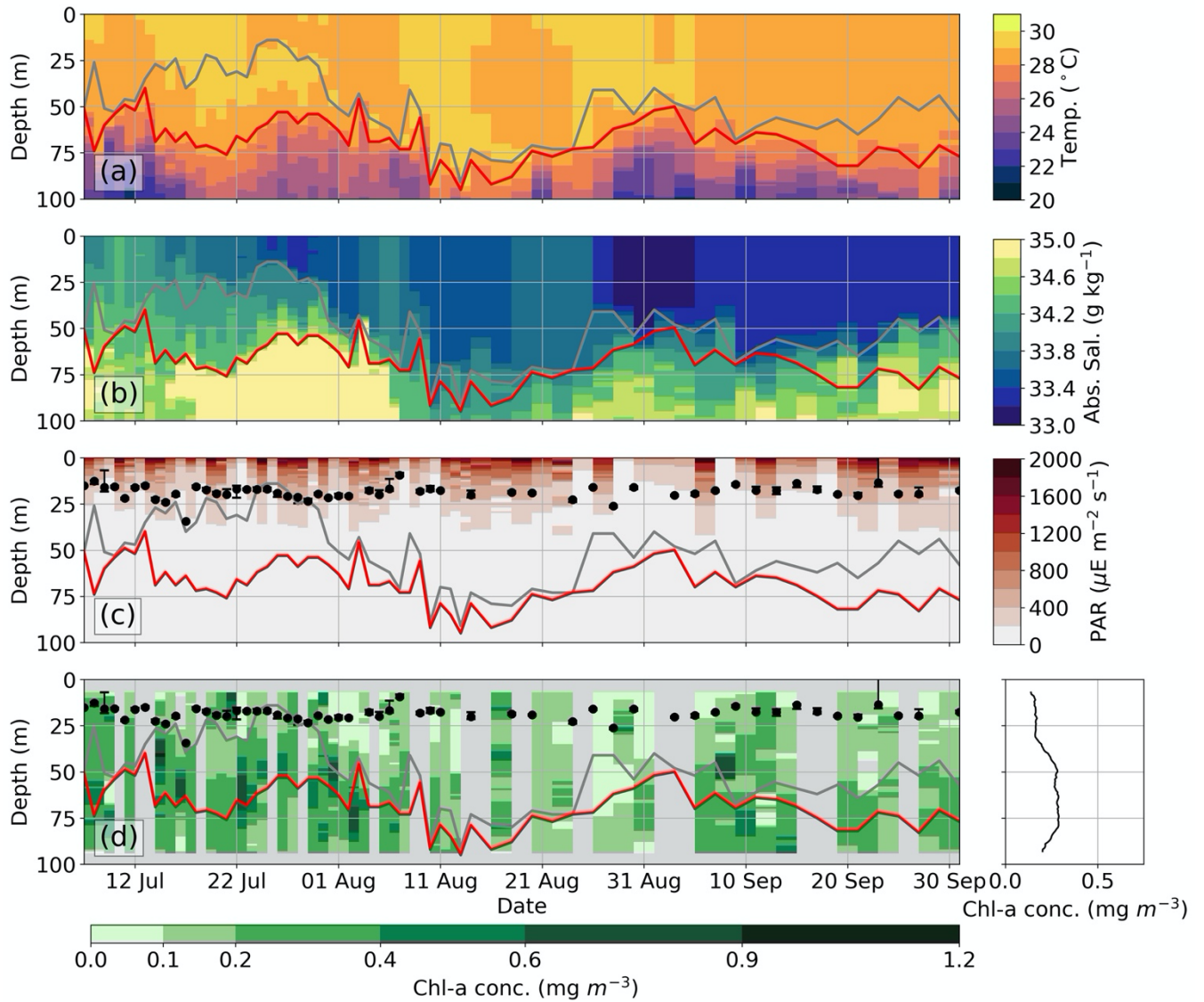
Figure 8: As Fig. 6 but for float 630.
