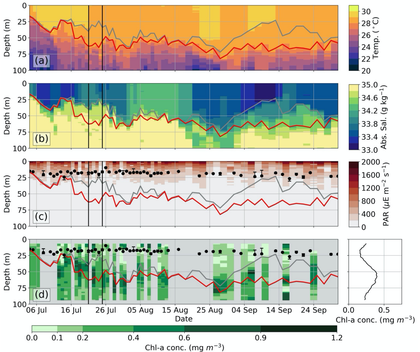
880 Figure 6: Time series of observations measured by float 631, linearly interpolated to 1 m depth intervals: (a) temperature [°C], (b) absolute salinity [g kg -1 ], (c) PAR [ \mu\text{E m}^{-2} \text{s}^{-1} ], (d) chlorophyll concentration and vertical profile of the average chlorophyll concentration [mg m -3 ]. Grey sections in the chlorophyll time series represent removed E_d(490) profiles that displayed excessive noise. The black dots are scale depth values, h_2 [m]. The region between the MLD (grey line) and isothermal layer depth (red line) is the barrier layer.
