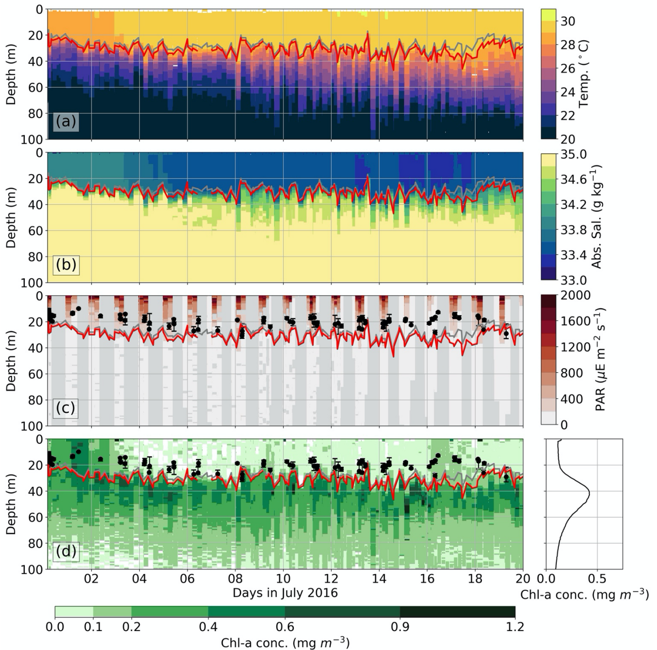
845 Figure 3: Time series of observations measured by glider SG579, linearly interpolated to 1 m depth intervals down to 100 m: (a) temperature [°C], (b) absolute salinity [g kg -1 ], (c) PAR [ \mu\text{E m}^{-2} \text{s}^{-1} ], (d) chlorophyll concentration and vertical profile of the average chlorophyll concentration [mg m -3 ]. The black circles are scale depth values, h_2 [m]. The MLD is defined as the depth where density is same as the surface density plus an increase in density equivalent to a 0.8°C decrease in temperature, and the isothermal layer depth is calculated as the depth where temperature is 0.8°C cooler than SST (Kara et al., 2000; Thushara et al., 2019). The region between the MLD (grey line) and isothermal layer depth (red line) is the barrier layer.
