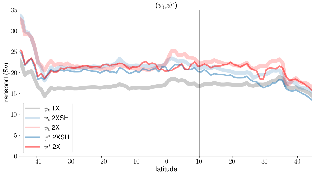
Figure 9. The total maximum overturning streamfunction \psi_t and the maximum overturning streamfunction \psi^* in the case that we hold-use the time-mean vertical velocity shear \frac{\partial^2 \psi}{\partial z^2} constant (of the 1X) reference experiment and the changes in the level of no motion from the 2XSH and 2X experiments to integrate the vertical shear vertically.
