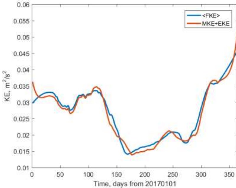
410 Figure 8: Temporal variability of area averaged, time smoothed full kinetic energy (blue); and the sum of eddy and mean kinetic energy (orange) in the surface layer of the Red Sea during 2017.
