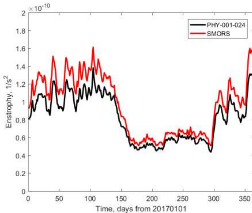
450 Figure 11: Seasonal variability area averaged enstrophy assessed from medium resolution PHY_001_024 (black) and high-resolution SMORS (red) models.
