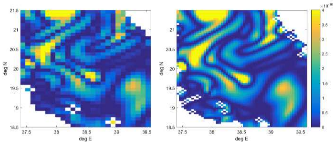
570 Figure 14: Enstrophy of surface currents in the central part of the Red Sea presented by eddy-permitting PHY_000_024 (left) and eddy resolving SMORS (right) model: The white areas represent land and are different as the fine model uses higher resolution bathymetry and coastline, which reveals more small islands.
