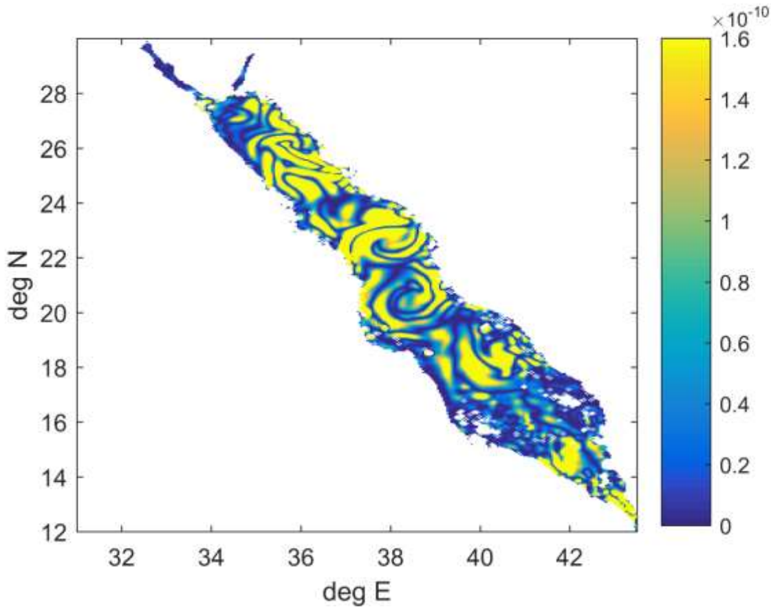
Figure 12: Distribution of local enstrophy of surface currents ( s^{-2} ) in the Red Sea on the 1 st April 2017 estimated from SMORS model output.
