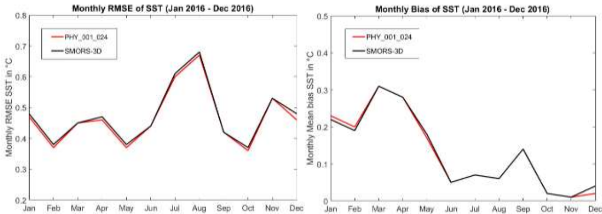
Figure 6: Monthly RMSE and bias comparisons: Monthly RMSE (left panel) and monthly bias (right panel) between PHY_001_024 and OSTIA (red line); and between SMORS and OSTIA (black line).
