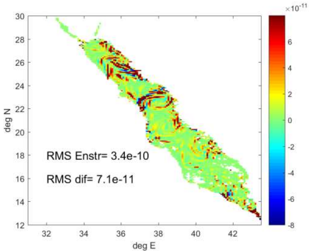
Figure 13: Spatial distribution of differences in surface enstrophy ( s^{-2} ) between the high-resolution and medium-resolution models on the 1 st of April of 2017.
