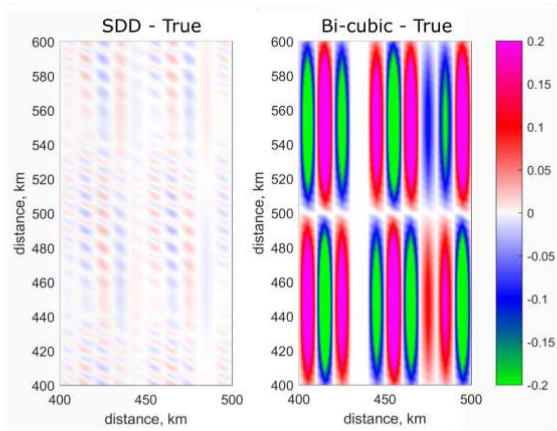
195 Figure 3: Comparison of skill between SDD and bi-cubic interpolation: Left: map of differences of parameter F values between SDD model and the true solution. Right: map of differences of parameter F values between bi-cubic interpolation and the true solution. The colour bar limits are chosen to be between -0.2 and 0.2 so the differences for SDD are visible, however, the maximum differences for the bi-cubic model are in fact between -0.4 and 0.4 .
