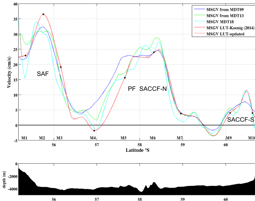
490 Figure 19: Mean surface geostrophic velocities (MSGV) derived from MDTCNES-CLS09 (blue), from MDTCNES-CLS13 (green), MDTCNES-CLS18 (cyan) and LUT (red) along Jason track #104. Location of the Drake moorings are indicated M1 to M10. Below bathymetry along the section.
