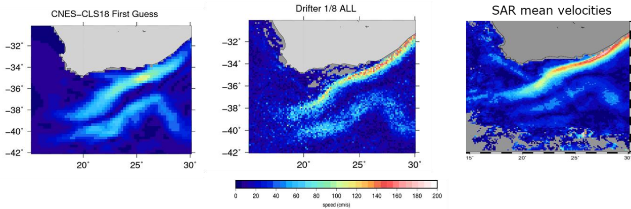
430 Figure 14: Mean velocities in the Agulhas Current area from (left) the GOCE-only derived MDT First Guess, (middle) drifting buoy velocities and (right) SAR derived mean velocities
