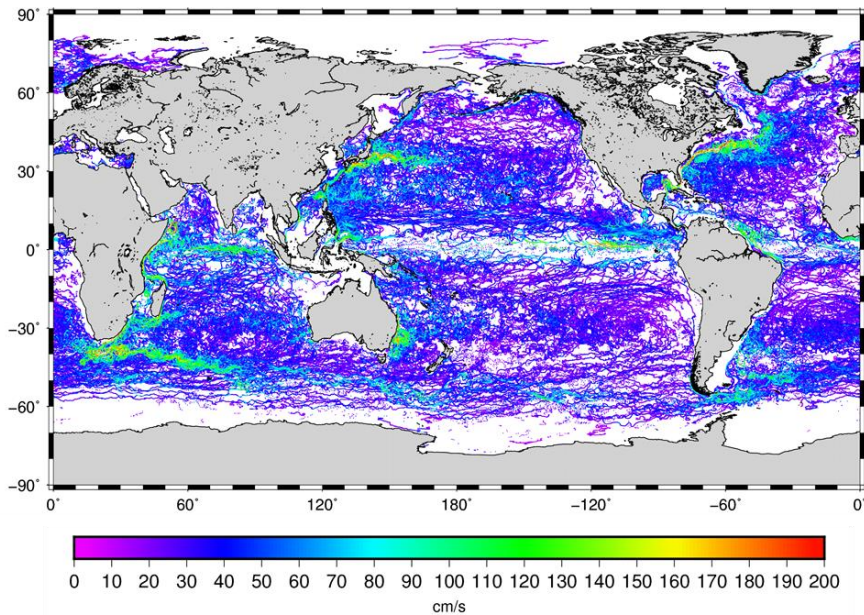
505 Figure 20: Trajectories of the 15m drogued SVP drifters available over year 2017. Colors give the speed velocities deduced along the drifter trajectories.
