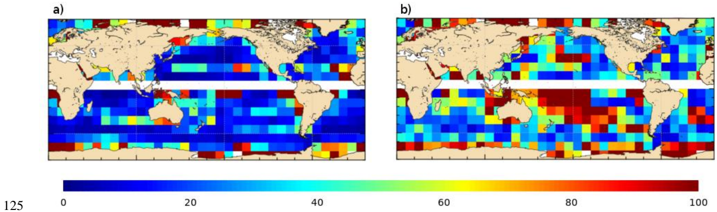
Figure 1: Root Mean Square differences between (a) zonal and (b) meridional mean geostrophic drifter velocities and the MDT CNES-CLS18 first guess geostrophic velocities in percentage of drifter variance (%) in 5^\circ \times 5^\circ boxes
