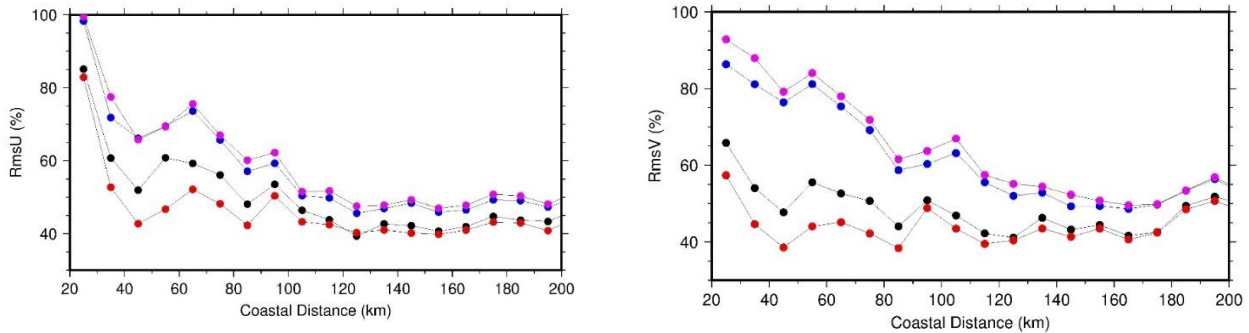
520 Figure 21: Zonal (left) and Meridional (right) RMS differences as a function of coastal distance between the independent drifting buoy velocities and the altimeter geostrophic velocities obtained using different MDT solutions: Pink the CNES-CLS13 MDT first guess; Blue the CNES-CLS18 MDT First Guess; Black the CNES-CLS13 MDT and Red the CNES-CLS18 MDT
