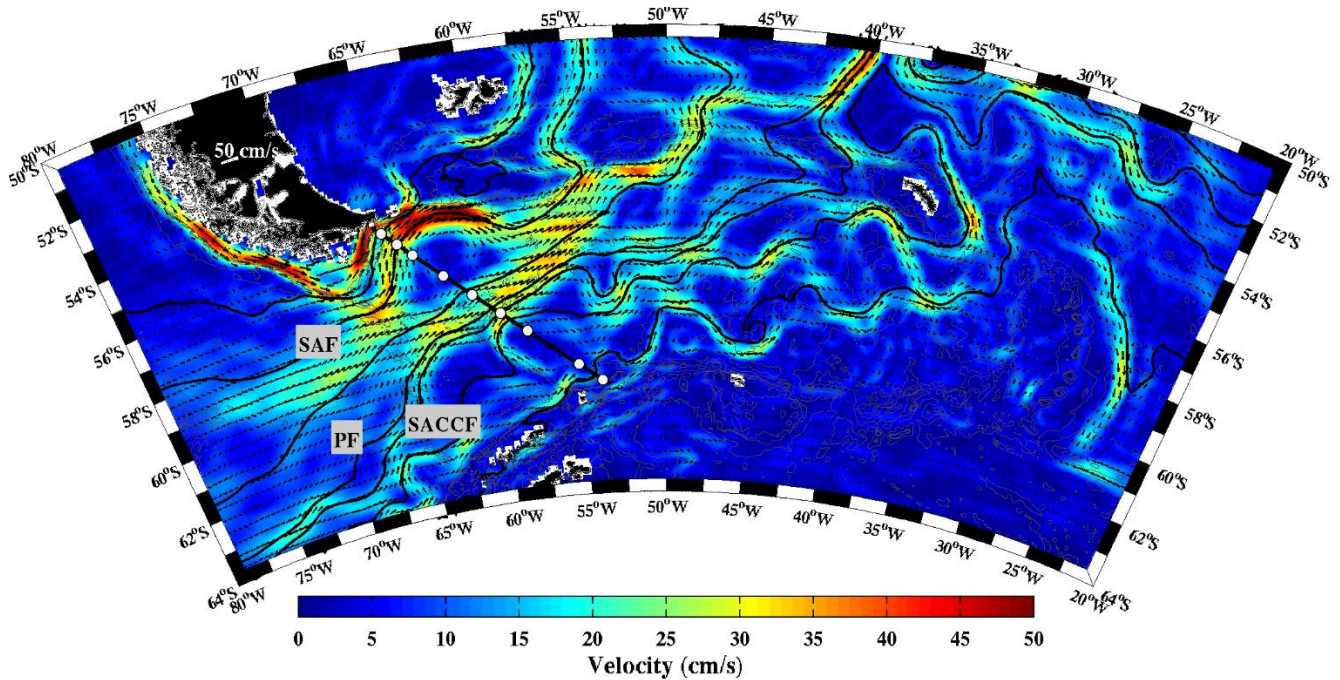
495 Figure 18: Mean surface velocity magnitude (in cm/s) and mean surface velocity vectors from MDT CNES-CLS18. Black lines are isolines of mean sea surface height corresponding to the main Antarctic Circumpolar Current (ACC) fronts and their branches: SAF-N (23 cm), SAF-M (0 cm), PF-N (43 cm), PF-M (-70 cm), PF-S (-79 cm), SACCF-N (-93 cm) and SACCF-S (-114 cm). White dots indicate the position of the DRAKE moorings.
