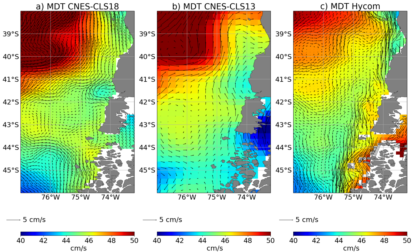
410 Figure 13: MDT and associated mean geostrophic current along the south Chilean coast from the MDT CNES-CLS13, MDT CNES-CLS18 and the numerical model HYCOM interpolated on the MDT CNES-CLS18 grid (1/8°)
