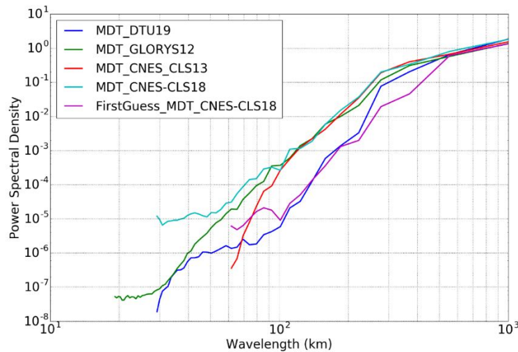
Figure 7: Meridional Spectral Power Density obtained for different MDT solutions in a 10^\circ box centered around (43^\circ\text{E}, 49^\circ\text{S})
