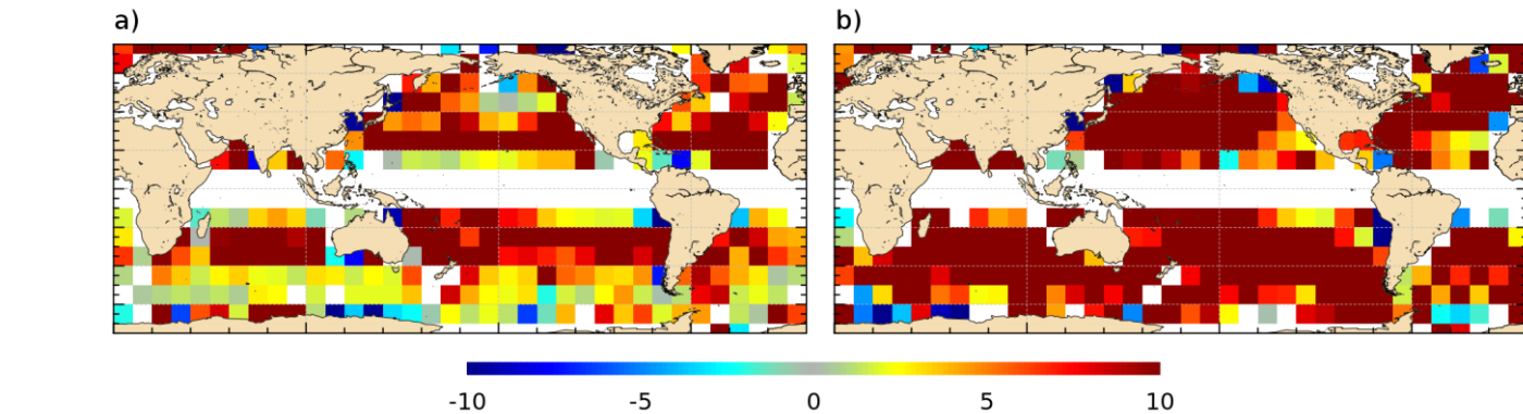
Figure 2: Difference (cm/s) of the RMSD obtained using the first guess of MDT CNES-CLS13 and the first guess of MDT CNES-CLS18 for the (a) zonal and (b) meridional components in 5^\circ \times 5^\circ boxes. Only boxes with more than 500 points and where difference is statistically significant at more than 95% (T-test) are shown. The reddish color underline improvement while bluish stand for degradation (see text for more detail)
