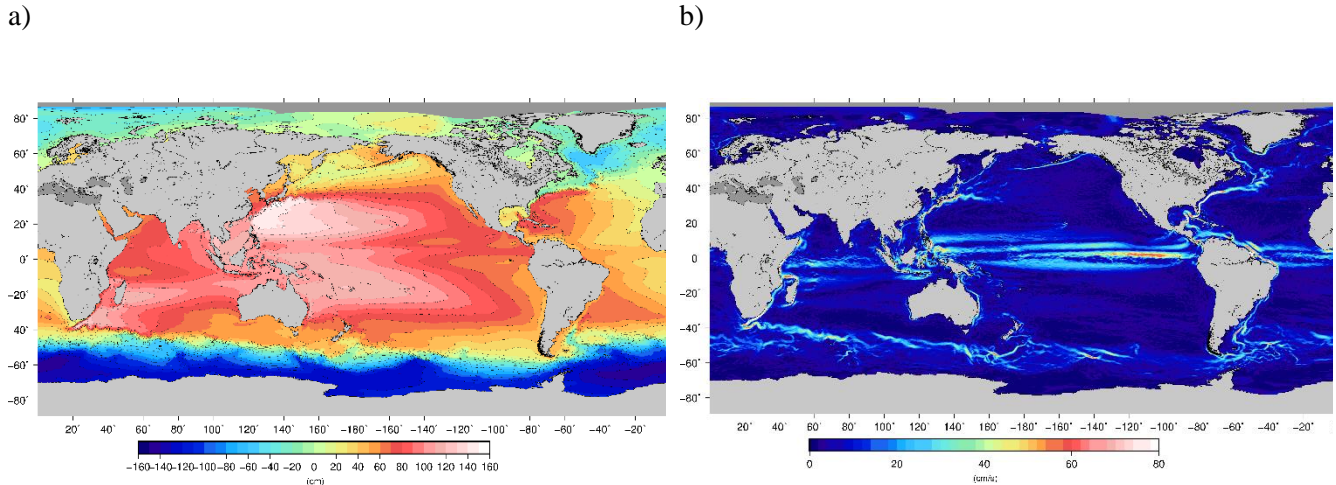
Figure 6: (a) The CNES-CLS18 Mean Dynamic Topography (cm) and (b) intensity of their associated mean geostrophic velocities (cm/s)
