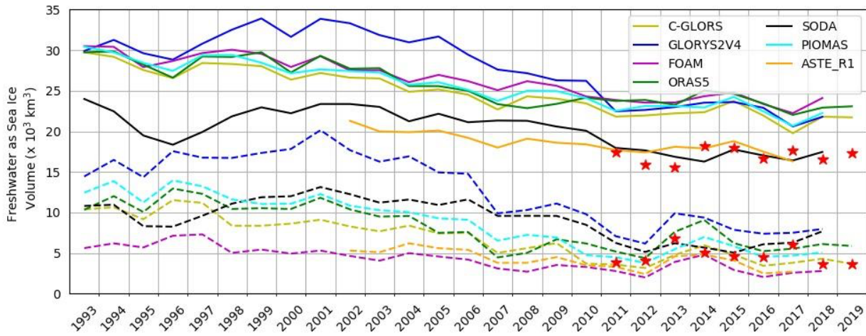
360 Figure 5: Time series of annual freshwater volume stored as sea ice from 7 ORAs and CRYOSAT2 (red stars), (in 10^3 \text{km}^3 ). The sea ice volume is calculated as the product of sea ice area and thickness. Annual volume maxima are shown by bold lines, while annual minima are shown by dashed lines.
