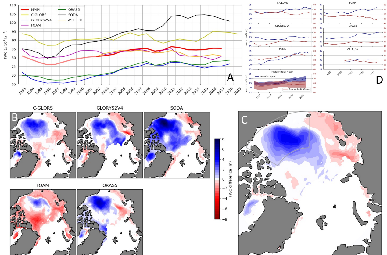
160 Figure 2: Ordered counter-clockwise: A) Time series of annual freshwater content integrated from 70-90°N and down to the 34 isohaline for the period 1993-2019 from 6 ORAs (in 10^3 \text{ km}^3 ). Multi-model mean shown in red, darker red indicates all 6 ORAs included. B) Difference (in m) between 2010-2017 and 2000-2010 means in 5 ORAs (not including ASTE_R1). C) Multi-model mean of differences (in m) shown in (B). D) Annual freshwater content separated into contributions from Beaufort Gyre (blue) and the rest of the Arctic Ocean (red). Lower right figure shows the multi-model mean with \pm 1 standard deviation shown with shading. The Beaufort Gyre is defined as 70-80°N, 120-180°W to be consistent with the satellite estimates below.
