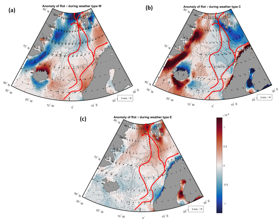
Fig. 5. Figure 8. Anomalies of the wind stress curl
