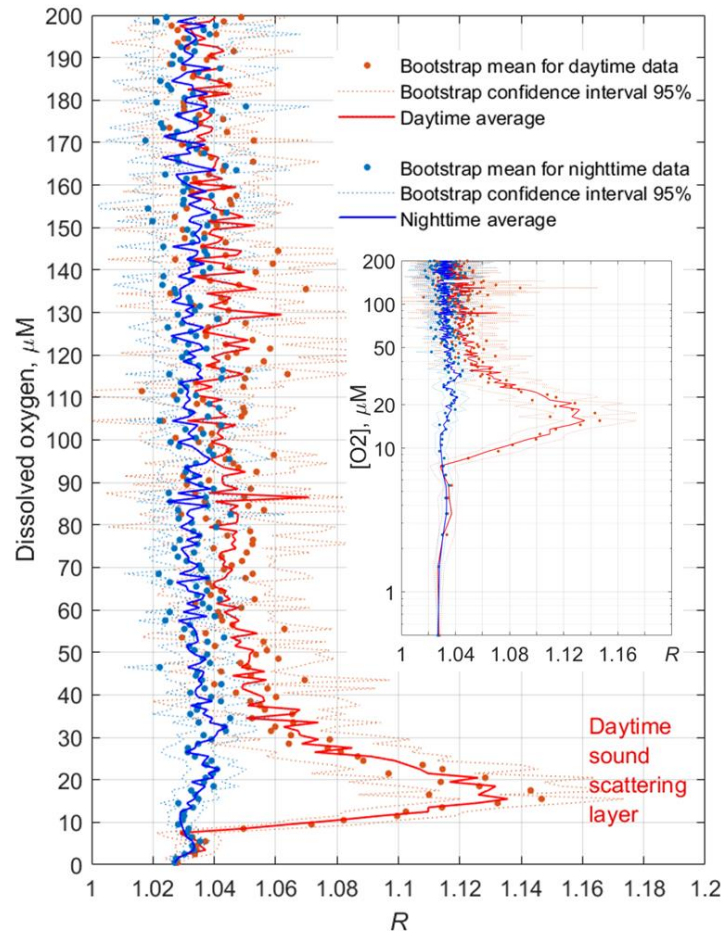
Figure 13: Example profiles of the daytime and nighttime averages \langle R([O_2]) \rangle in November 2019. The inset shows the same plots with the Y-axis drawn logarithmically to reflect the lower parts of the profiles (the hypoxic zone) in more detail.
