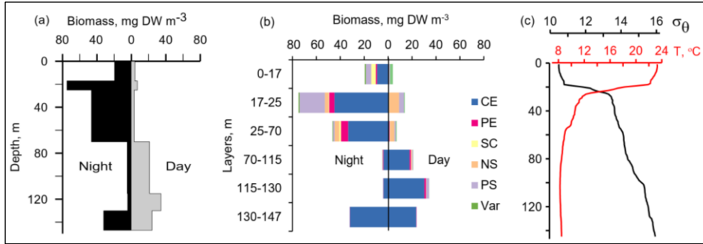
Figure 10: The day/night vertical distribution of (a) total mesozooplankton biomass, (b) zooplankton composition, (c) temperature ( T ) and density ( \sigma_{\theta} ) near the mooring site on July 1 (13:30-14:30) and July 2 (02:30-03:30) of 2014. Temperature and density profiles (c) indicate the selection of sampling strata. CE – Calanus euxinus ; PE – Pseudocalanus elongatus ; SC – small crustaceans; NS – Noctiluca scintillans ; PE – Parasagitta setosa ; Var – varia.
