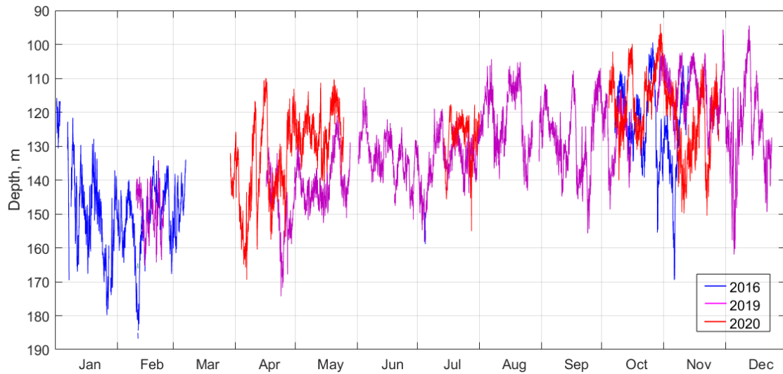
Figure 15: The suboxic boundary depth ( [O_2] = 10 \mu\text{M} ) as observed by the moored profiler in 2016, 2019, 2020.
