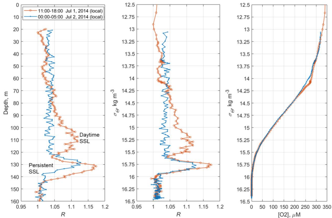
Figure 11: Left - The depth profile of R for the daytime of July 1, 2014, and the nighttime of July 2, 2014, when net sampling (Fig. 11) took place. Middle – the daytime and nighttime averages R versus the specific density, \sigma_{\rho} . Right – Distribution of the daytime and nighttime averages of the dissolved oxygen versus \sigma_{\rho} .
