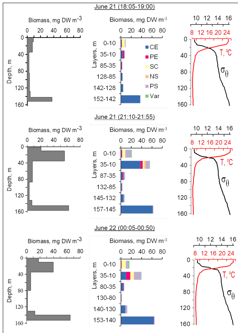
245 Figure 4: The diel changes in vertical distributions of (left) total mesozooplankton biomass, (middle) zooplankton composition, (right) temperature ( T ) and density ( \sigma_{\theta} ) near the mooring site on June 21-22, 2010. The temperature and density profiles were used for the selection of sampling strata. CE – Calanus euxinus ; PE – Pseudocalanus elongatus ; SC – small crustaceans; NS – Noctiluca scintillans ; PE – Parasagitta setosa ; Var – varia.
