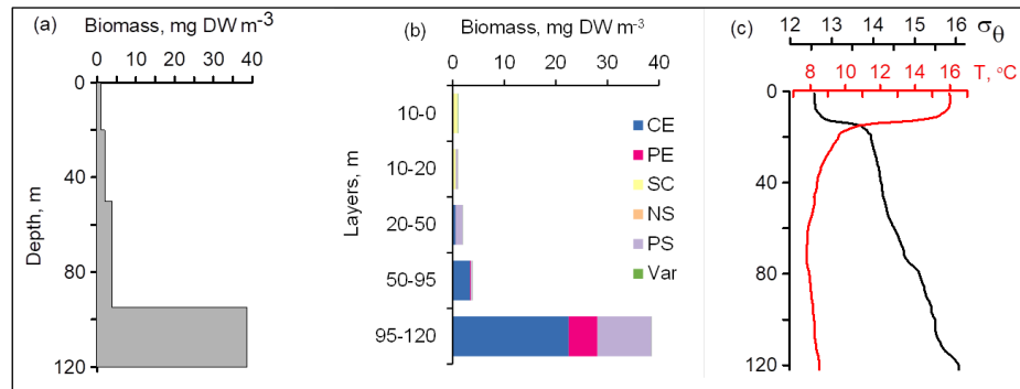
285 Figure 6: The daytime vertical distributions of (a) total mesozooplankton biomass, (b) zooplankton composition, (c) temperature ( T ) and density ( \sigma_\theta ) near the mooring site at 12:30-13:20 on October 6, 2013. Temperature and density profiles (c) indicate the selection of sampling strata. CE – Calanus euxinus ; PE – Pseudocalanus elongatus ; SC – small crustaceans; NS – Noctiluca scintillans ; PE – Parasagitta setosa ; Var – varia.
