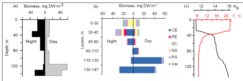
315 Figure 8: Day/night vertical distribution of (a) total mesozooplankton biomass, (b) zooplankton composition, (c) temperature ( T , °C) and density ( \sigma_\theta ) near the mooring site on October 4-5, 2016. Temperature and density profiles (c) indicate the selection of sampling strata. CE – Calanus euxinus ; PE – Pseudocalanus elongatus ; SC – small crustaceans; NS – Noctiluca scintillans ; PE – Parasagitta setosa ; Var – varia.
