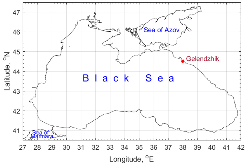
190 Figure 2: The Black Sea coastline ( http://openstreetmapdata.com/data/coastlines ). The observational site off Gelendzhik is shown by a red dot. © OpenStreetMap contributors 2020. Distributed under a Creative Commons BY-SA License.
