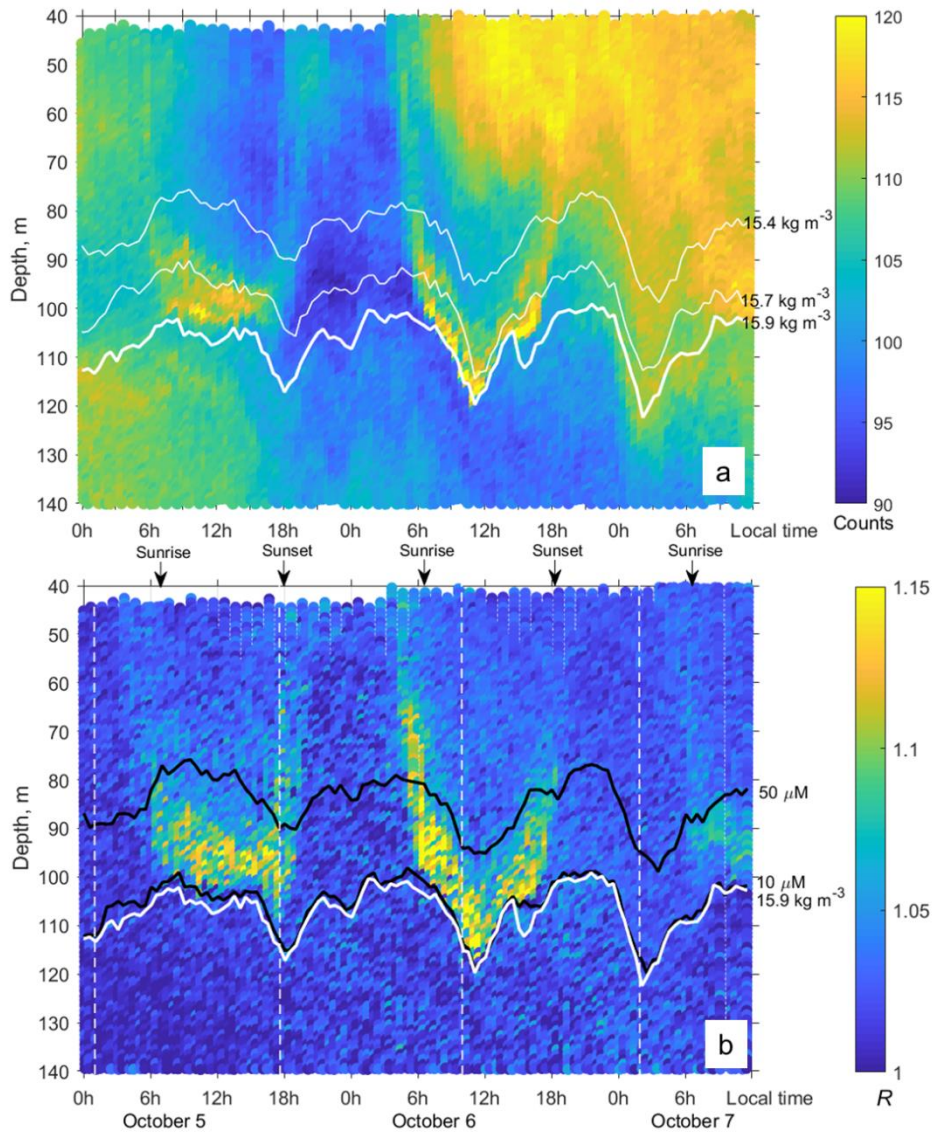
270 Figure 5: a - The time-depth graph of the Aquadopp horizontal-beam (A_1 + A_2)/2 echogram showing acoustic backscatter intensity (counts) on October 5-7, 2013. The Aqualog profiler with the Aquadopp instrument performed ascending/descending cycles every 1 h. The upper, middle and lower white lines are for isopycnals \sigma_\theta 15.4, 15.7 and 15.9, respectively. b - Time-depth scatterplot of the Aquadopp directional acoustic backscatter ratio R = (A_1 + A_2)/2A_3 . Colored lines show [O_2] = 50 \mu\text{M} (upper black line); [O_2] = 10 \mu\text{M} (lower black line); and \sigma_\theta = 15.9 \text{ kg m}^{-3} (white line), which can be taken as a proxy for the boundary of the oxygen zone in the NE Black Sea (Glazer et al., 2006, Ostrovskii, Zatsepin, 2016). Vertical dotted white lines indicate a 17.3 h time interval, which is equal to the period of inertial oscillations at the latitude of the observation. They approximately coincide with troughs of inertial waves.
