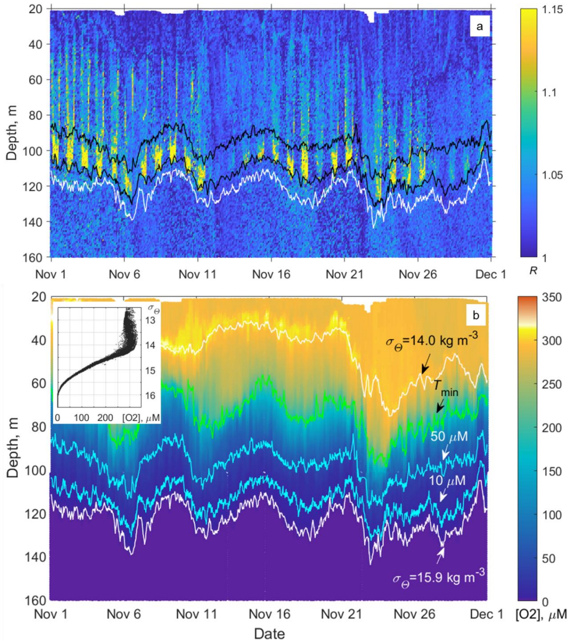
365 Figure 12: a – Example of the monthly long time series of the vertical profiles of the directional acoustic backscatter ratio R for for November 2019 (in total 960 profiles from the moored profiler survey). The upper and lower black lines are iso-oxyline of 50 and 10 \mu\text{M} , respectively. The white line indicates isopycnal \sigma_\theta = 15.9 . b – Evolution of the dissolved oxygen at the profiler mooring site in November 2019. The colored lines indicate the following: the depths of the isopycnals \sigma_\theta = 14 and 15.9 (top and bottom white lines); the depth of the temperature minimum (green line); and [\text{O}_2] = 50 and 10 \mu\text{M} (blue lines). The inset shows the diagram of 370 the dissolved oxygen versus the potential density, [\text{O}_2] - \sigma_\theta , plotted from the moored profiler data of November 2019. In this example, as well as for other observational periods, the dissolved oxygen deviates very little from isopycnal surfaces in the lower part of the oxycline where [\text{O}_2] < 200 \mu\text{M} .
