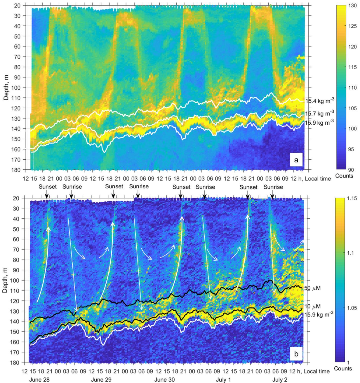
Figure 9: a — The time-depth graph of the Aquadopp horizontal-beam echo (A1 + A2)/2 during the moored profiler survey on June 28–July 2, 2014. The isopycnals are superimposed near the SSLs. b - The graph of time-depth variation in R based on the measurements of sound backscattering. The upper and lower black lines are iso-oxyline of 50 and 10 \mu\text{M} , respectively. The white line indicates isopycnal \sigma_\theta = 15.9 . There is a persistent SSL under iso-oxyline [\text{O}_2] = 10 \mu\text{M} . Thin white arrows schematically show the diel migration of mesozooplankton. The maximum depth of the diel vertical migration is 120–150 m, although some specimens dive to depths of only 80–100 m. The slope of the straight arrow pointing downwards corresponds to a diving speed of \sim 1.5 \text{ cm s}^{-1} . The ascent is accelerated and reaches values of approximately 2.5 \text{ cm s}^{-1} in the upper 60 m depth.
