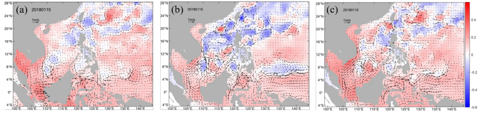
Fig. 2. Figure 12-Daily averaged SLA on January 15, 2018, from AVISO, SCSOFSv1.3, and SCSOFSv2, respectively
