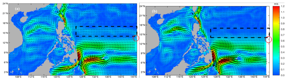
Fig. 1. Figure2 with enlarging the domain to include SCS
