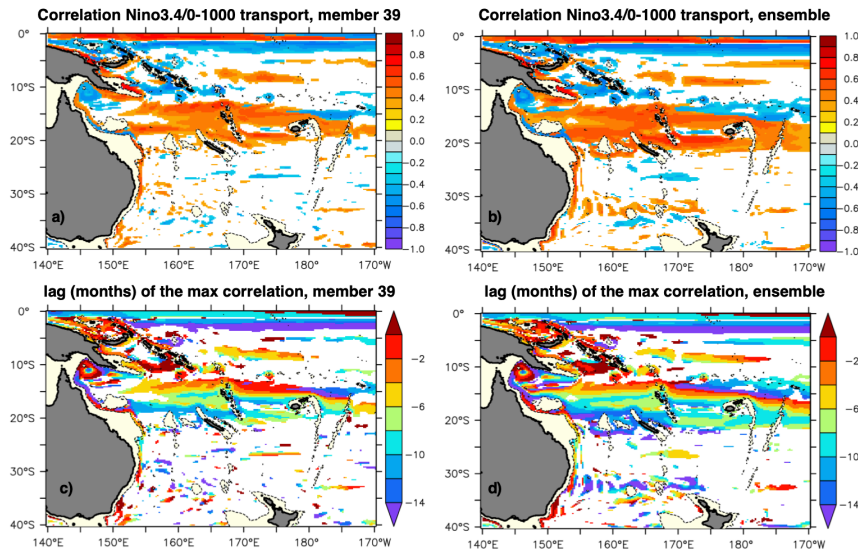
Figure 7: Maximum lagged correlation (a, b) and corresponding lag in months (taken between -15 and 5 months) (c, d) between Nino3.4 index and the 0-1000m interannual transport variations for (a, c): member 39 of the ensemble, and (b, d) the ensemble mean. A negative lag means that Nino3.4 lead the transports variations. Only significant correlations are plotted.
