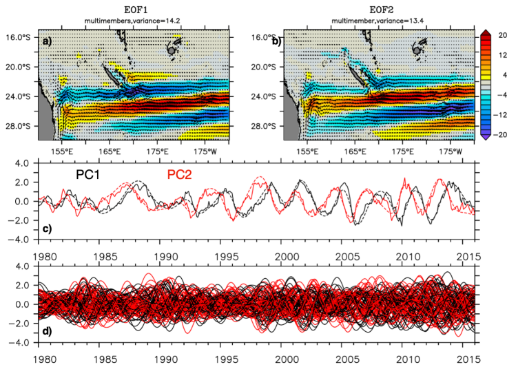
Figure 11: First (a) and second (b) spatial EOFs in the STCC region (15°S-30°S, 150°E-170°W) of the 50 members deviations from the ensemble mean of zonal and meridional transports, considered as a single time series. (c) PCs of the first (black) and second (red) mode, from monthly chaotic transports in thin lines, and interannual chaotic transports in dashed line. (d) The 50 first (black) and second (red) PCs from the 50 chaotic members interannual transports.
