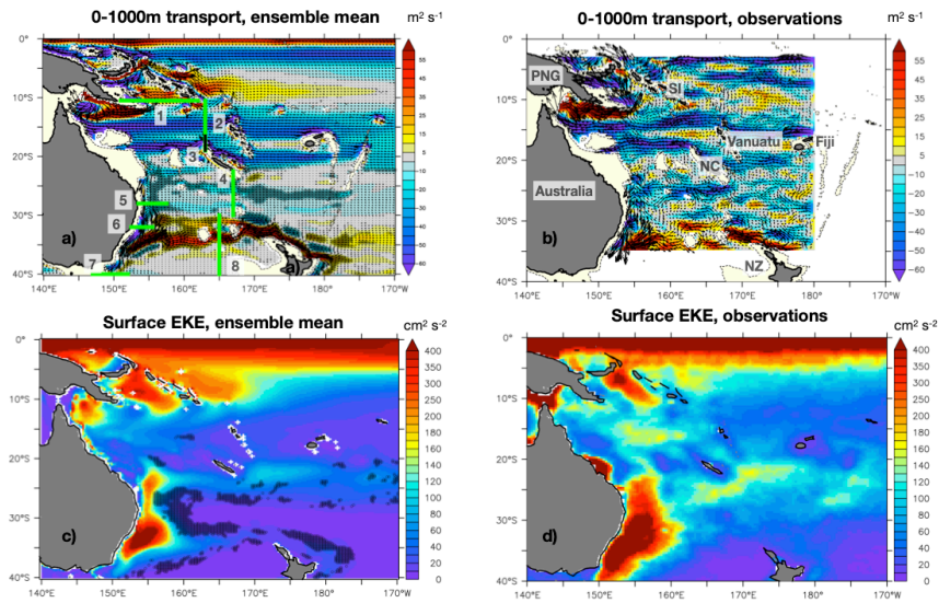
Figure 2: a) 1980-2015 time averaged 0-1000m transport from the ensemble mean. Colors show zonal transport (positive values mean eastward, negative values westward), and arrows total transport. The hatched areas show regions where the spread of these 1980-2015 time averaged 0-1000m transport are at least 15% of the ensemble mean. The green thick lines (and the black thick line) show the main current sections shown in Figure 4, with the associated numbers corresponding to the caption of Figure 4. b) 0-1000m transport from the Argo-Merged observations; colors show zonal transport. The names of the main islands are also indicated. NC: New Caledonia; NZ: New Zealand; SI: Solomon Islands and PNG: Papua New Guinea. c) Time averaged ensemble mean of the 1980-2015 surface EKE. The hatched areas show regions where the spread of these 1980-2015 time EKE are between 10% and 20% of the ensemble mean d) 1993-2015 time averaged surface EKE from OSCAR product.
