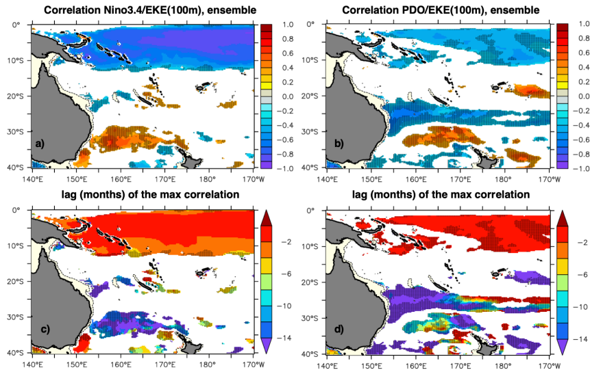
Figure 8: Maximum lagged correlation (a) and corresponding lag in months (taken between -18 and 0 months) (c) between Nino3.4 index and the 100m-EKE interannual variations for the ensemble. Only significant correlations are plotted. A negative lag means that Nino3.4 lead the EKE variations. (b, d): same as (a, c) for the PDO index. In all panels, the hatched areas show regions where the same maximum lagged correlation for 100m-EKE interannual variations in one member picked randomly (member 39) are not significant.
