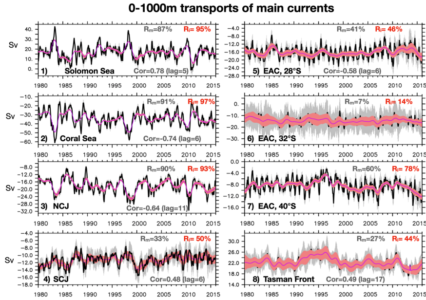
Figure 4: Time series of the 0-1000m integrated transports across various sections (in Sv). In black: monthly values from the ensemble mean; in grey shades, ensemble mean plus or minus the monthly ensemble spread. In red: interannual values from the ensemble mean, and the red shades, ensemble mean plus or minus the interannual ensemble spread. The percentage of the deterministic variance is given as R m for the monthly values and R i for the interannual values. The maximum correlation of the transport with the Nino3.4 index is also given, with the associated lag in months. 1) meridional transport through the entrance of the Solomon Sea (positive is northward) 2) zonal transport through the entrance of the Coral Sea (positive is eastward) 3) westward transport of the NCJ 4) westward transport of the SCJ 5) meridional total transport of the EAC at 28°S (see section 2.3 for definition). R m and R i for the southward only meridional transport are 44% and 58%, respectively. R m and R i for the northward recirculation branch are 21% and 50%, respectively. 6) meridional total transport of the EAC at 32°S. R m and R i for the southward only meridional transport are 10% and 29%, respectively. R m and R i for the northward recirculation branch are 6% and 22%, respectively. 7) meridional transport of the EAC at 40°S. 8) Zonal transport of the Tasman front. See text for details.
