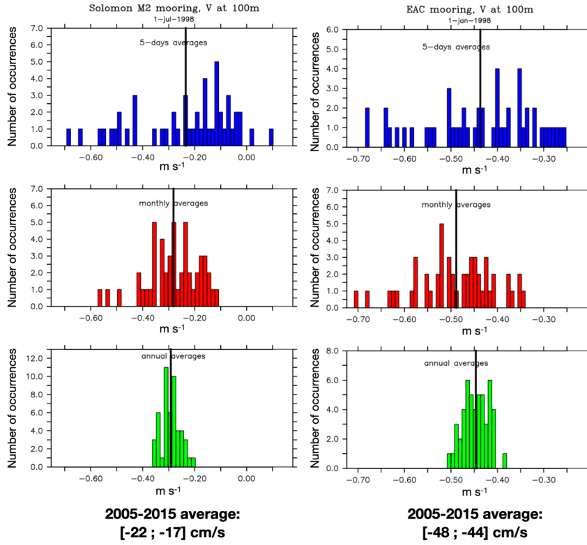
Figure 12: Histograms of velocity among the 50 members, for the meridional velocity at 100m from 5-days average values in blue (a,d), monthly averages in red (b,e) and annual averages in green (c,f), at two locations around a particular date (on 1 July 1998 inside the Solomon Strait, at 154.2°E, 5.36°S (a,b,c) and on 1 January 1998 in the EAC, at 154°E, 27.06°S (d,e,f)). The value of the ensemble mean is also plotted in black lines.
