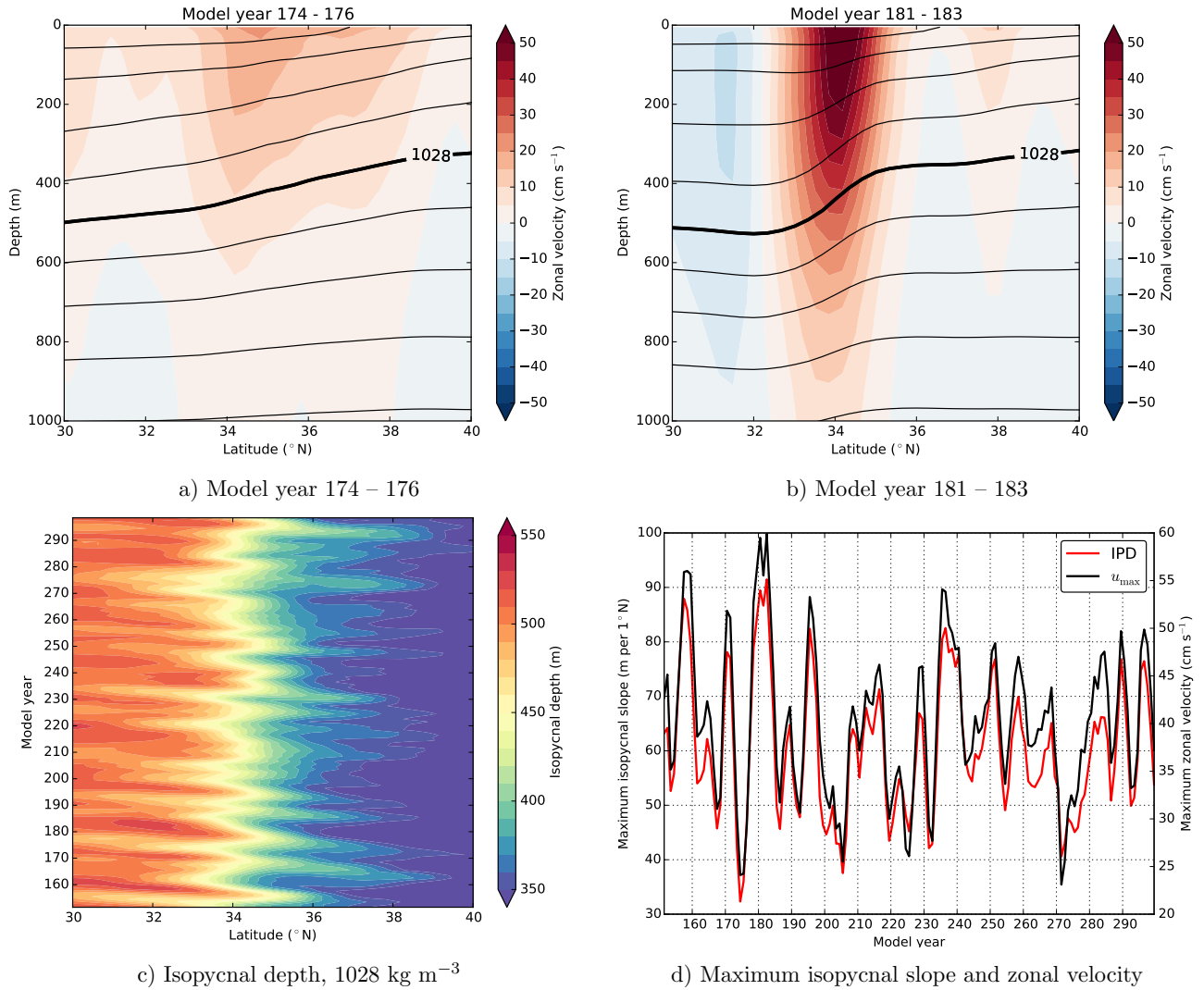
Figure 6. (a & b): The zonally averaged ( 140^{\circ}\text{E} - 160^{\circ}\text{E} ) zonal velocity with depth, averaged in time (3-year average) for a) model years 174 – 176 and b) model years 181 – 183. The black curves are isopycnals each spaced by 1 \text{ kg m}^{-3} and for reference the 1028 \text{ kg m}^{-3} isopycnal is indicated. (c): Hovmöller diagram for the evolution of the 1028 \text{ kg m}^{-3} isopycnal depth, smoothed by a running mean of 36 months. (d): Time series of the maximum slope of the 1028 \text{ kg m}^{-3} isopycnal and the maximum zonal velocity at the maximum slope latitude. The time series are smoothed by a running mean of 36 months.
