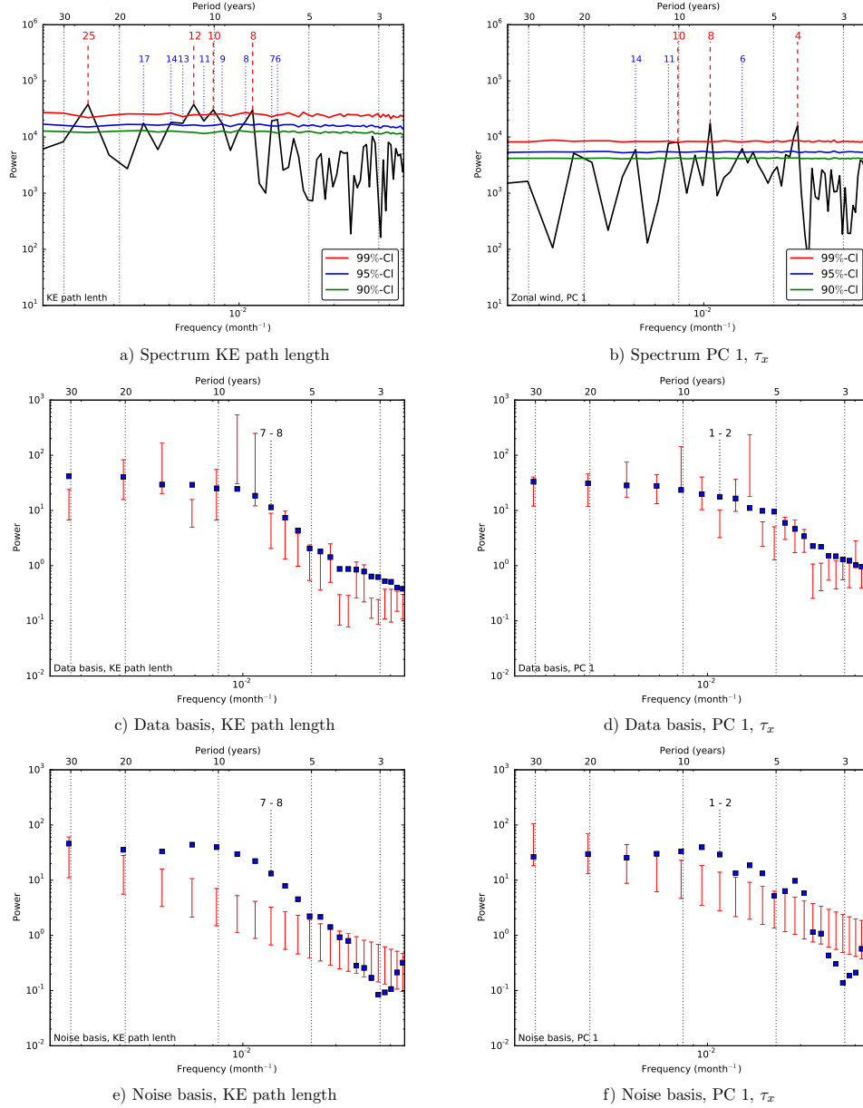
Figure 3. (a & b): Fourier spectrum (black curve) of the KE path length and the first PC of the zonal wind stress (obtained from the projection of the EOF pattern). The colour-coded curves are the significance levels of red-noise surrogates, where the numbers (in years) indicate significant periods. (c & d): Data basis from the Monte Carlo SSA for the KE path length and the first PC of the zonal wind stress (obtained from the projection of the EOF pattern). (e & f): Noise basis from the Monte Carlo SSA for the KE path length and the first PC of the zonal wind stress (obtained from the projection of the EOF pattern). SSA was performed with a total lag of 365 months and for the Monte Carlo SSA 2500 realisations have been used. The 95% confidence intervals which have been calculated from the surrogates are shown by the red vertical bars. A specific ST-PC resulting from the SSA is represented by the blue markers and is associated with a certain frequency. The ST-PCs related to the 8-year period are significant in both the data basis and the noise basis (Allen and Robertson, 1996) and the ST-PC pair related to this variability is indicated.
