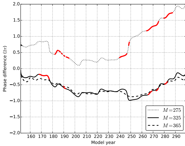
c) Phase difference
