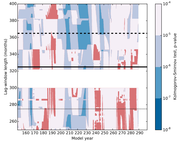
d) KS-test, p-value
