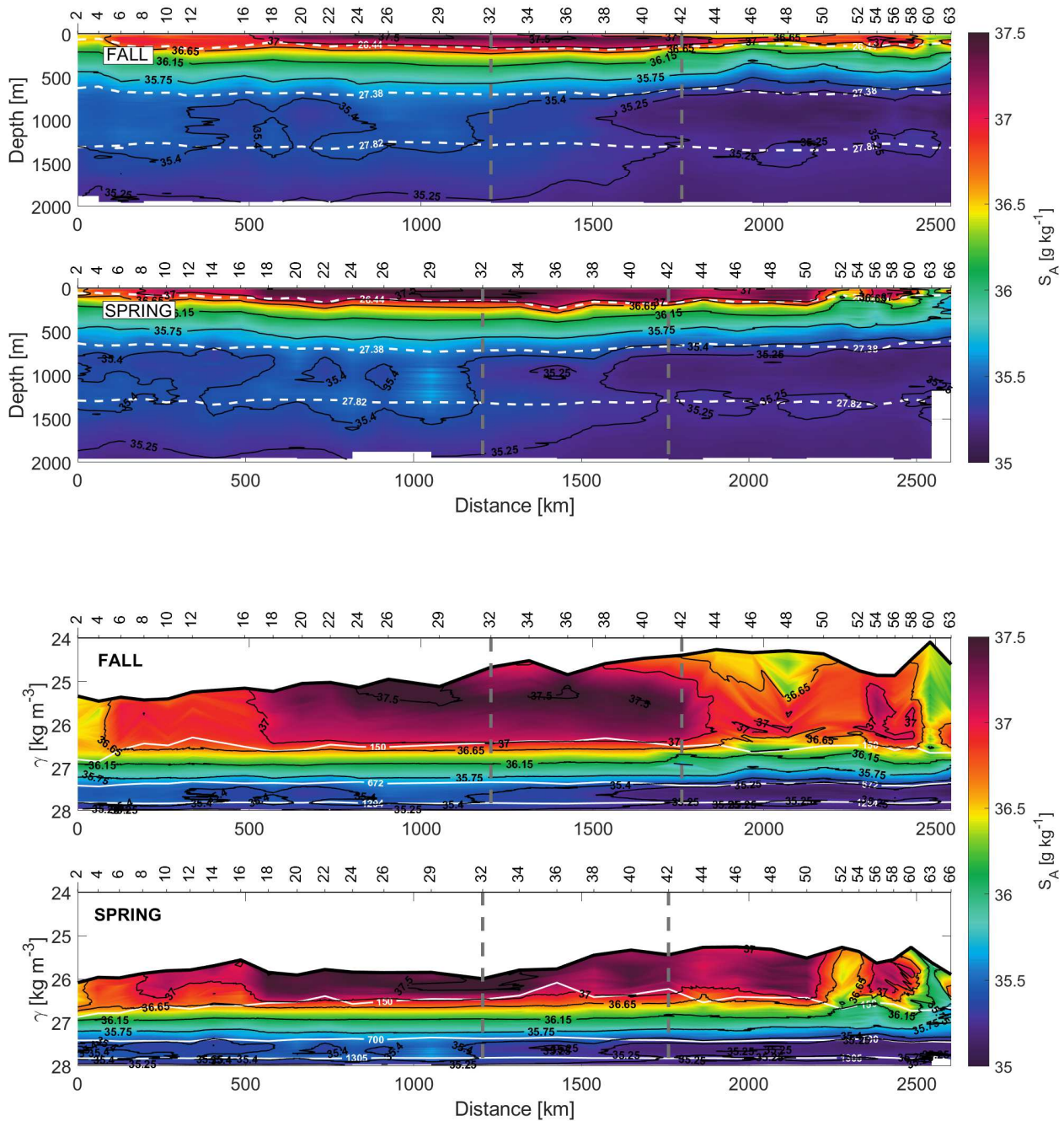
Figure 4. Sections of absolute salinity ( S_A ) with respect to depth (top) and \sigma_n (bottom) during fall and spring. In depth section (top), the isoneutrals which delimit the transports at surface, central, intermediate and deep water are represented by white dashed contours. In \sigma_n section (bottom), the depths of 150, 672/700 and 1204/1294/1305 m are also shown.
