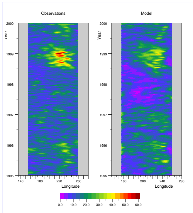
Figure 6. Observed and model sea surface height r.m.s. variance in of the Pacific northward component of ocean surface geostrophic velocity at latitude 6°N between 135°E and 280°E (80°W) model sea surface height fields using Eqns. 1 and 2. The values were calculated from the satellite altimeter and model sea surface height fields using Eqns. 1 and 2. Units are meters \text{cm s}^{-1} .
