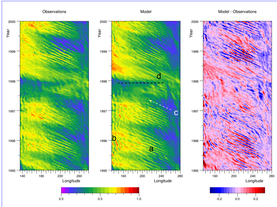
Figure 4. Observed and model sea surface height and their difference in the Pacific at latitude of 6°N between 135°E and 280°E (80°W). Showing (a) westward propagating tropical instability waves or eddies, (b) quasi-steady meanders near the start of the NECC, (c) westward propagating annual Rossby wave, (d) eastward propagating Kelvin-wave Transition Event (see text). Units are metres.
