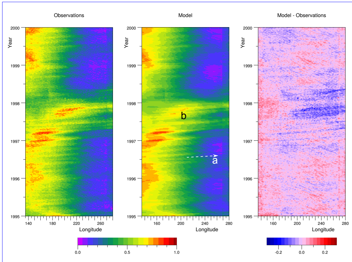
Figure 5. Observed and model sea surface height and their difference in the Pacific on the Equator between 135°E and 280°E (80°W). Showing (a) eastward propagating Kelvin waves, (b) sea level high moving to the central Pacific. Units are metres.
