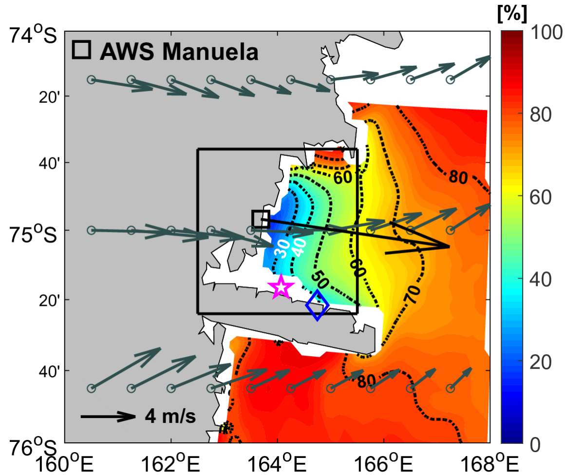
Figure 3: Spatial distributions of averaged sea-ice concentrations from July 2014 to March 2018. The interval of the dotted contour lines is a concentration of 10%. The black square (blue diamond and magenta star) indicates the Automatic Weather System (AWS) Manuela station (DITN and DITD). The dark-gray (black) arrows are mean wind vectors for July 2014–March 2018 using ERA-Interim data (data from AWS Manuela station). The black box denotes an averaged region for sea-ice concentrations.
