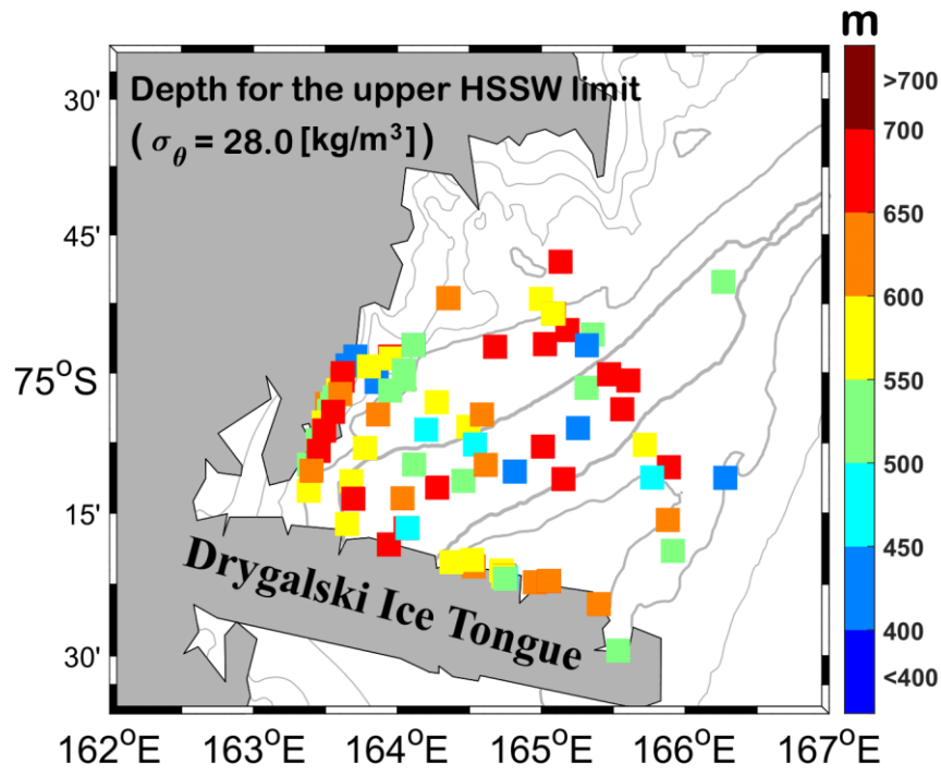
535 Figure 10: Distributions of depth (m) for the upper HSSW limit ( \sigma_\theta = 28 \text{ kg/m}^3 ) in vertical CTD profiles during the four hydrographic surveys (see details in Table 1). The bold gray line indicates the 1,000 m isobaths and the interval between the thinner gray lines is 200 m.
