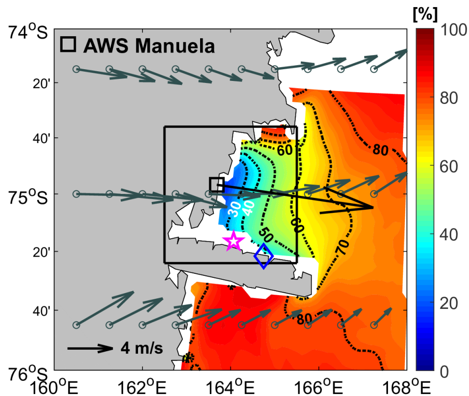
Figure 3: Spatial distributions of averaged sea-ice concentrations from July 2014 to March 2018. The interval of the dotted contour lines is a concentration of 10%. The black square indicates (blue diamond and magenta star) indicates the Automatic Weather System (AWS) Manuela station. The blue diamond and magenta star are for the (DITN and DITD). The dark-gray and (black) arrows are mean wind vectors for July 2014–March 2018 using ERA-Interim data and (data from AWS Manuela station, respectively). The black box denotes the averaged region over which the for sea-ice concentrations are averaged in Fig. 9.
