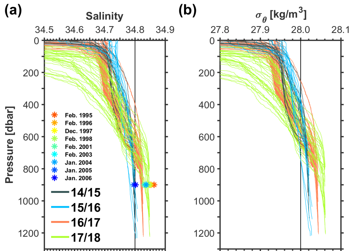
530 Figure 7: (a) Vertical salinity profiles at each observation period. The black solid line indicates 34.8. The asterisks indicate salinity at ~ 900 m depth in TNB observed during 1995–2006 from Fusco et al. (2009) (b) The same as Fig. 7a, but for potential density ( \sigma_\theta ), where the black solid line indicates 28.0 kg m -3
