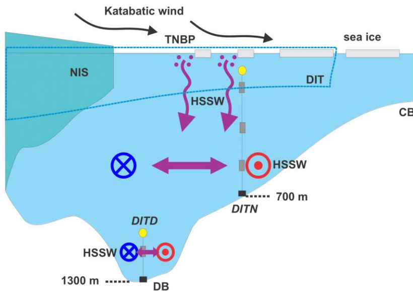
Figure 14: A schematic of the spatio-temporal variations in the production of HSSW in TNBP. The downward arrows show HSSW formation through convection from brine rejection (dots) during sea ice formation atled by a supply of brine from the surface in the polynya opened by off-shelf, which is related to polynya development via winds. The brine rejecting process associated with sea ice formation, which is driven by katabatic winds, is denoted with dots near the surface. The horizontal bi-directional arrows indicate that the HSSW that formed near the Nansen Ice Shelf (NIS) advects at the deepest depths of both the eastern Terra Nova Bay (DITN) and Drygalski Basin (DITD) via cyclonic pattern flows in TNBP. The blue and red circle represents flow into and out of the page (outgoing (incoming) flow). DB, CB and DIT denote the Drygalski Basin, Crary Bank and Drygalski Ice Tongue, respectively.
