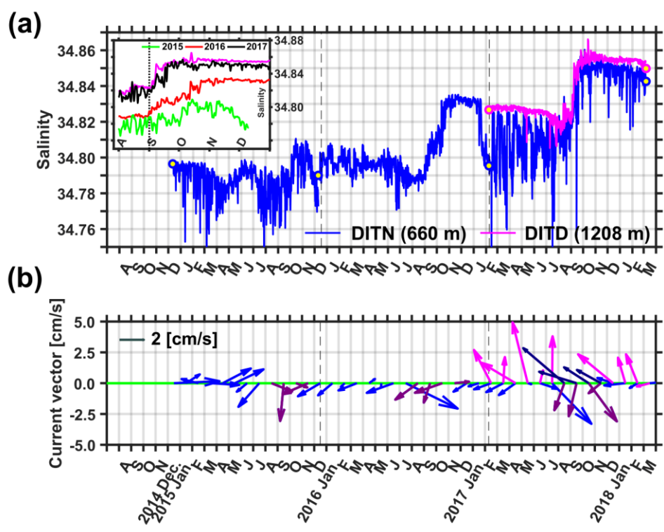
Figure 4: (a) Time-series of the near-bed salinity observed in the DITN (blue) and DITD (magenta) from December 2014 to March 2018. The blue (magenta) circles filled with yellow indicate the averaged salinity in a 5-m layer at the bottom obtained using CTD data observed near the DITN (DITD). The black dashed line divides periods of each leg in the moorings (see details in Table. 1). A zoomed-in plot for the one-day moving average near-bed salinity time-series from August to December of each year is shown in the small upper-left inset. The magenta time-series in the inset is also for the DITD. (b) Monthly mean current vectors at 660 m in the DITN and 1222 m in the DITD are indicated by blue and magenta arrows. Mean current vectors from August to November in the DITN and DITD are emphasized using denoted by purple and navy arrows, respectively.
