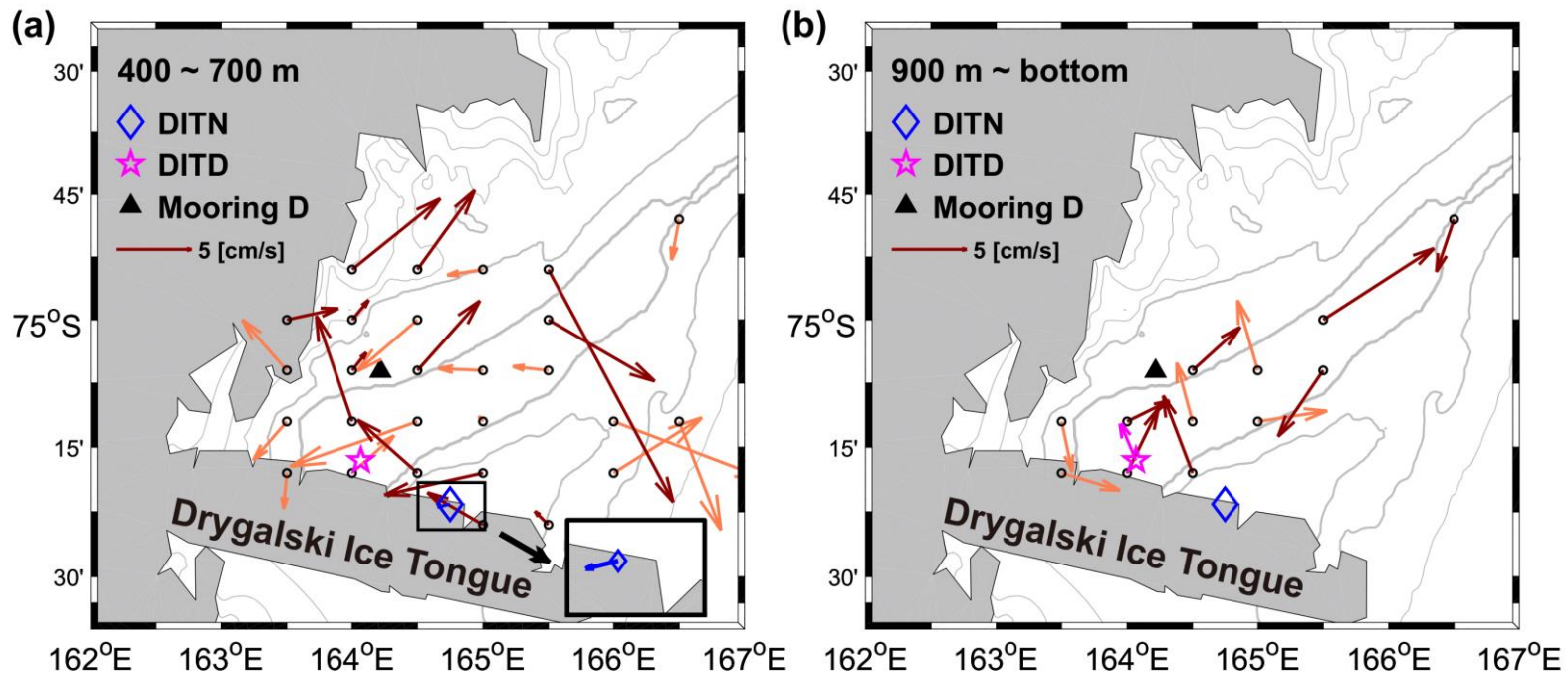
550 Figure 12: (a) Mean currents in a range of 400–700 m during four hydrographic surveys (see details in Table 1). The LADCP data are arranged by averaging the data on a 0.5^\circ \times 0.1^\circ grid. The averaged current vector from January to February at 660 m in the DITN is denoted by a blue arrow. The inset shows the current vectors of the DITN. The current vectors mainly discussed in Section 4.2 are highlighted by a dark red. The bold grey line indicates the 1,000 m isobaths and the interval between the thinner gray lines is 200 m. A scale arrow is denoted in the left part of the figure. (b) The same as Fig. 12a, but for the range of 900 m–bottom. A magenta arrow shows the averaged current vector from January to February at 1,222 m in the DITD.
