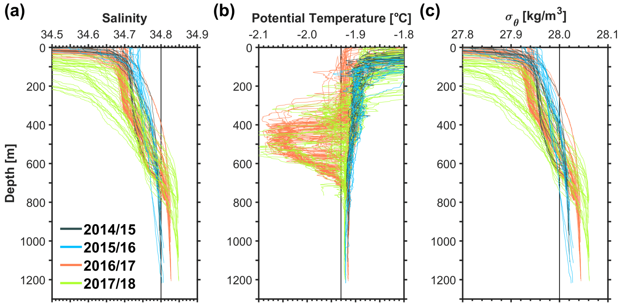
Figure 7: (a) Vertical salinity profiles at each observation period. The black solid line indicates 34.8 (b) The same as Fig. 7a, but for potential temperature, whereas the black green solid line denotes -1.935 °C. (c) The same as Fig. 7a, but for potential density ( \sigma_\theta ), whereas the black solid line indicate means 28.0 kg m -3
