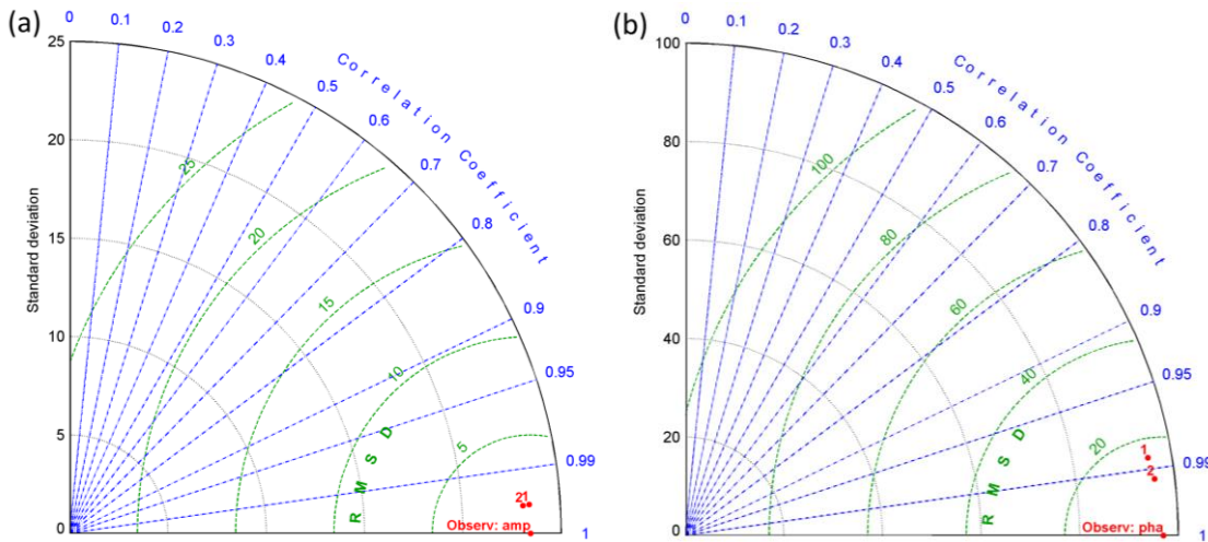
Figure B1. Taylor diagrams based on observed and modelled data at 3 gauging stations, '1' and '2' indicate simulation results on curvilinear and unstructured grids respectively: a) for amplitude; b) for phase.
