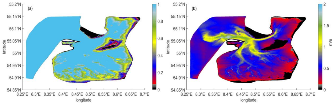
1225 Figure 3. a) The probability of wetting based on simulations of the two full tidal cycles using the unstructured grid. b) The peak tidal velocities at the current position using the unstructured grid.
