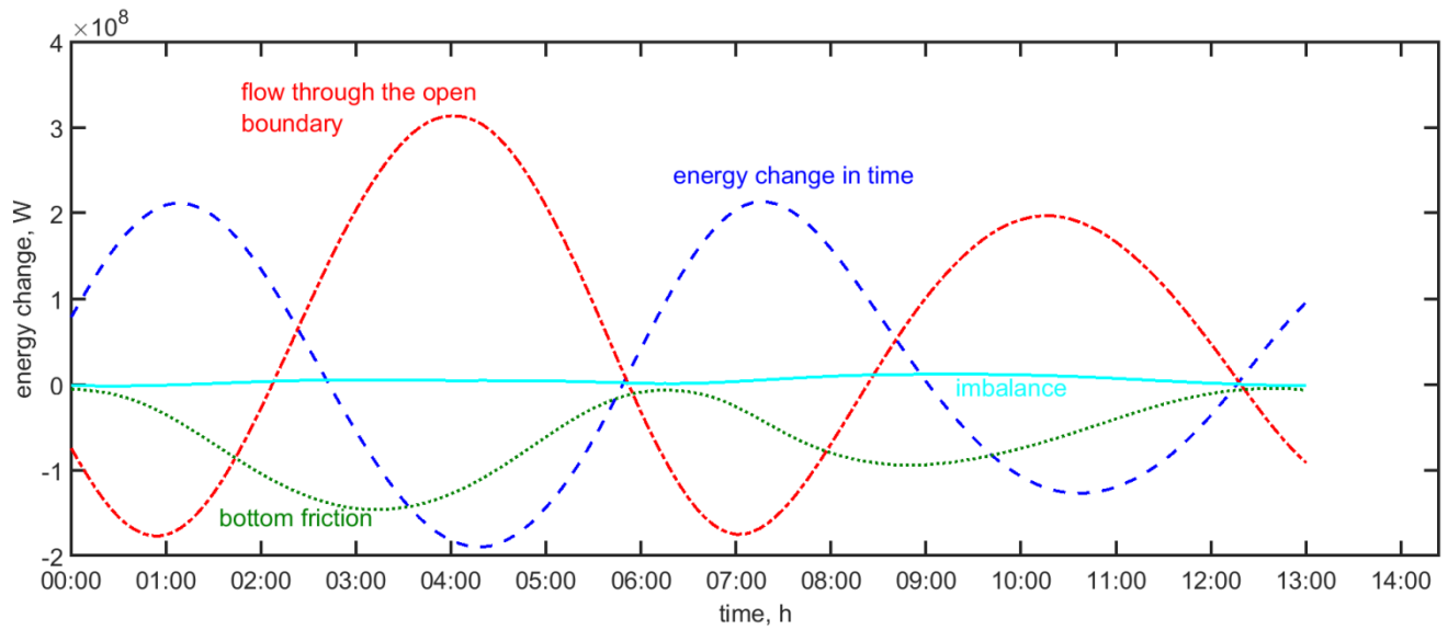
Figure 4. The energy budget for the depth-averaged solution with open boundary conditions from the TPXO 9 database for summary tide, [W], in blue (dashed line): energy change in time, in red (dash-dotted line): flow through the open boundaries, in green (dotted line): bottom friction, in cyan (solid line): imbalance.
