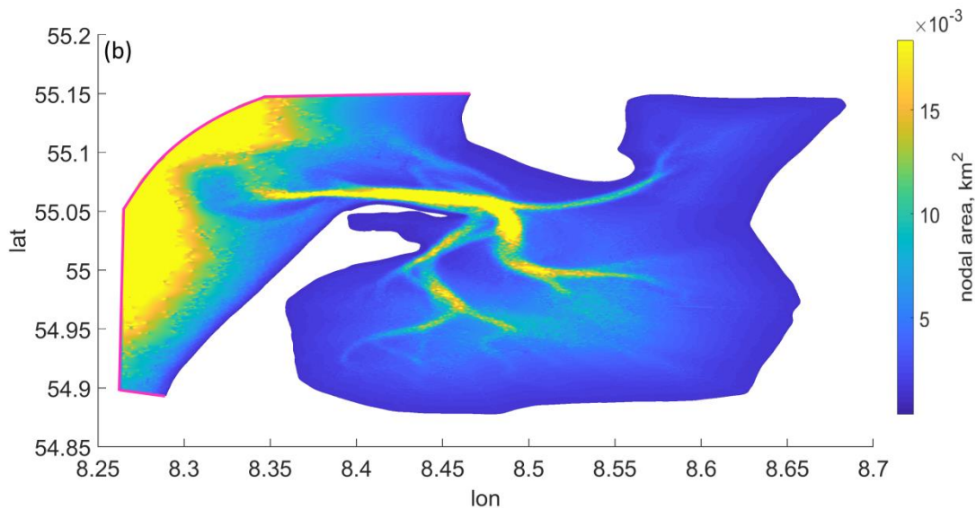
Figure A1. Nodal area, pink color indicates position of the open boundary: a) curvilinear grid; b) unstructured grid.
