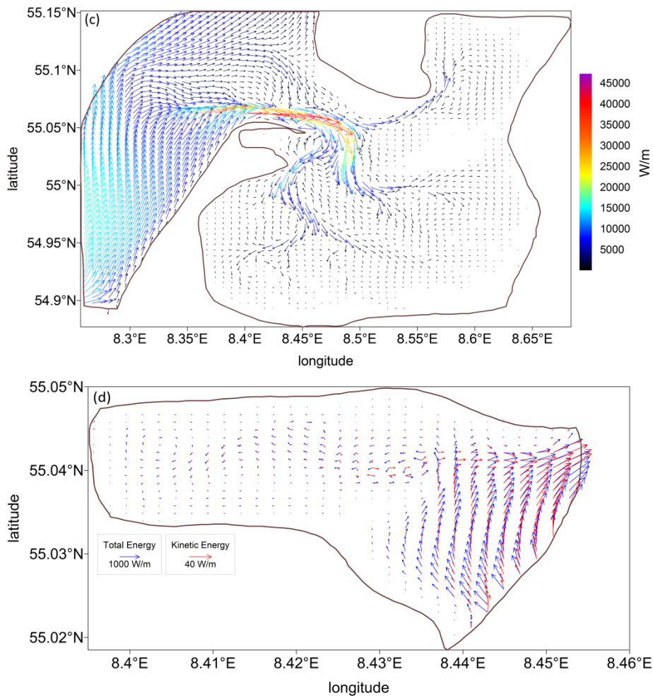
1240 Figure 5. The flux of tidal energy (summary tide): a) kinetic; b) potential; c) total ( \mathbf{E}_\lambda, \mathbf{E}_\theta ); d) the total (blue arrows) and kinetic (red arrows) energy fluxes for the Königshafen subarea. The potential energy fluxes behavior is visually identical to the total energy fluxes one.
