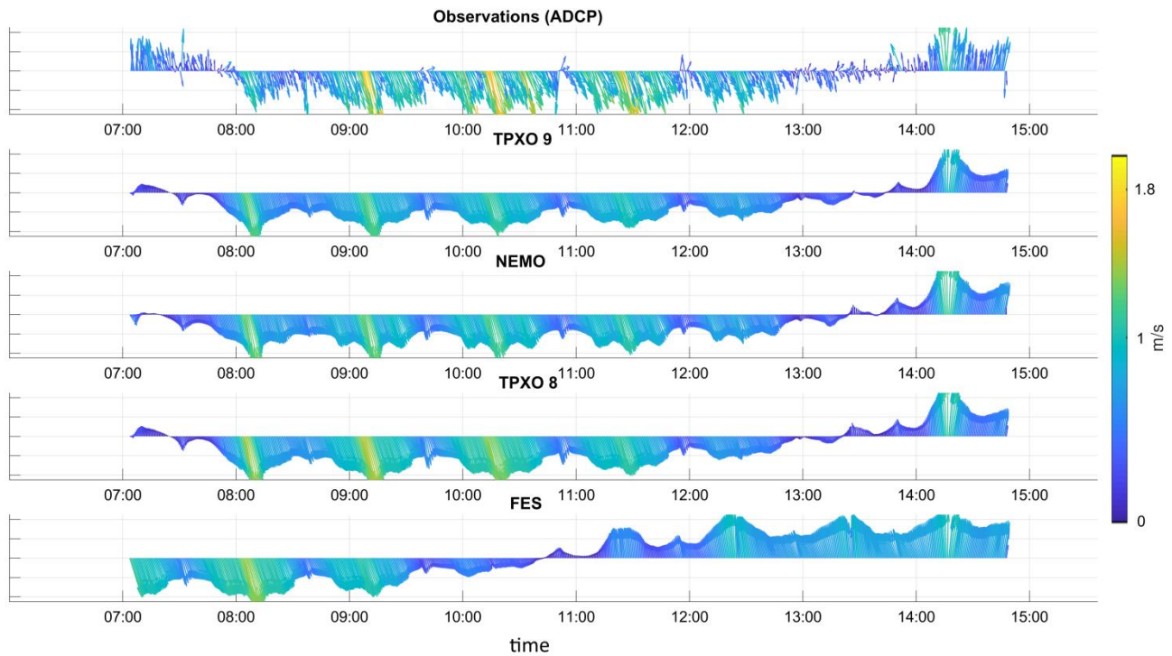
1220 Figure 2. The observed and modelled depth-averaged velocities on May 29, 2018. The arrow color indicates the current magnitude [m/s]; arrow directions indicate the current direction.
