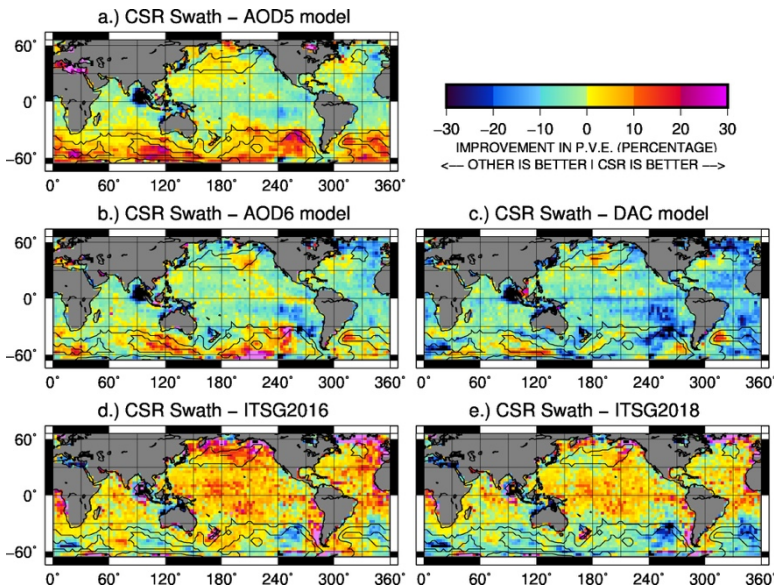
Figure 4: Differences in sub-monthly P.V.E for CSR swath vs. another data type: (a) AOD5 de-aliasing ocean model, (b) AOD6 de-aliasing ocean model, (c) altimetry's DAC de-aliasing ocean model, (d) ITSG2016 GRACE data, and (e) ITSG2018 GRACE data. Values are relative to CSR swath P.V.E.s, so positive numbers (red) denote that CSR swath matches altimetry better, while negative numbers (blue) denote that the other series matches altimetry better.
