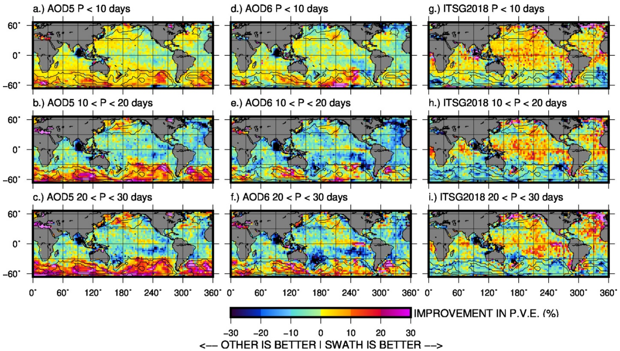
545 Figure 7: Differences in P.V.E for CSR swath vs. another data type, per frequency band: (a, b, c) AOD5 de-aliasing ocean model, (d, e, f) AOD6 de-aliasing ocean model, and (g, h, i) ITSG2018 GRACE data. The top row gives the highest sub-monthly frequency band, while the bottom gives the lowest sub-monthly frequency band. Values are relative to CSR swath P.V.E.s, so positive numbers (red) denote that CSR swath matchest altimetry better, while negative numbers (blue) denote that the other series matches altimetry better.
