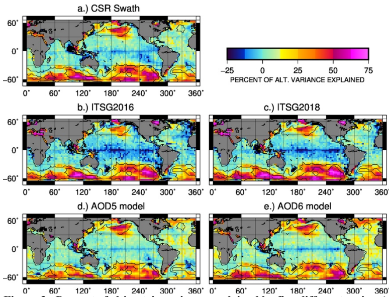
Figure 3: Percent of altimetry variance explained by five different series: (a) CSR swath GRACE data, (b) ITSG2016 GRACE data, (c) ITSG2018 GRACE data, (d) AOD5 ocean de-aliasing model, and (e) AOD6 ocean de-aliasing model.
