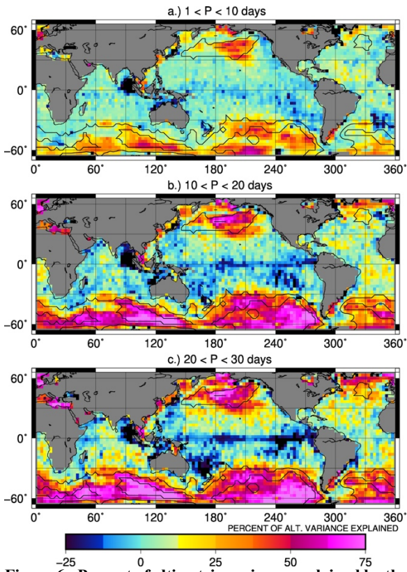
540 Figure 6: Percent of altimetric variance explained by the CSR swath series at three sub-monthly frequency bands: (a) periods below 10 days, (b) periods between 10-20 days, (c) periods between 20-30 days.
