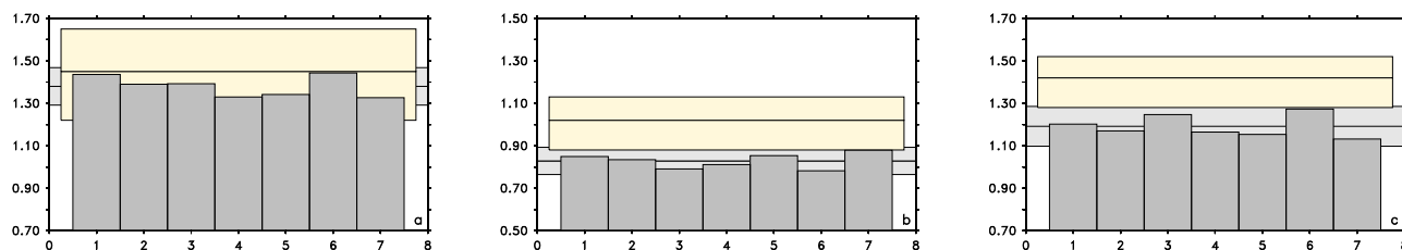
Figure 3. Extreme sea levels from RCA4-NEMO ERA40 with 100-year return period for three stations: Furuögrund (a), Stockholm (b), Smögen (c). The different analysis periods are 1961 to 2005 (1), 1970 to 2009 (2), 1961 to 1989 (3), 1970 to 1999 (4), 1980 to 2009 (5), 1961 to 1984 (6) and 1985 to 2009 (7). The horizontal line represents the mean of the different estimates and the lightly shaded area around it is the 95% confidence interval.
