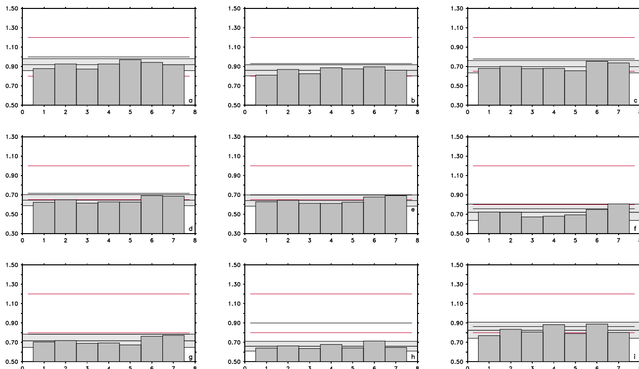
Figure 8. Mean 99.9 percentile of ESLs for nine stations along the Swedish coast: Furuögrund (a), Ratan (b), Spikarna (c), Stockholm (d), Landsort (e), Kungsholmsfort (f), Klagshamn (g), Goteborg (h), Smögen (i). The different realizations have been estimated from RCA4-NEMO ERA40 (1), RCA4-NEMO ensemble mean HISTORICAL (2), RCA4-NEMO MPI-ESM-LR HISTORICAL (3), RCA4-NEMO EC-EARTH HISTORICAL (4), RCA4-NEMO GFDL-ESM2M HISTORICAL (5), RCA4-NEMO HadGEM2-ES HISTORICAL (6), RCA4-NEMO IPSL-CM5A-MR HISTORICAL (7). The horizontal lines and shaded areas are as in Fig. 2. The red lines represent SMHI’s warning level 1 and warning level 2, respectively. The horizontal black line is the 99.9 percentile of the observations. All estimates are based on the common historical period 1970 to 1999.
