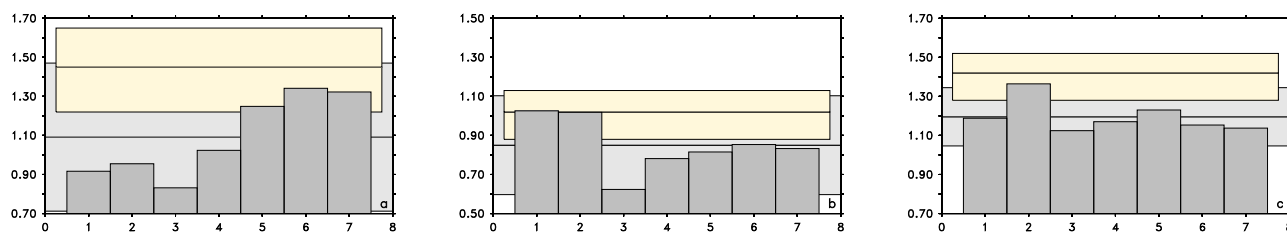
Figure 4. Extreme sea levels as in Fig. 3. The different sensitivity runs are NEMO-Nordic ERA40 (1), NEMO-Nordic ERA-interim (2), NEMO-Nordic interpolated (3), NEMO-Nordic 3.6 ERA40 (4), NEMO-Nordic 3.6 EURO4M (5), RCA4-NEMO ERA40 (6), RCA4-NEMO-1hr ERA40 (7). Table 3 gives an overview of the experiments. The common analysis period was 1980 to 2009, except for NEMO-Nordic 3.6 ERA40 it was 1980 to 2005.
