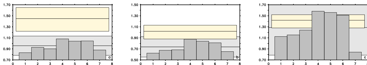
Figure 5. Extreme sea levels as in Fig. 3. The different bars refer to the experiments NEMO-Nordic interpolated (1), NEMO-Nordic ORAS4 (2), NEMO-Nordic ORAS4 b (3), NEMO-Nordic ORAS4 c (4), NEMO-Nordic Surge (5), NEMO-Nordic Surge b (6), NEMO-Nordic NOT (7). The different experiments are listed in Table 4. The common analysis period was 1980 to 2009.
