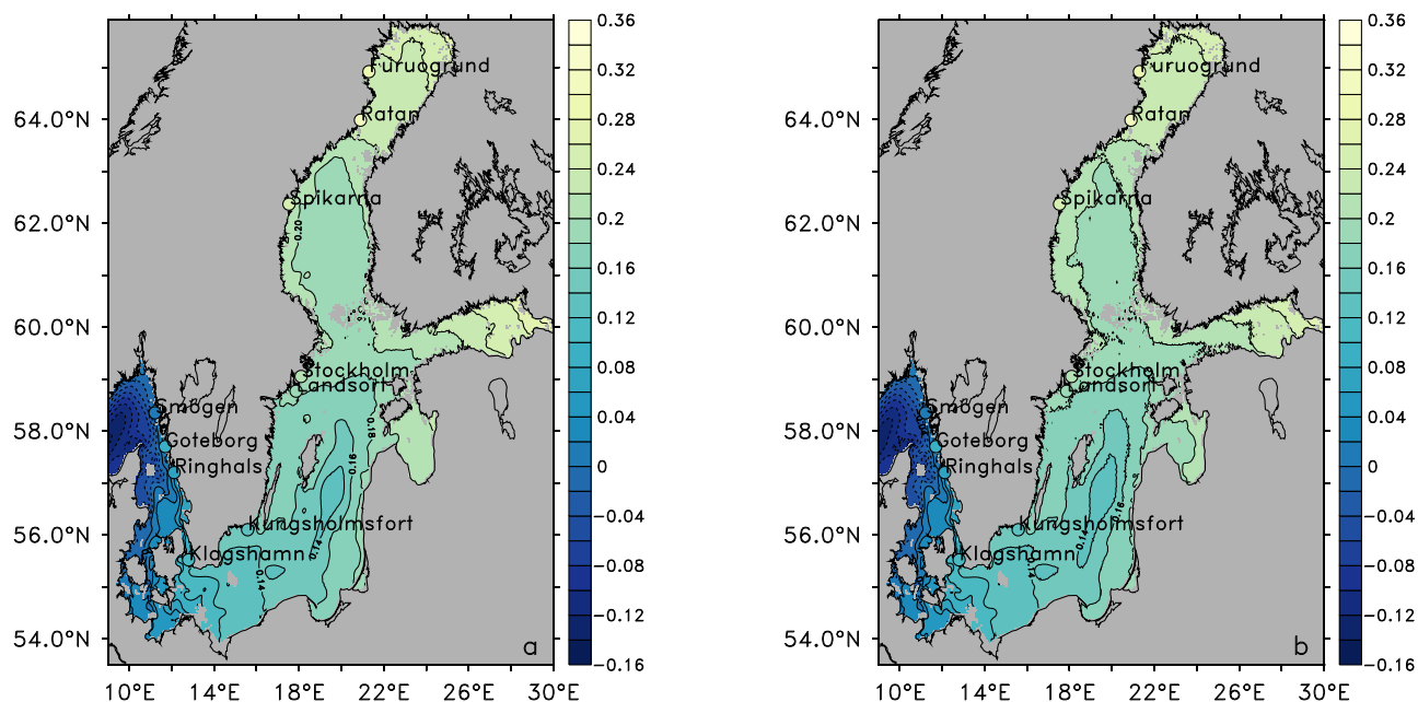
Figure 1. Mean sea level [cm] for the period 1970 to 1999 for the hindcast RCA4-NEMO ERA40 (a) and the ensemble mean (b). The colored dots indicate MSL estimated from long-term observations (WISKI, 2017).
