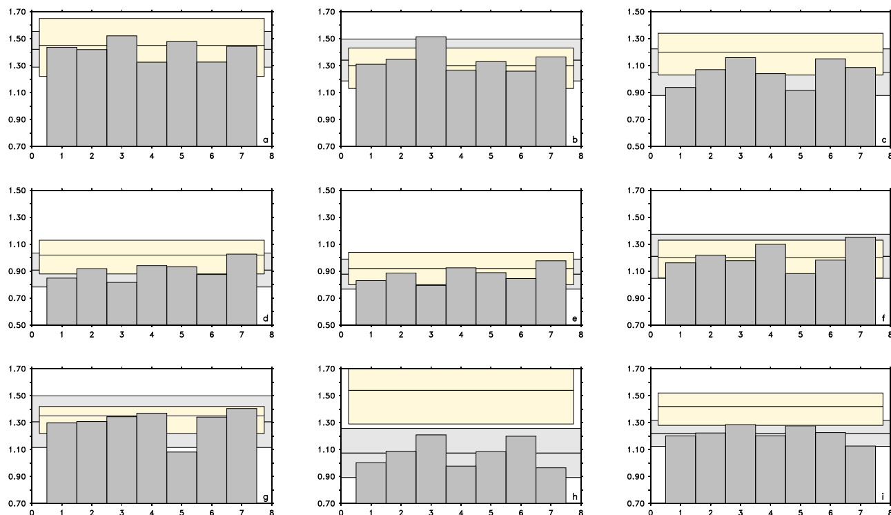
Figure 7. Extreme sea levels with 100-year return period for nine stations along the Swedish coast: Furuögrund (a), Ratan (b), Spikarna (c), Stockholm (d), Landsort (e), Kungsholmsfort (f), Klagshamn (g), Goteborg (h), Smögen (i). The different realizations have been estimated from RCA4-NEMO ERA40 (1), RCA4-NEMO ensemble mean HISTORICAL (2), RCA4-NEMO MPI-ESM-LR HISTORICAL (3), RCA4-NEMO EC-EARTH HISTORICAL (4), RCA4-NEMO GFDL-ESM2M HISTORICAL (5), RCA4-NEMO HadGEM2-ES HISTORICAL (6), RCA4-NEMO IPSL-CM5A-MR HISTORICAL (7) (cf. Table 1). The horizontal lines and shaded areas are as in Fig. 2. All model estimates are based on the common historical period 1961 to 2005.
