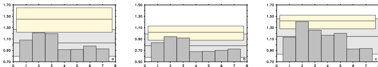
Figure 6. Extreme sea levels as in Fig. 3. The different sensitivity runs are NEMO-Nordic viscous (1), NEMO-Nordic no-slip (2), NEMO-Nordic free-slip (3), NEMO-Nordic interpolated (4), NEMO-Nordic MSL (5), NEMO-Nordic E-HYPE (6), NEMO-Nordic discharge (7). Table 5 gives an overview of the experiments. The common analysis period was 1961 to 2005.
