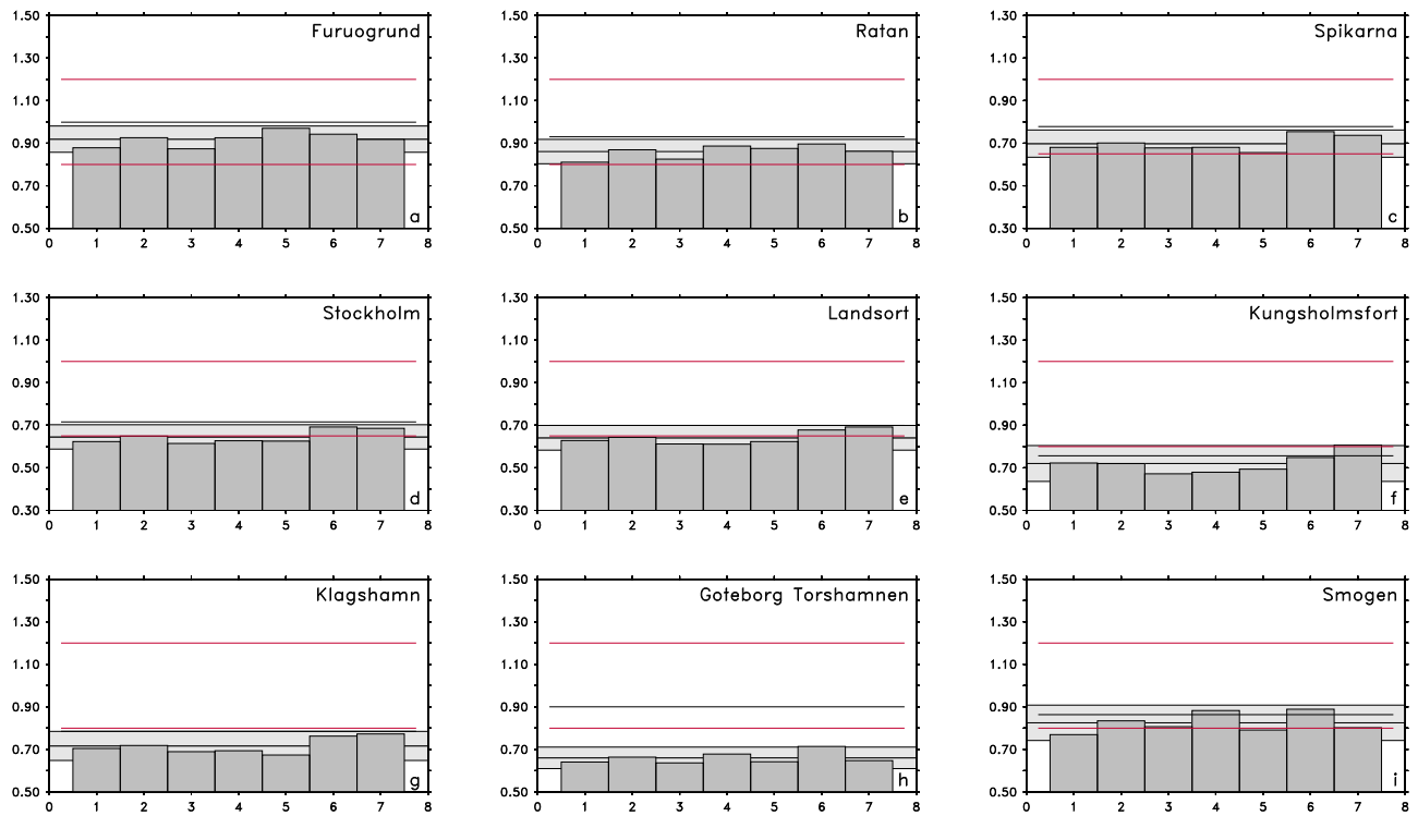
Figure 5. Mean 99.9 percentile of ESLs [m] for the same stations and the same realizations as in Fig. 4. The red lines represent SMHI's warning level 1 and warning level 2, respectively. The black line is the 99.9 percentile of the observations. All estimates are based on the common historical period 1970 to 1999.
