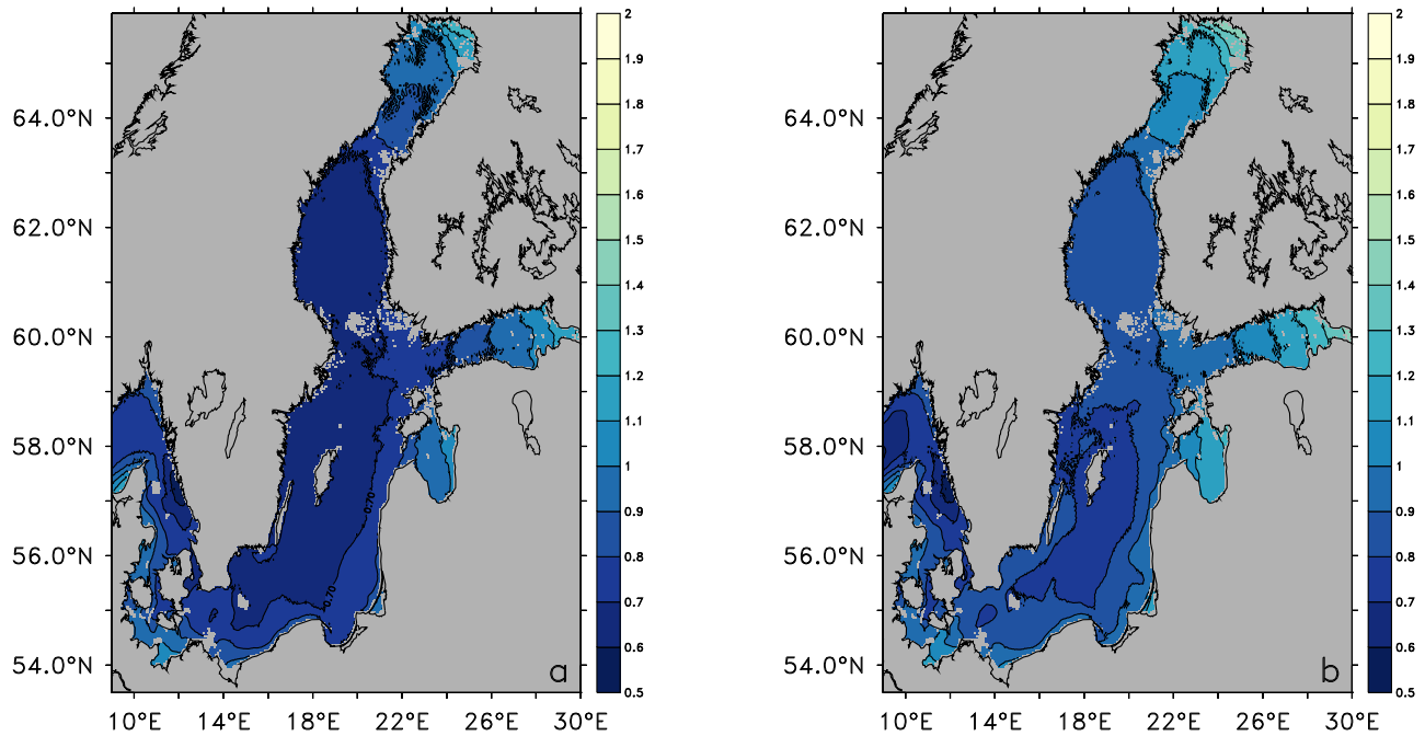
Figure 6. Ensemble median of the 99.9 percentile of ESLs [m] for the period 1970 to 1999 relative to the mean sea surface (a) and relative to bedrock (b).
