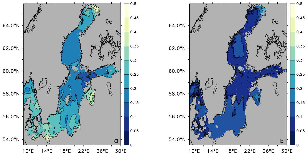
Figure 7. Uncertainty of ESL [m] for the period 1970 to 1999 for the RCM ensemble (a) and the GCM ensemble (b). The uncertainty is defined here as the likely range (5% to 95% range of ensemble solutions).
