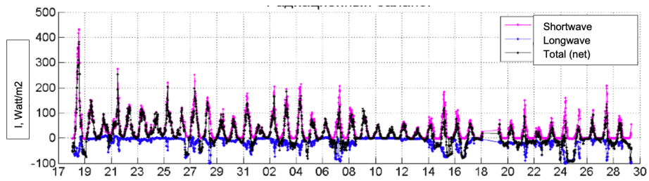
Fig. 4. Radiative balance components (Watt/m 2 ) measured from RV Akademik Tryoshnikov during ARKTIKA-2018 expedition: magenta - shortwave radiation; blue, longwave radiation; black, total (done by A.Pashkov)
