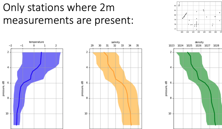
Fig. 2. The upper 10 meters of T, S, density from vertical CTD profiles
