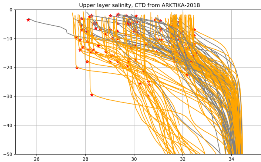
Fig. 3. Vertical profiles of practical salinity (b) from CTD measurements in the upper 50 meters. Red stars indicate the mixed layer depth, calculated using de Boyer Montégut et al. (2004) method
