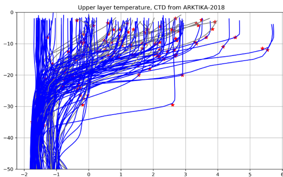
Fig. 2. Vertical profiles of conservative temperature from CTD measurements in the upper 50 meters. Red stars indicate the mixed layer depth, calculated using de Boyer Montégut et al. (2004) method
