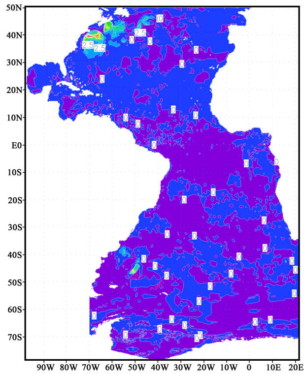
Fig. 1. Figure 5. SST for all assimilation methods. (a) control, (b) EnOI, (c) GKF, (d) EnOI minus GKF.
